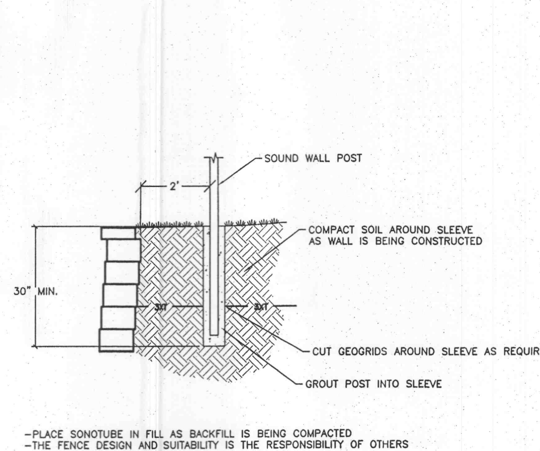
SOUND WALL POST DETAIL NOT TO SCALE
