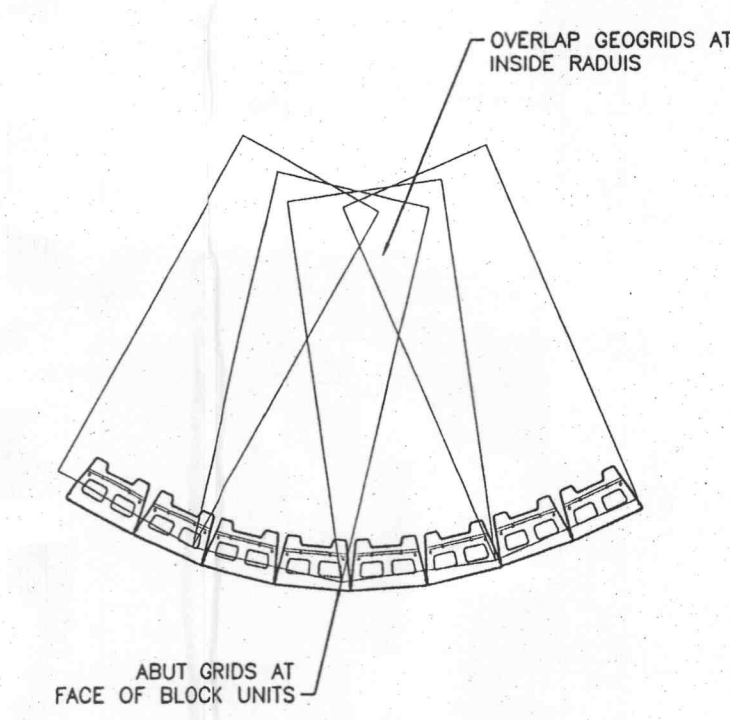
RADIUS DETAIL NOT TO SCALE
