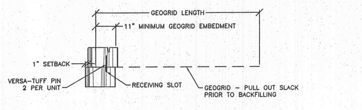
CONNECTION DETAIL NOT TO SCALE
