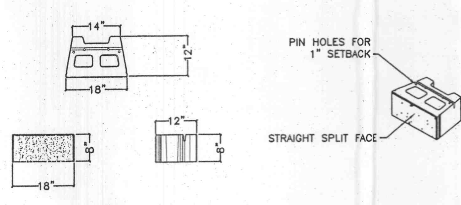
VERSA-LOK SQUARE FOOT UNIT NOT TO SCALE
