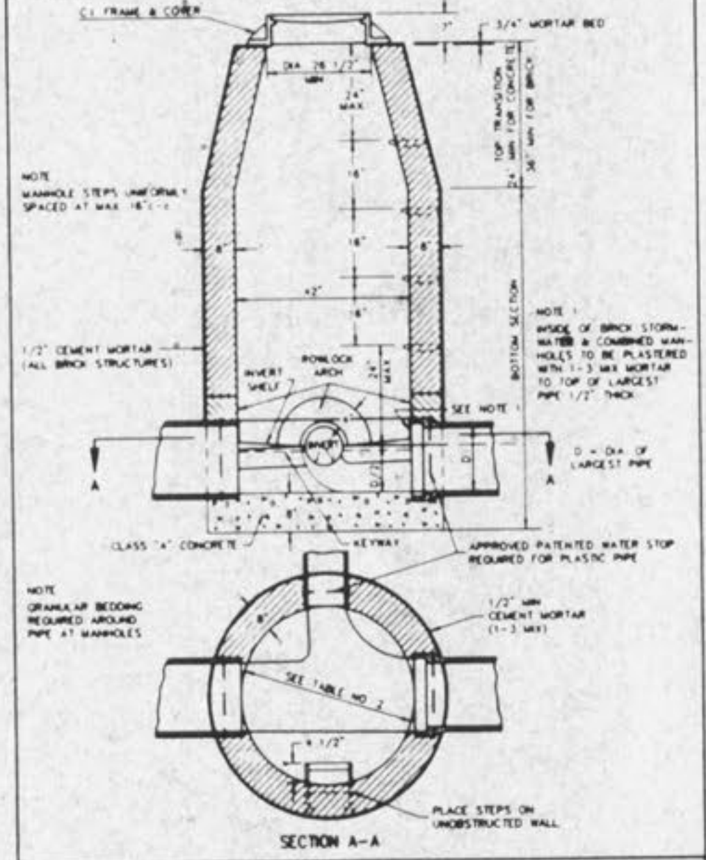
LINE MANHOLE ON PIPE SEWERS 8"-24" DIA. METROPOLITAN ST. LOUIS SEWER DISTRICT Standard Details of Sewer Construction Dr. W.S.H. Ch. J.C.K. 1992 SHEET 8
