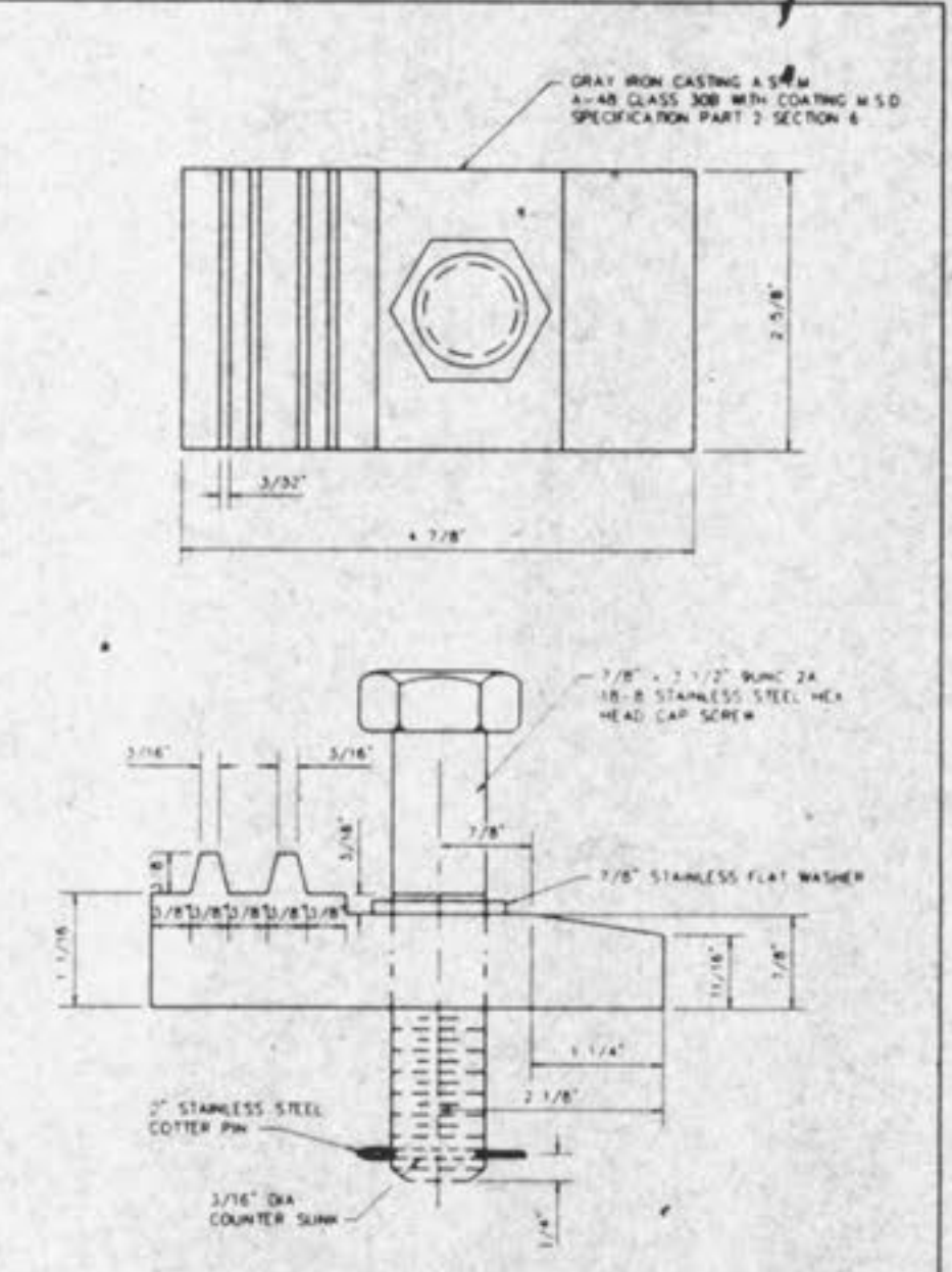
LOCKING DEVICE FOR TYPE "T" LOCK TYPE MANHOLE COVER METROPOLITAN ST. LOUIS SEWER DISTRICT Standard Details of Sewer Construction Dr. R.G.W. Ch. J.C.K. 1992 SHEET 51
