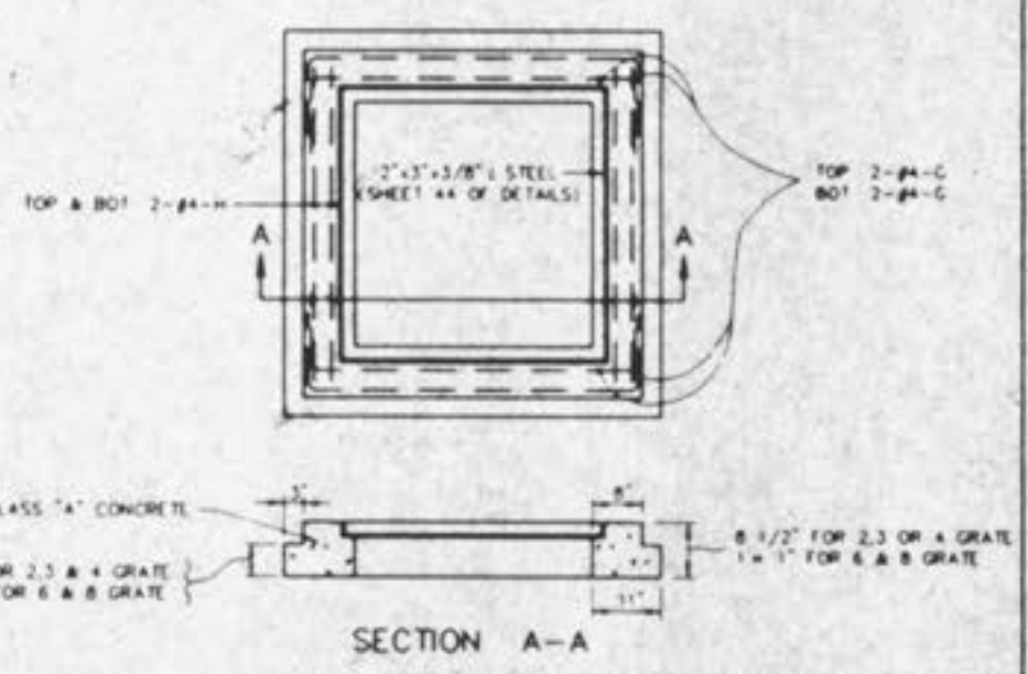
STEEL REQUIREMENTS FOR GRATE INLET SEAT METROPOLITAN ST. LOUIS SEWER DISTRICT Standard Details of Sewer Construction Dr. W.S.H. Ch. J.C.K. 1992 SHEET 46
