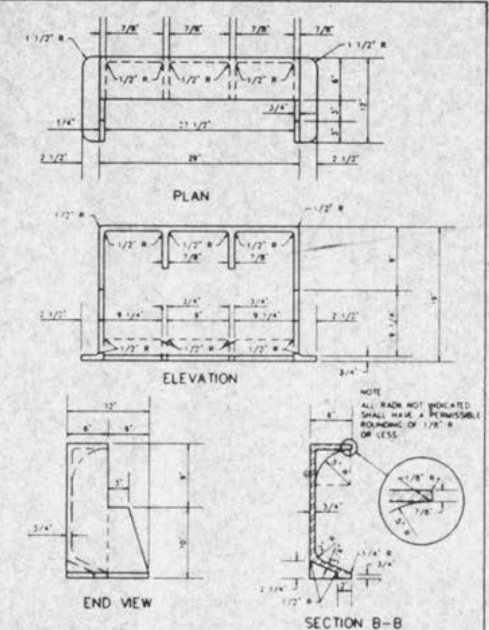
CAST IRON SIDE INTAKE UNIT FOR GRATED INLETS METROPOLITAN ST. LOUIS SEWER DISTRICT Standard Details of Sewer Construction Dr. R.G.W. Ch. J.C.K. 1992 SHEET 47
