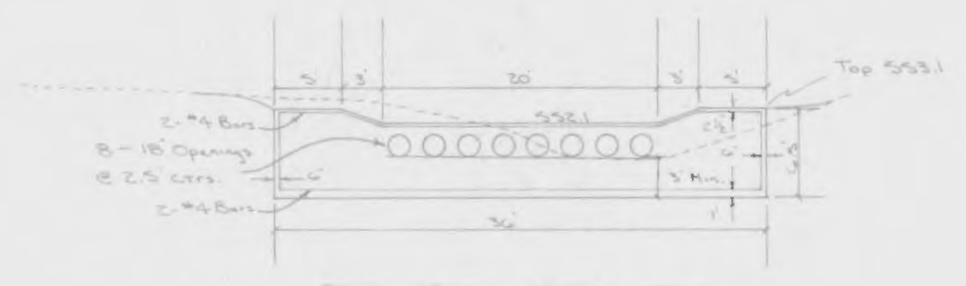
WEIR DETAIL
