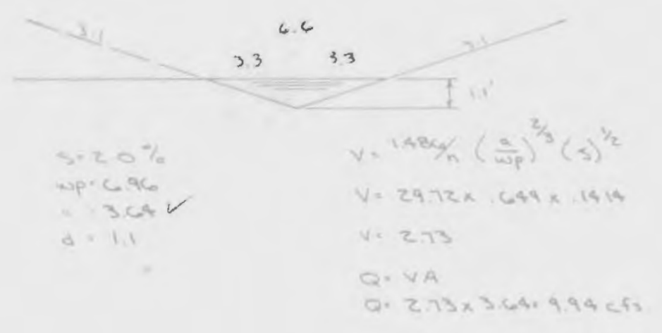
SWALE DETAIL (Scale to A1 14)
