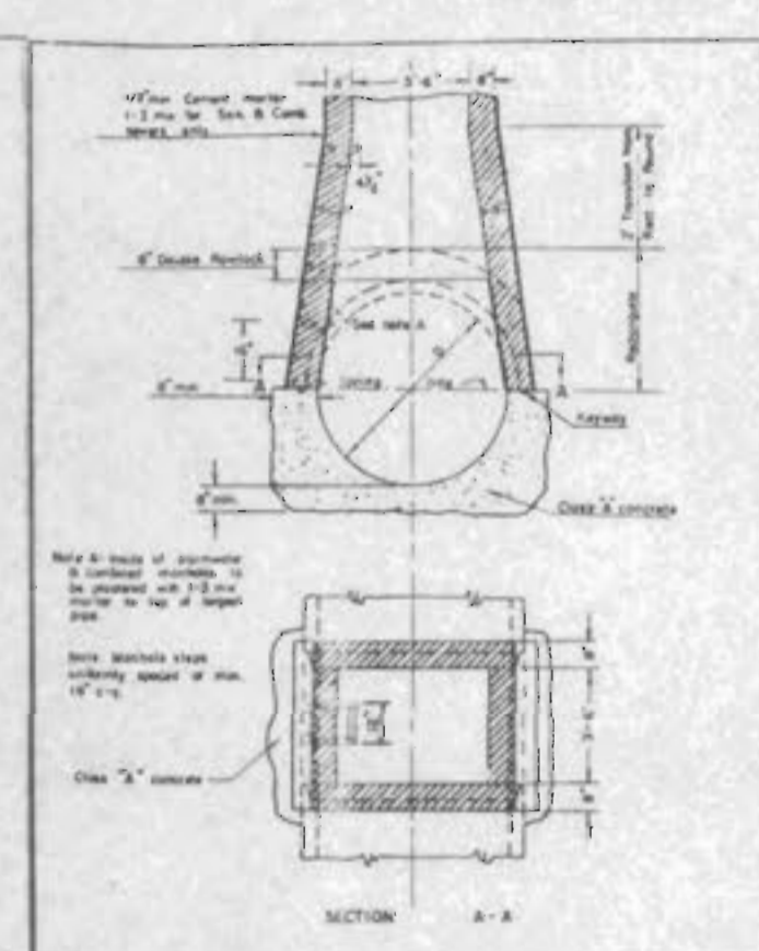
METROPOLITAN ST. LOUIS SEWER DISTRICT Standard Details of Sewer Construction D. S. J. April 1978 Sheet 11
