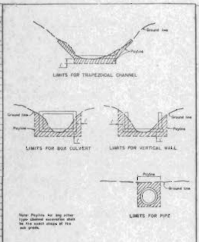
METROPOLITAN ST. LOUIS SEWER DISTRICT Standard Details of Sewer Construction D. S. J. April 1978 Sheet 1
