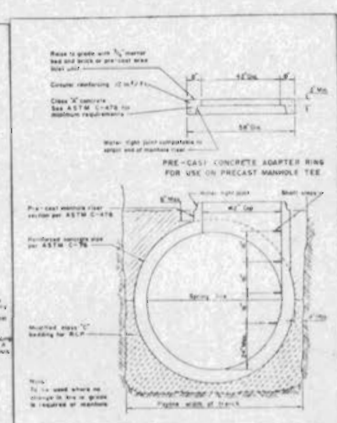
METROPOLITAN ST. LOUIS SEWER DISTRICT Standard Details of Sewer Construction D. S. J. April 1978 Sheet 14
