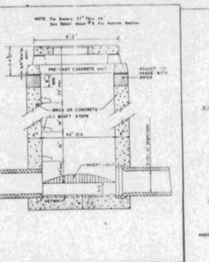
METROPOLITAN ST. LOUIS SEWER DISTRICT Standard Details of Sewer Construction D. S. J. April 1978 Sheet 15
