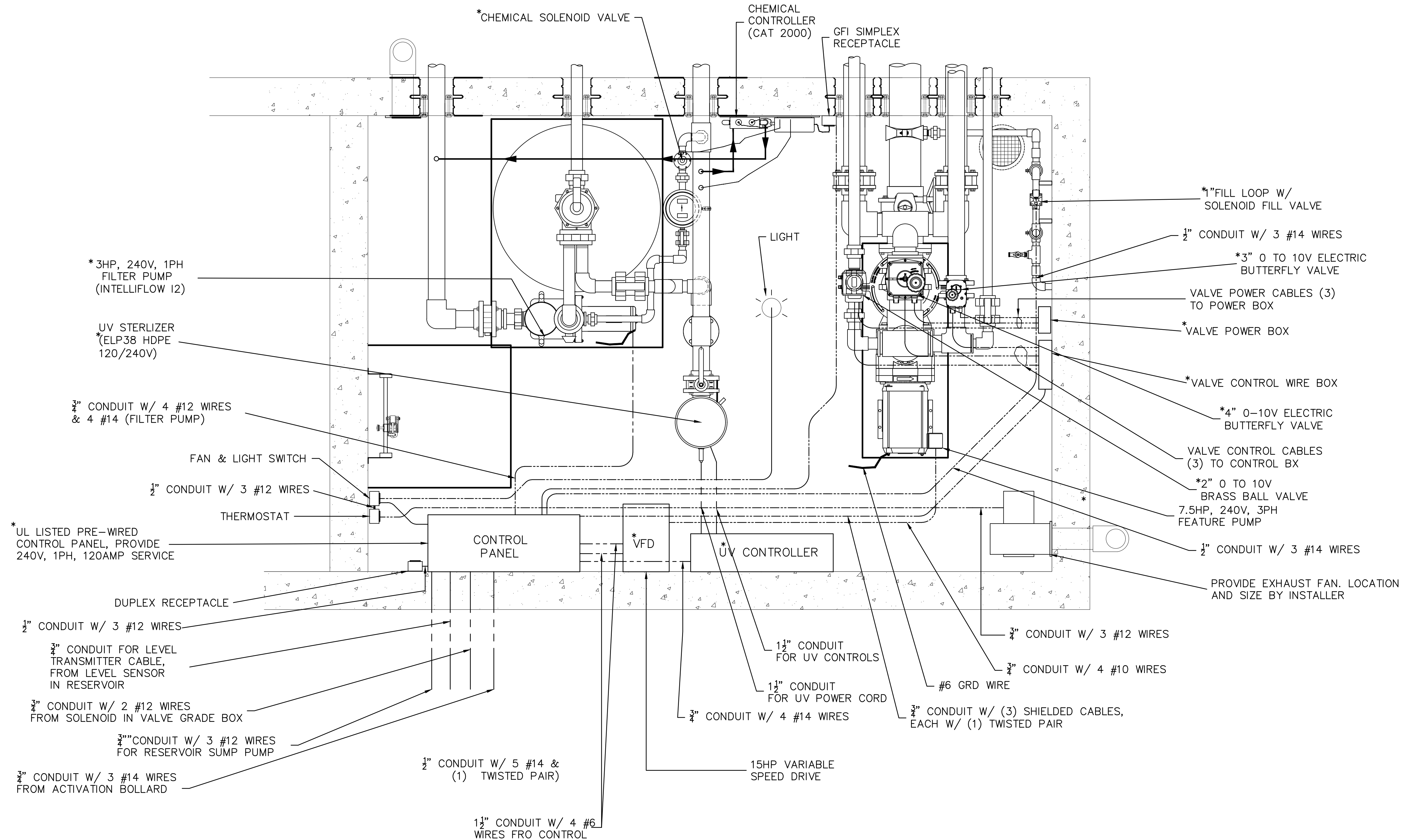
EQUIPMENT ROOM ELECTRICAL PLAN SCALE: 1" = 1'
