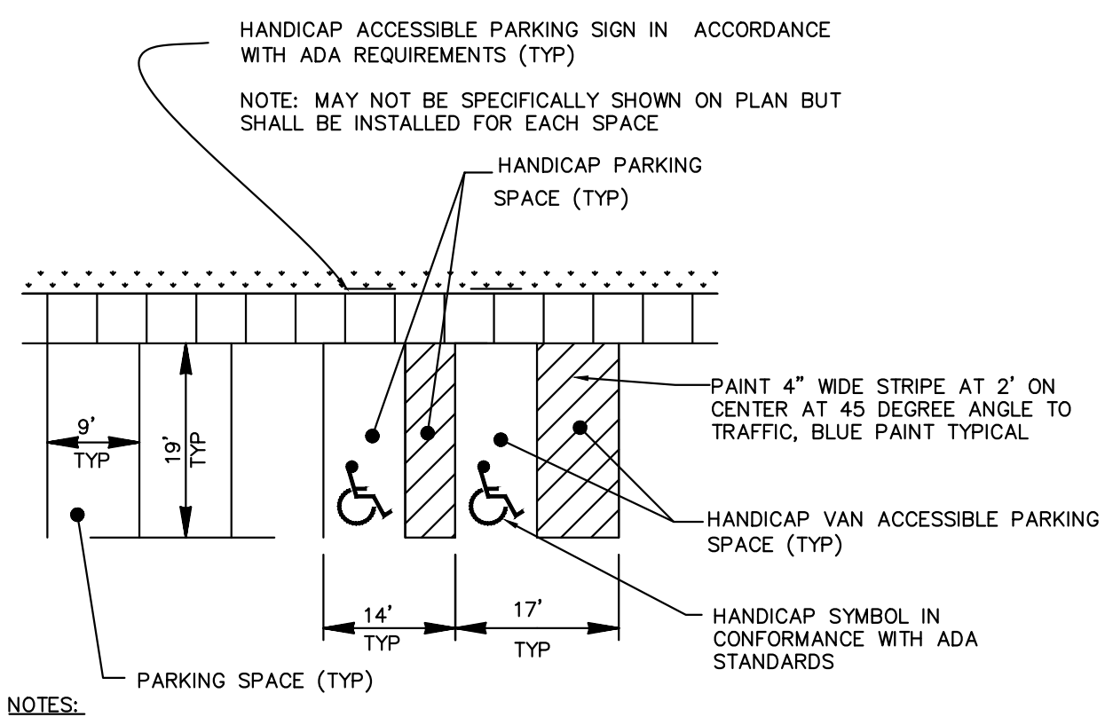
TYPICAL PARKING STRIPING N.T.S.
