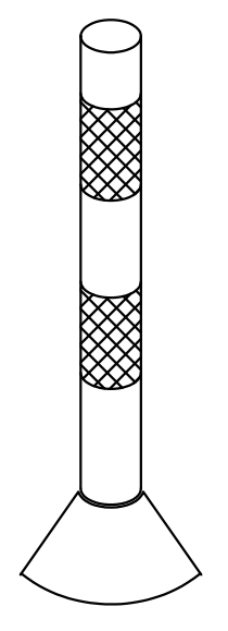
18" REFLECTORIZED FLEXIBLE DELINEATOR POST (R.F.D.P.) DETAIL NOT TO SCALE
