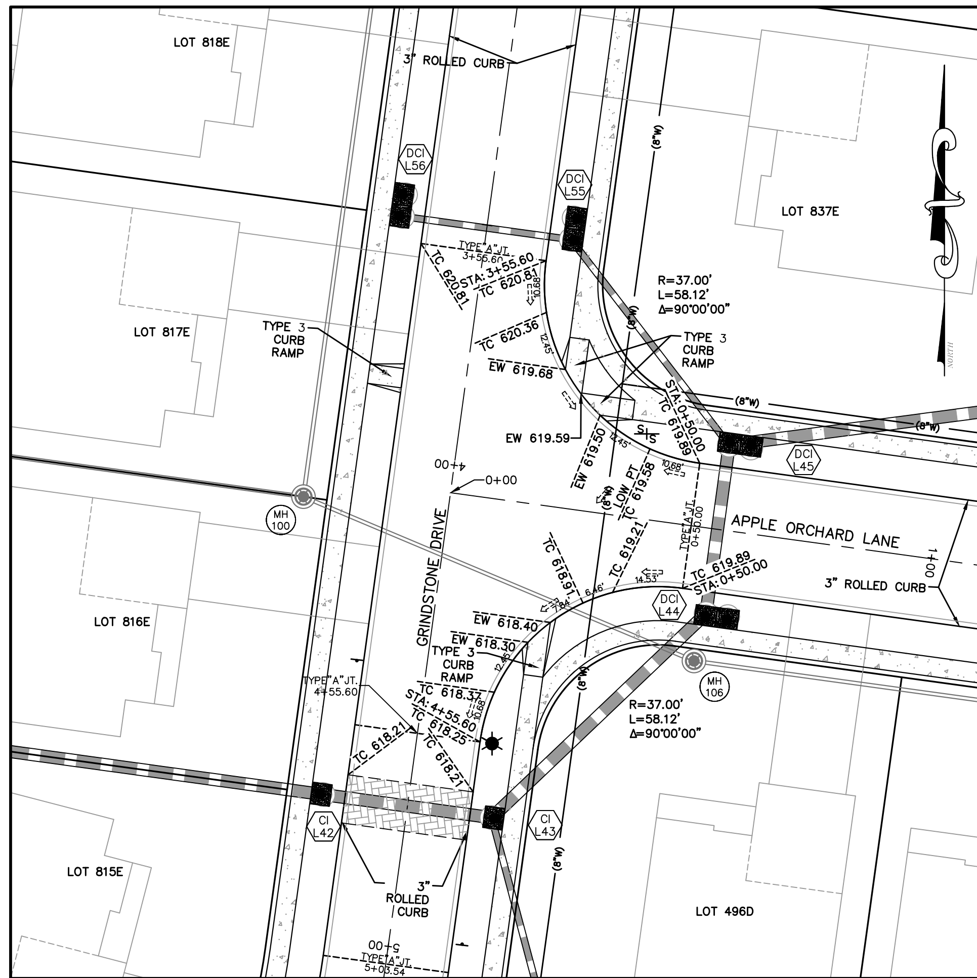
INTERSECTION DETAIL GRINDSTONE DRIVE & APPLE ORCHARD LANE SCALE: 1"=20'
