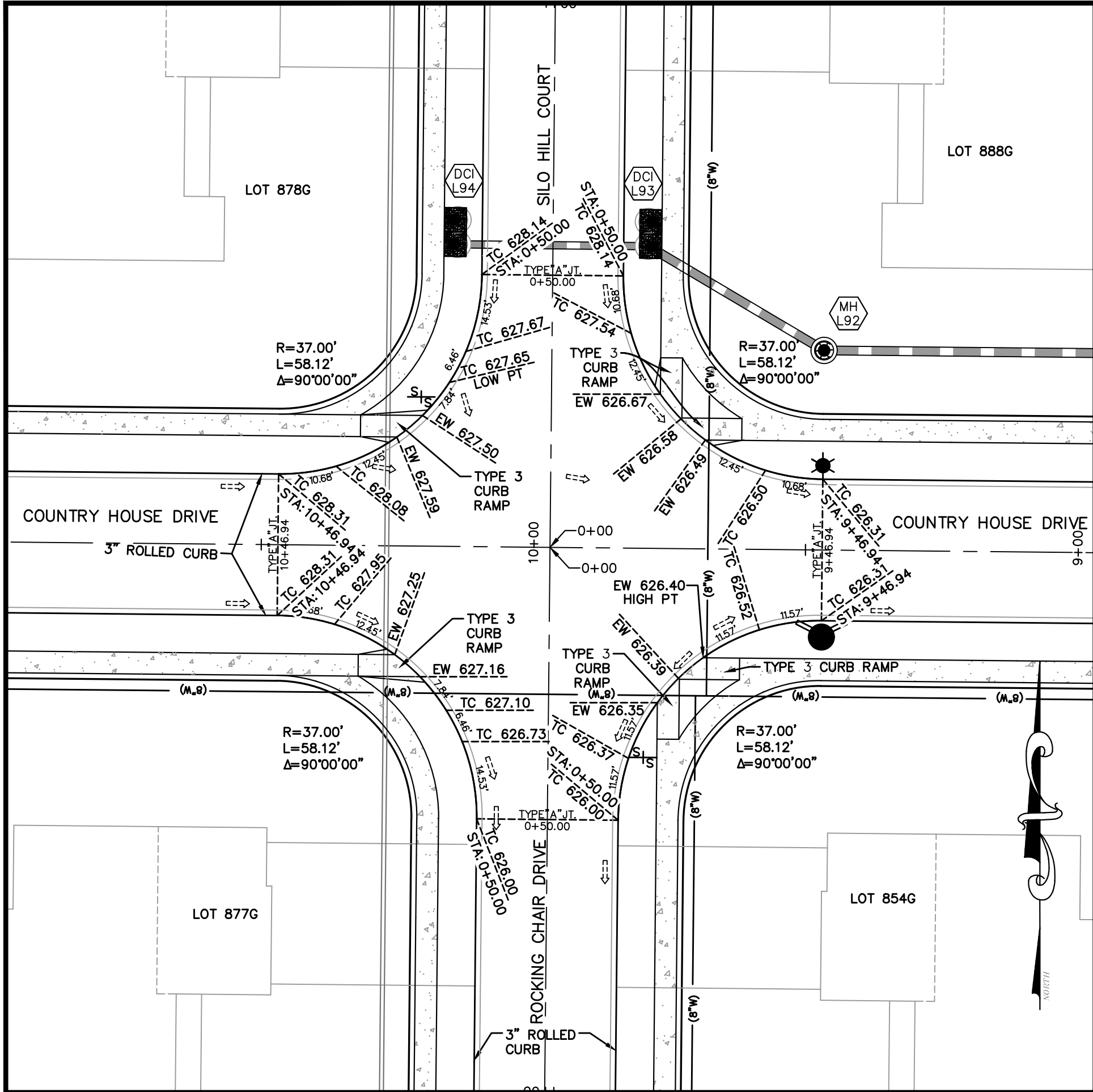
INTERSECTION DETAIL COUNTRY HOUSE DRIVE AT ROCKING CHAIR DRIVE & SILO HILL COURT SCALE: 1"=20'
