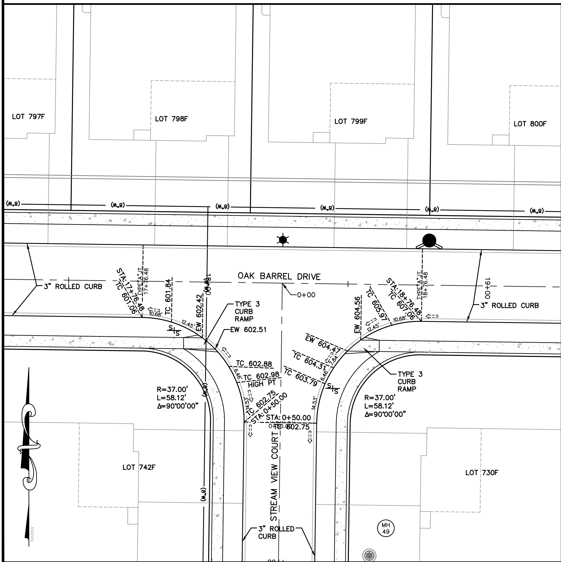
INTERSECTION DETAIL OAK BARREL DRIVE & STREAM VIEW COURT SCALE: 1"=20'
