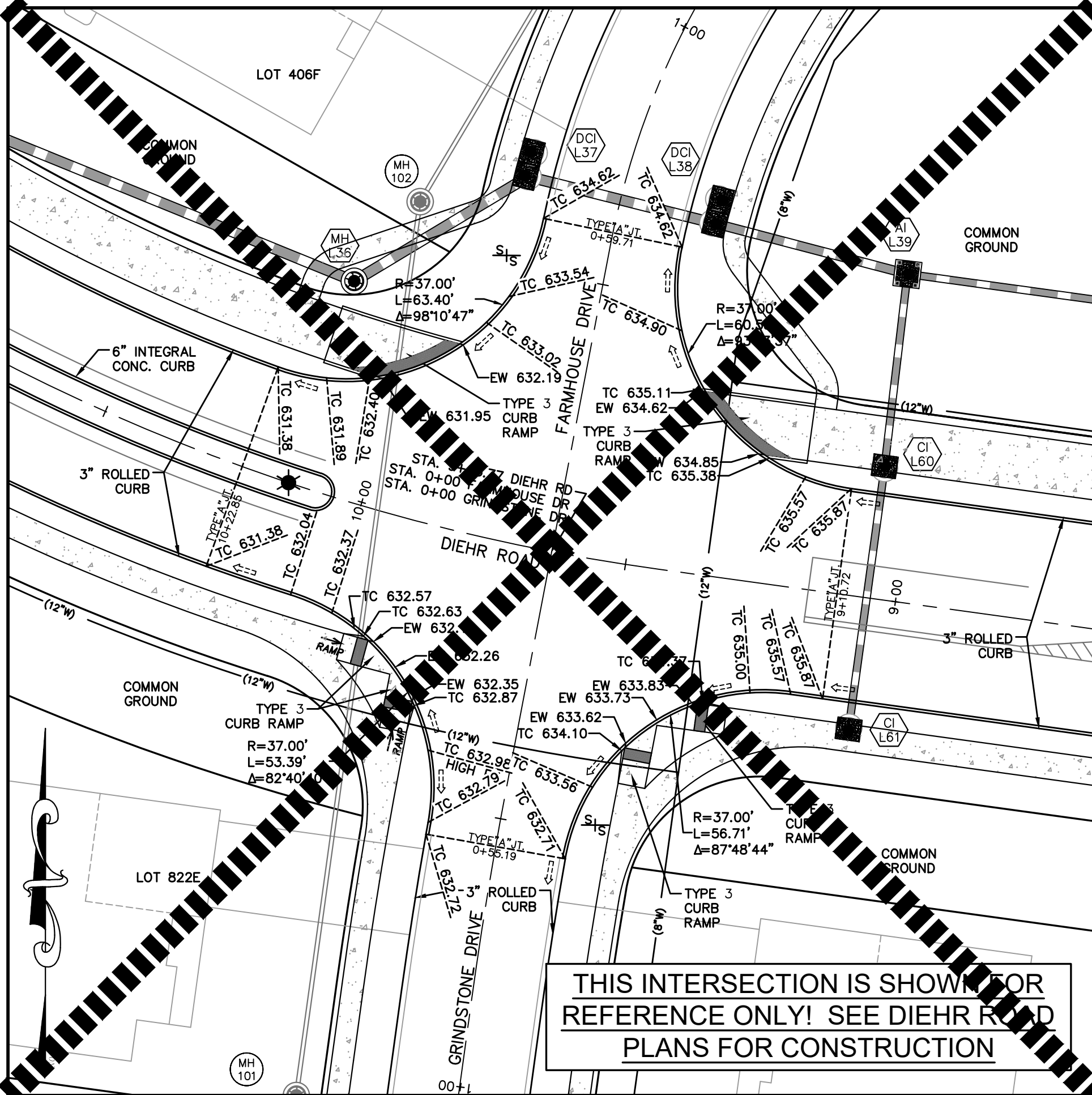
INTERSECTION DETAIL DIEHR ROAD AT GRINDSTONE DRIVE & FARMHOUSE DRIVE SCALE: 1"=20'
