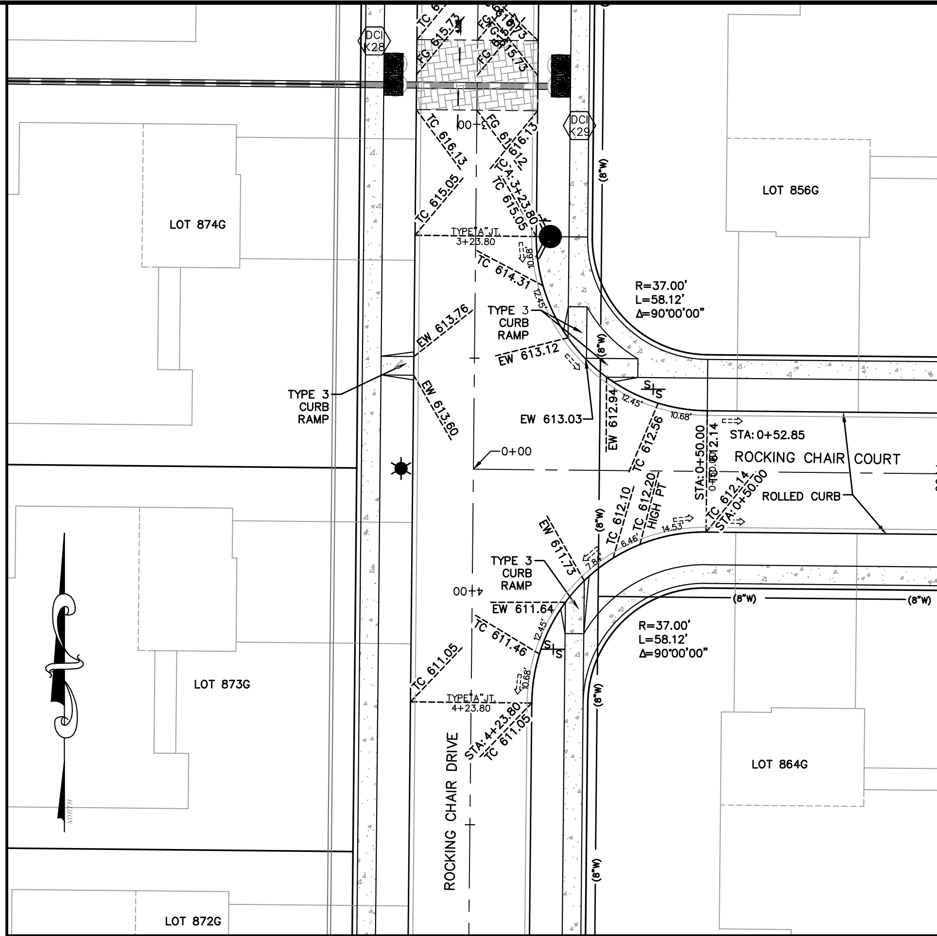
INTERSECTION DETAIL ROCKING CHAIR DRIVE & ROCKING CHAIR COURT SCALE: 1"=20'
