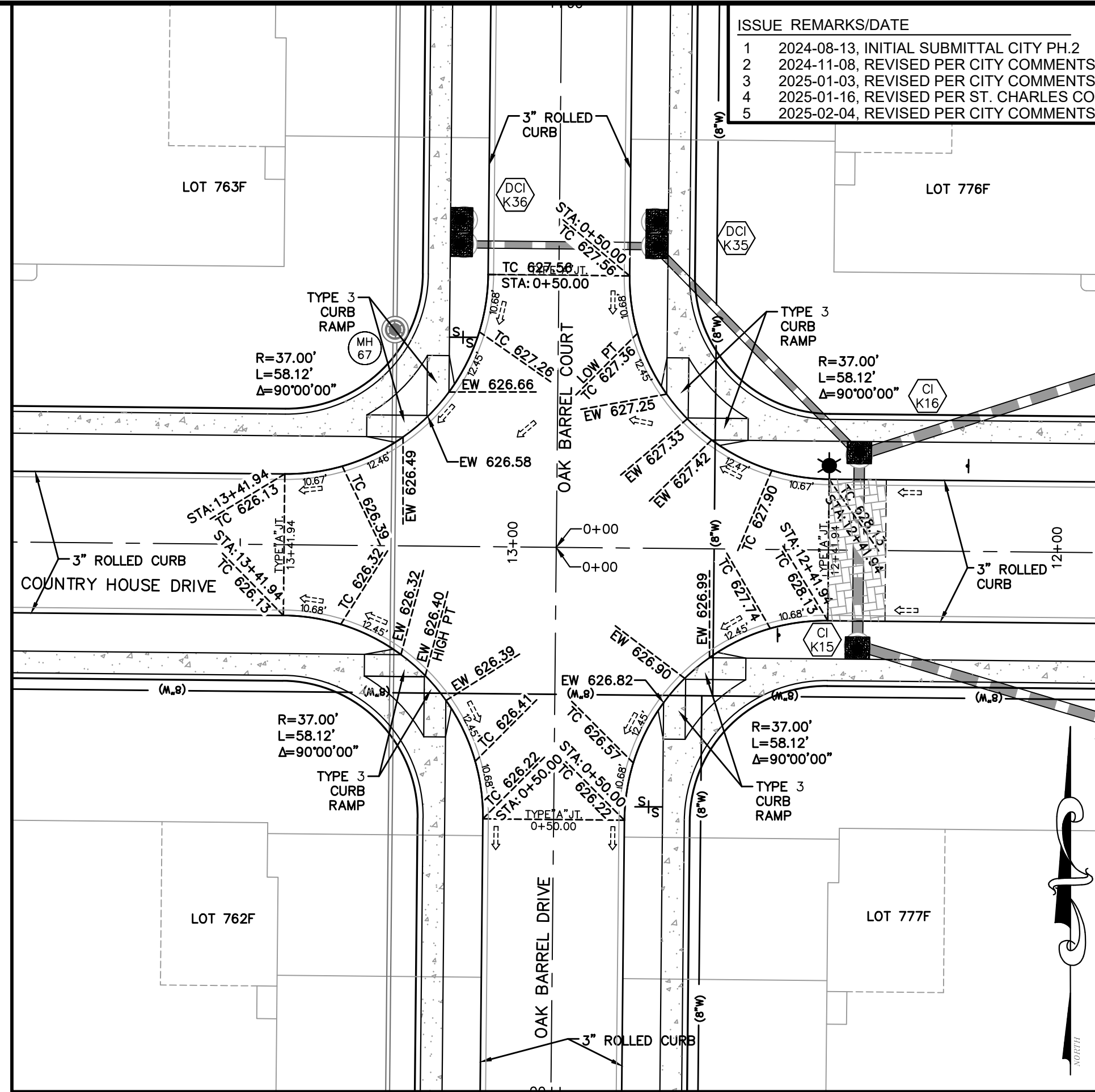
INTERSECTION DETAIL COUNTRY HOUSE DRIVE AT OAK BARREL DRIVE & OAK BARREL COURT SCALE: 1"=20'
