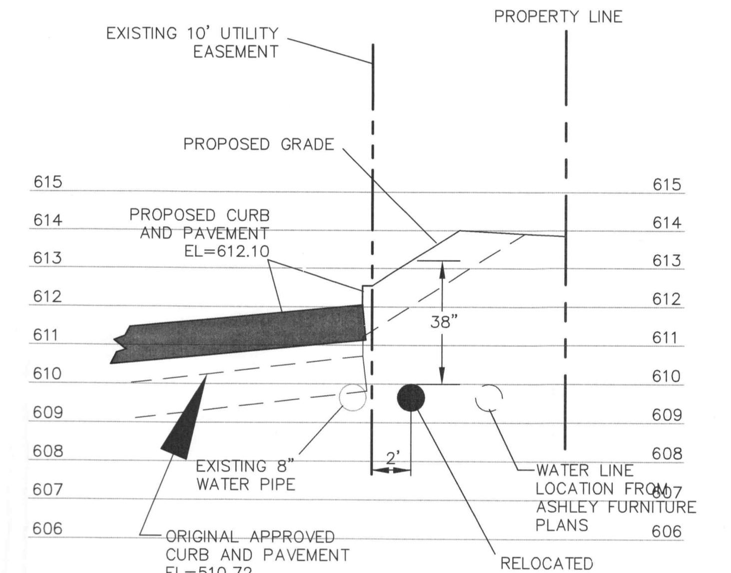
WATER LINE DETAIL
