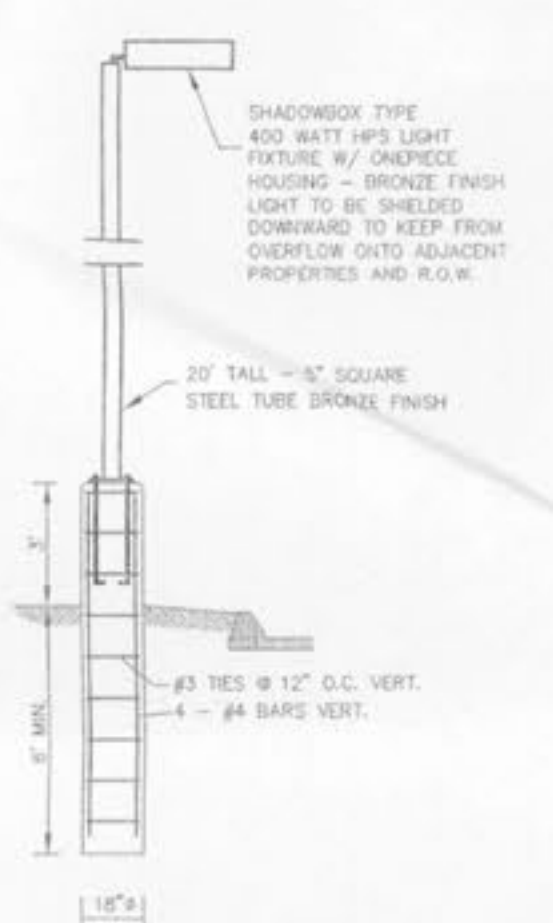
LIGHT POLE & BASE NOT TO SCALE
