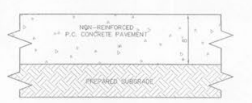
TRASH ENCLOSURE PAVEMENT DETAIL NOT TO SCALE
