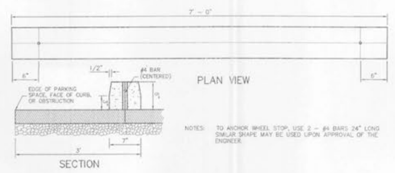
PRECAST CONCRETE WHEELSTOP
