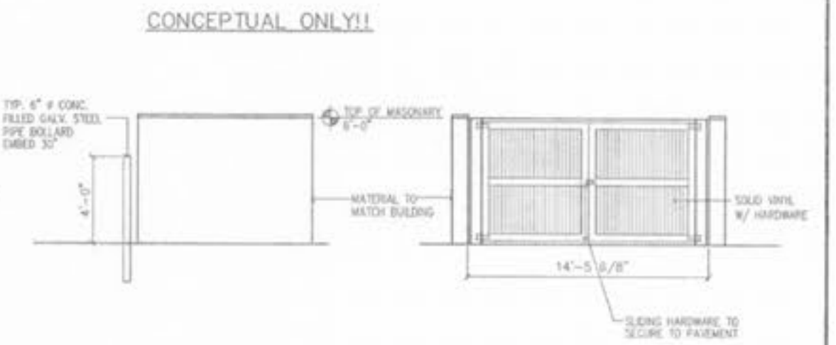
2. ELEVATION NOT TO SCALE
