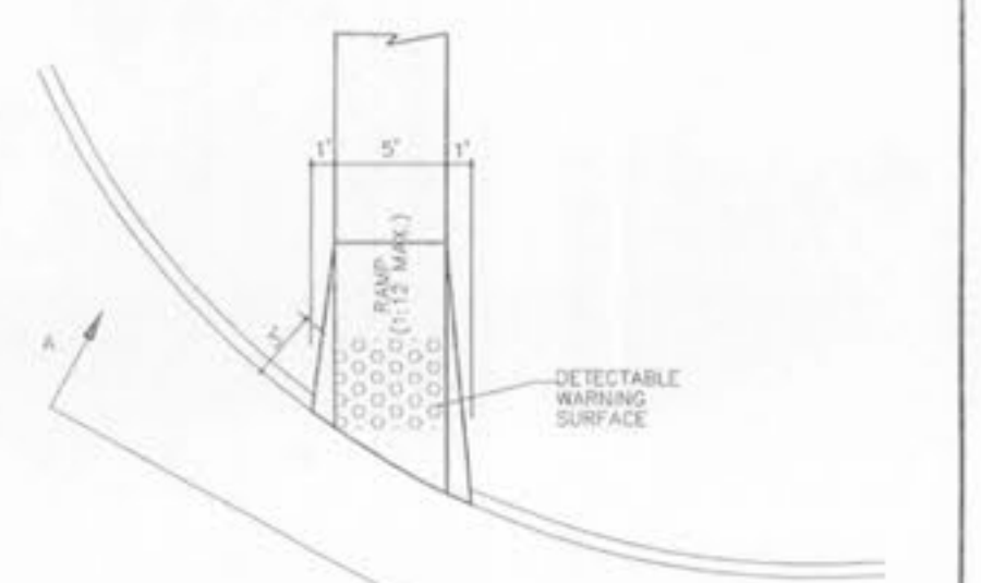
TYPICAL DETAIL OF DETECTABLE WARNING SURFACE NOT TO SCALE
