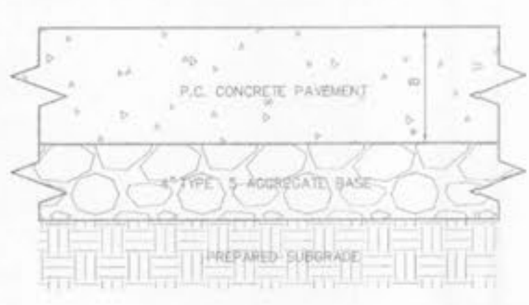
ENTRANCE PAVEMENT DETAIL NOT TO SCALE
