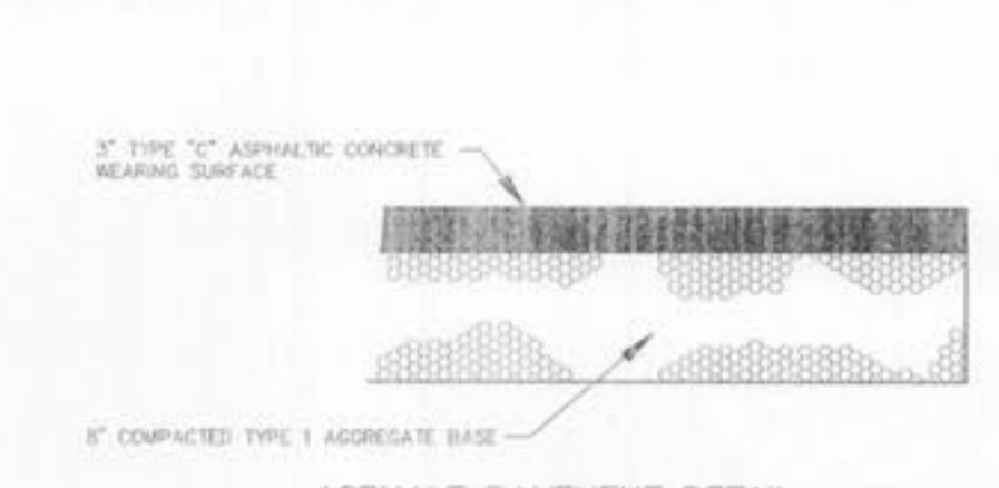
ASPHALT PAVEMENT DETAIL NOT TO SCALE
