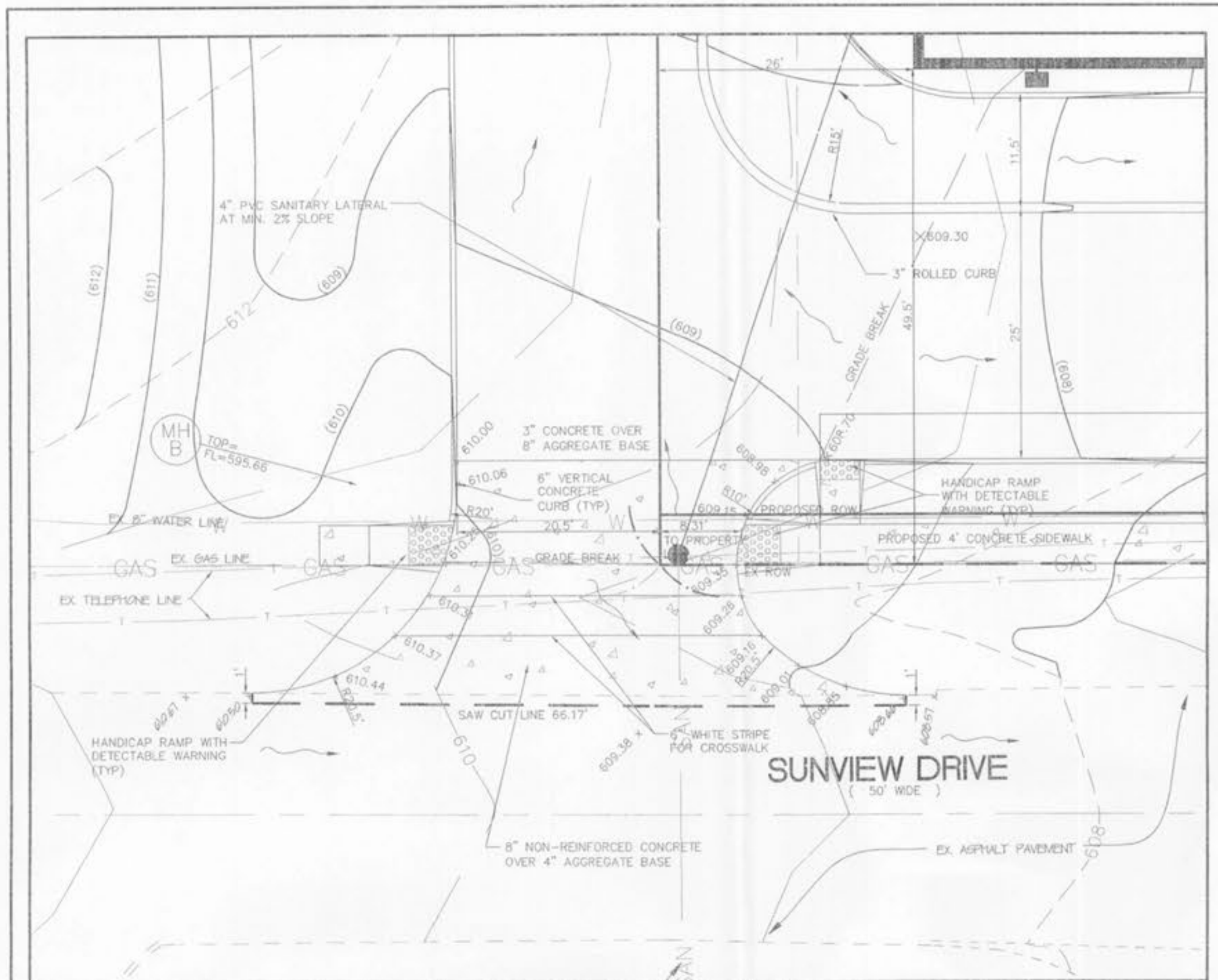
SUNVIEW DRIVE ENTRANCE DETAIL SCALE: 1"=10'
