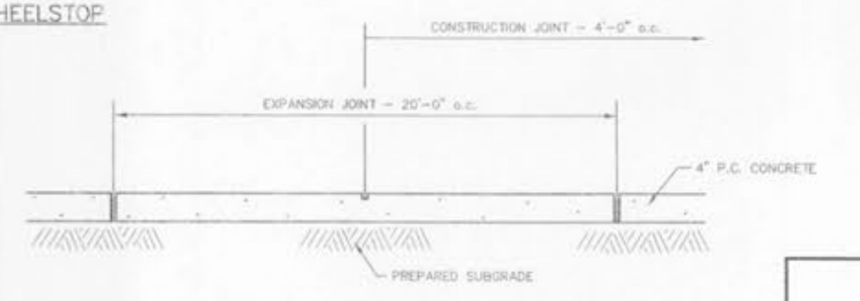
TRASH ENCLOSURE PAVEMENT DETAIL NOT TO SCALE
