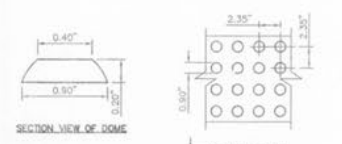
SECTION VIEW OF DOME NOT TO SCALE
