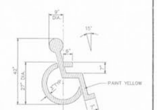
PAINTED HANDICAPPED PARKING SYMBOL NOT TO SCALE
