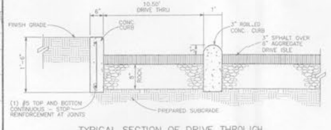
TYPICAL SECTION OF DRIVE THROUGH NOT TO SCALE
