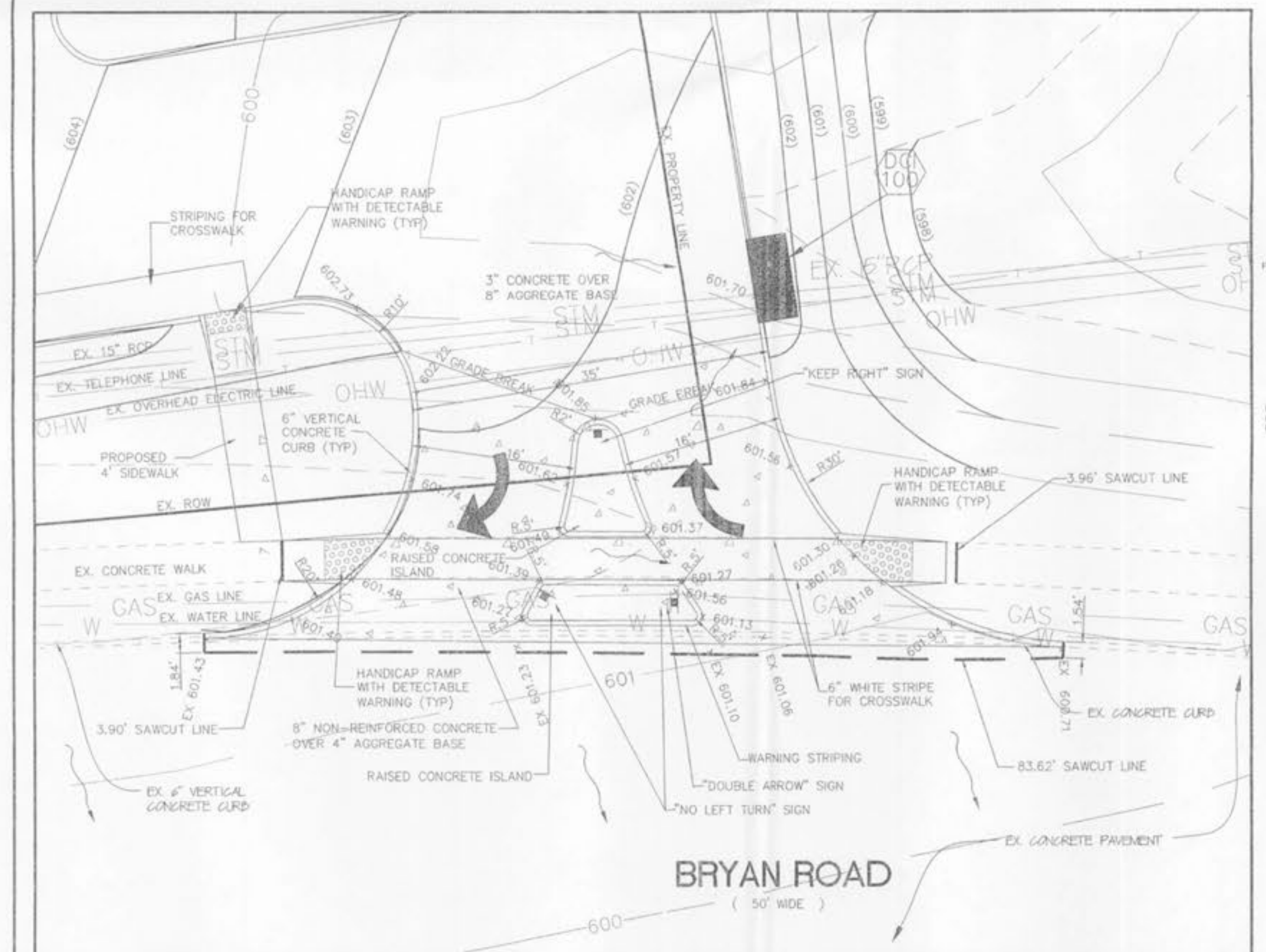
BRYAN ROAD ENTRANCE DETAIL SCALE: 1"=10'
