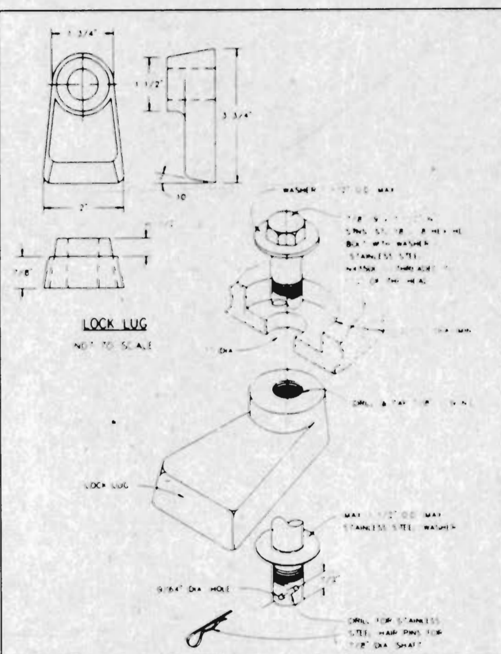
LOCKING DEVICE FOR TYPE 'N' LOCK TYPE MANHOLE COVER METROPOLITAN ST. LOUIS SEWER DISTRICT Standard Details of Sewer Construction Dr. J.L.G. / Ch. J.C.K. / 1992 / SHEET 52
