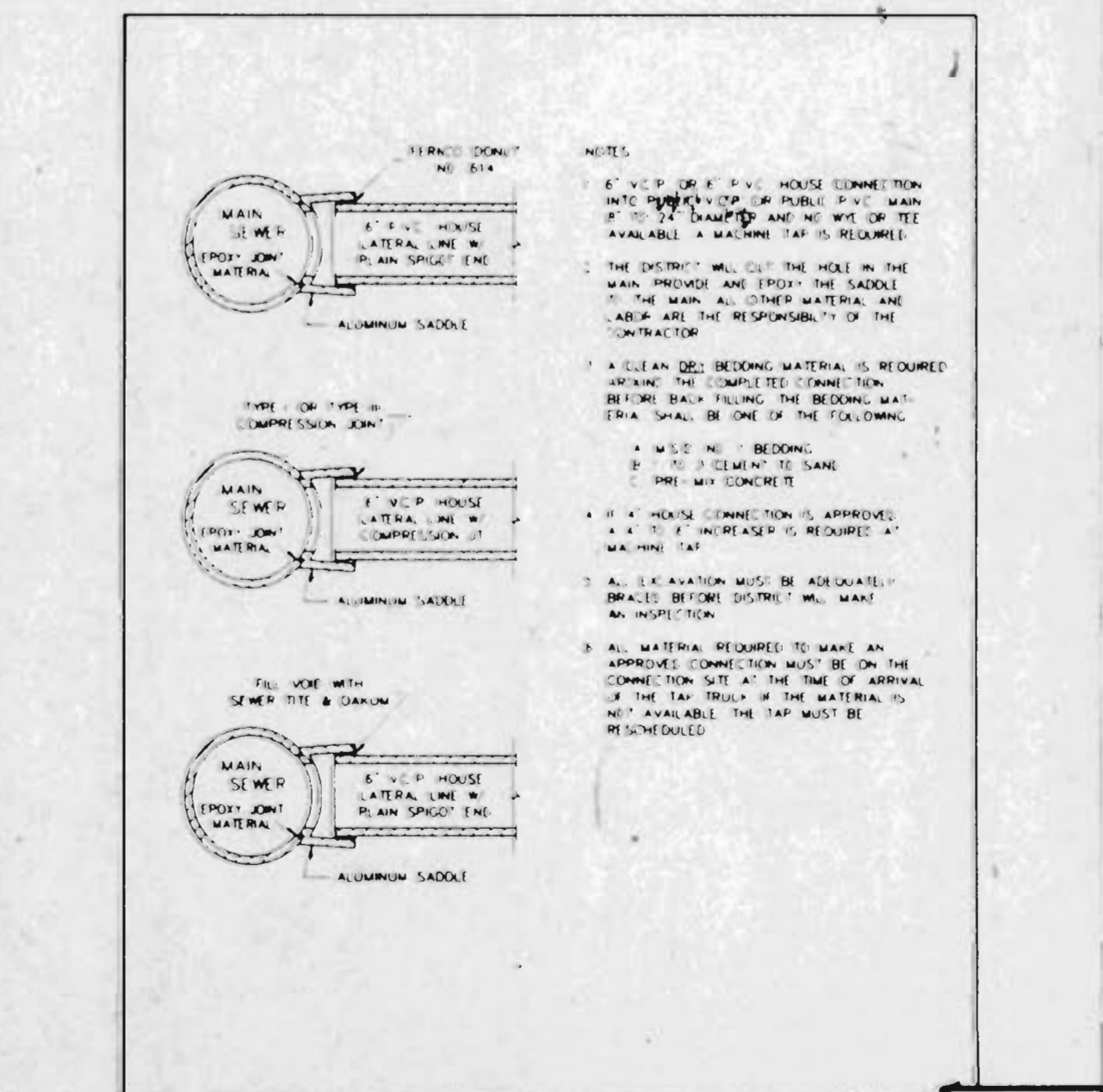
MACHINE TAP METROPOLITAN ST. LOUIS SEWER DISTRICT Standard Details of Sewer Construction Dr. W.S.H. / Ch. J.C.K. / 1992 / SHEET 60
