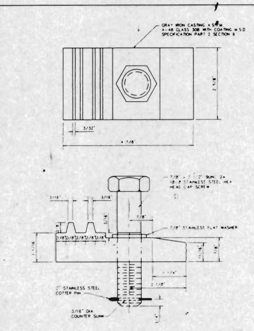
LOCKING DEVICE FOR TYPE 'T' LOCK TYPE MANHOLE COVER METROPOLITAN ST. LOUIS SEWER DISTRICT Standard Details of Sewer Construction Dr. R.G.W. / Ch. J.C.K. / 1992 / SHEET 51
