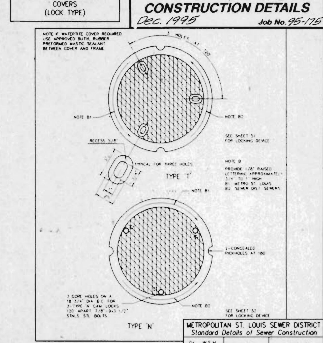
CAST IRON MANHOLE COVERS (LOCK TYPE) HIDDEN MEADOWS CONSTRUCTION DETAILS Dec. 1995 Job No. 95-175 METROPOLITAN ST. LOUIS SEWER DISTRICT Standard Details of Sewer Construction Dr. W.S.H. / Ch. J.C.K. / 1992 / SHEET 50
