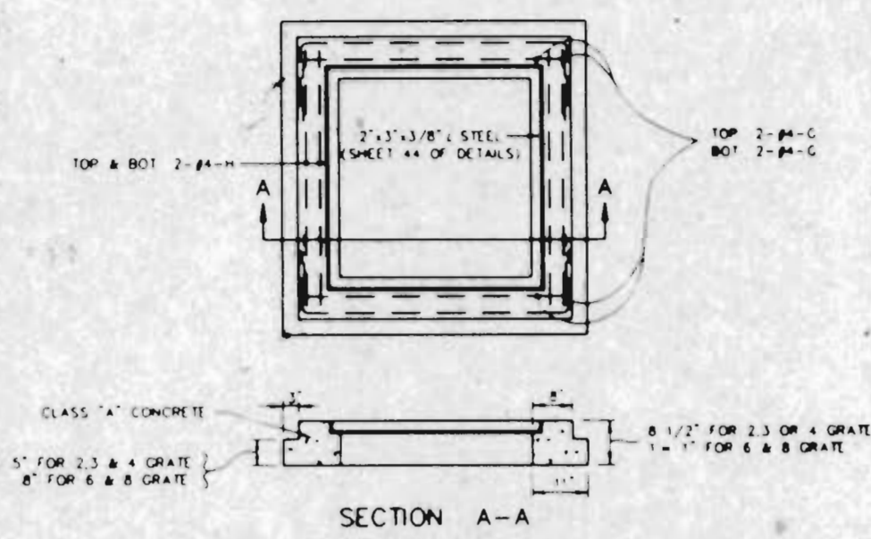
STEEL REQUIREMENTS FOR GRATE INLET SEAT METROPOLITAN ST. LOUIS SEWER DISTRICT Standard Details of Sewer Construction Dr. W.S.H. / Ch. J.C.K. / 1992 / SHEET 46
