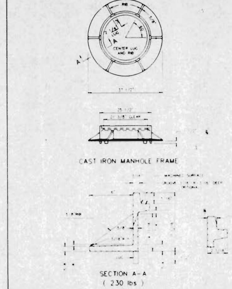
CAST IRON MANHOLE FRAME METROPOLITAN ST. LOUIS SEWER DISTRICT Standard Details of Sewer Construction Dr. G.A.P. / Ch. J.C.K. / 1992 / SHEET 48
