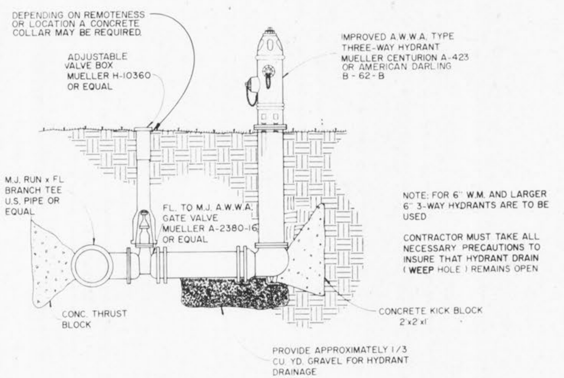
FIRE HYDRANT INSTALLATION DETAIL N.T.S.
