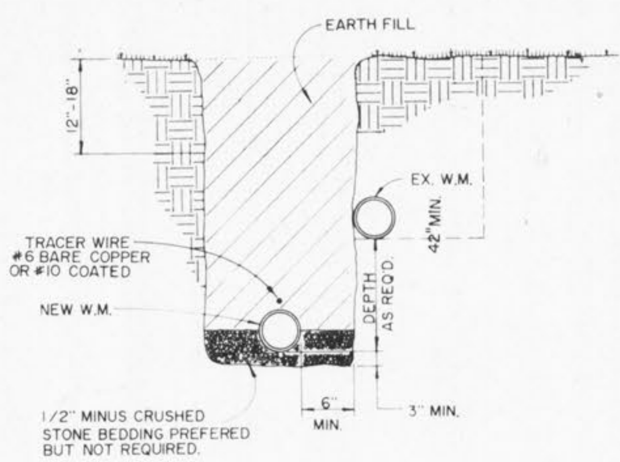
TYPICAL WATER MAIN LOWERING DETAIL N.T.S.
