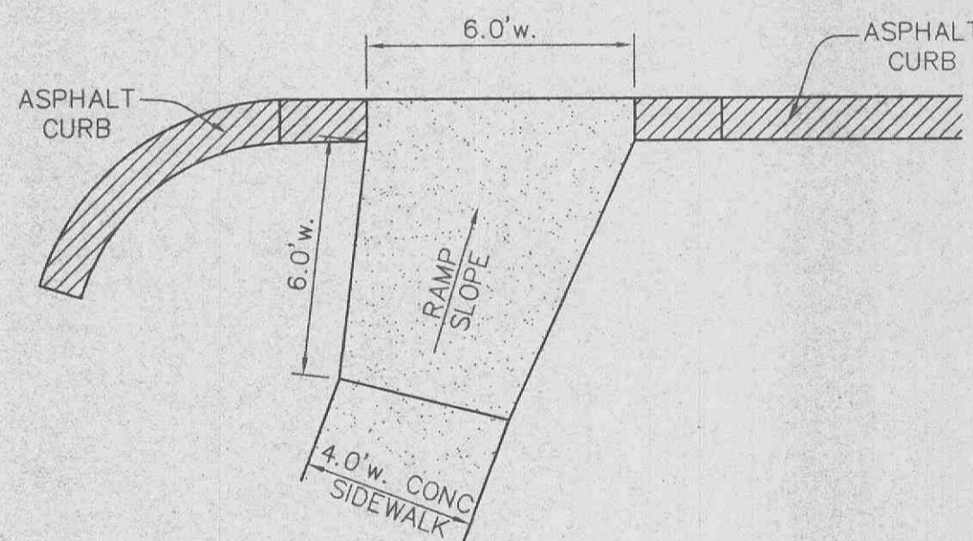
DETAIL "F" AT HANDICAP RAMP NO SCALE
