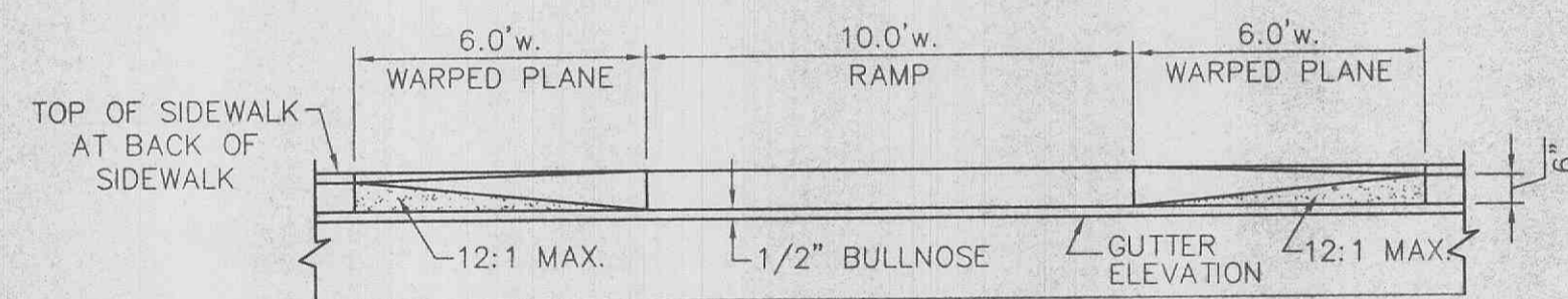
SECTION "C"-"C" AT HANDICAP RAMP NO SCALE
