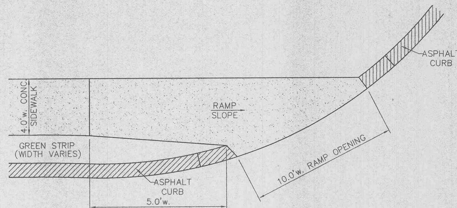
DETAIL "D" AT HANDICAP RAMP NO SCALE
