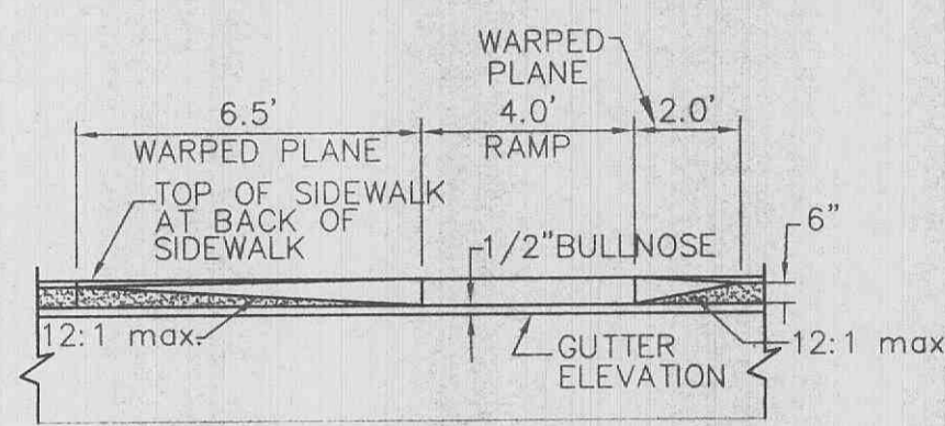
SECTION "B"-"B" AT HANDICAP RAMP NO SCALE
