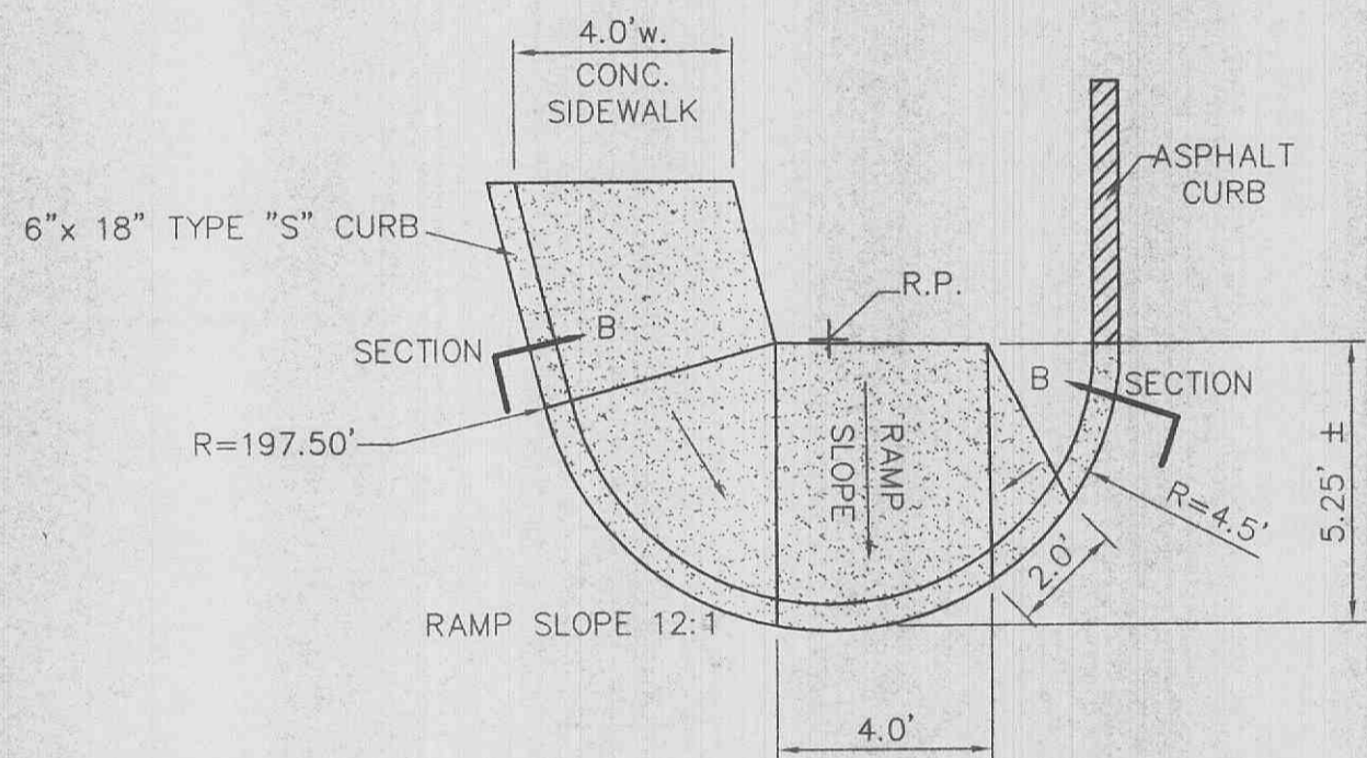
DETAIL "B" AT HANDICAP RAMP NO SCALE
