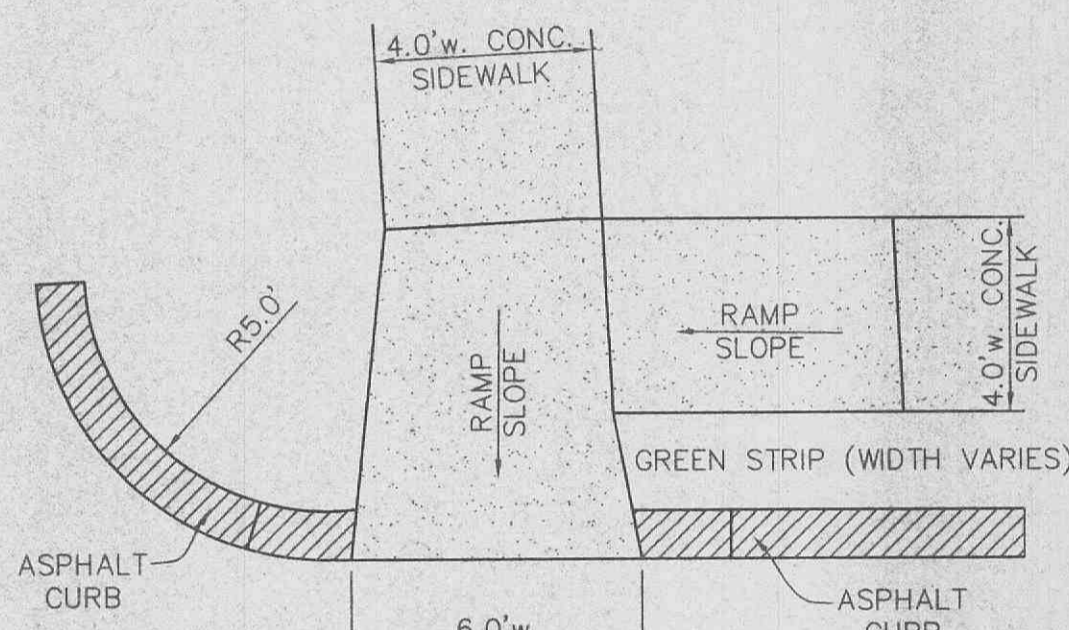
DETAIL "E" AT HANDICAP RAMP NO SCALE
