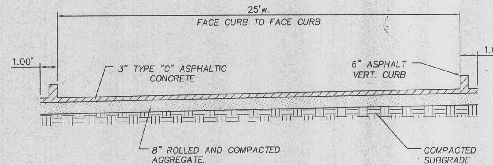
TYPICAL ROAD SECTION N.T.S.
