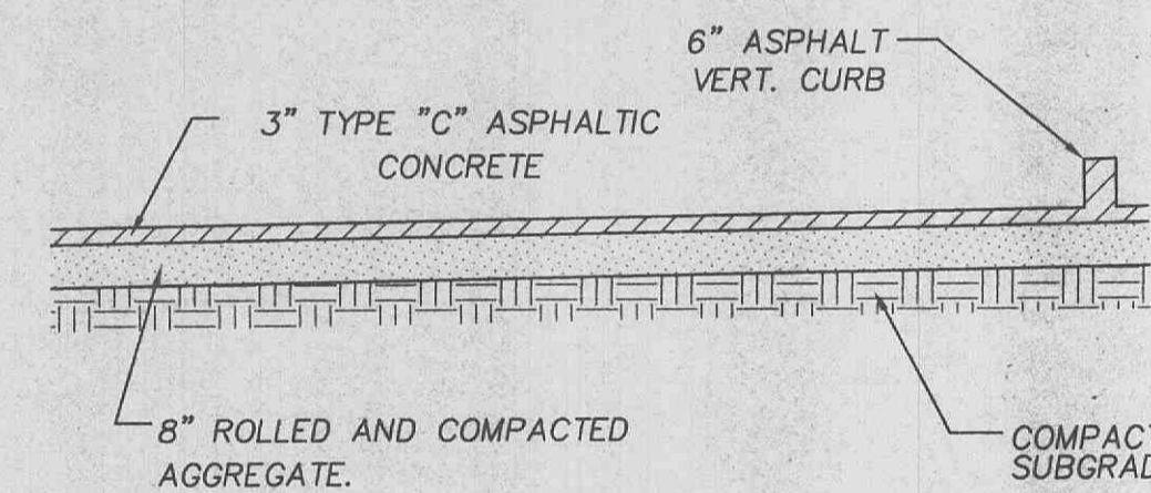
TYPICAL PARKING AREA SECTION N.T.S.
