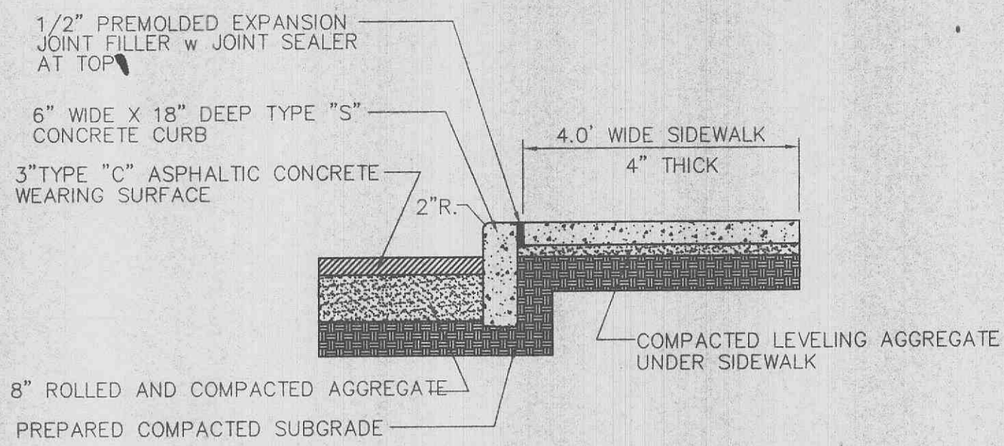
DETAIL "A" AT CONCRETE WALK AND CURB NO SCALE
