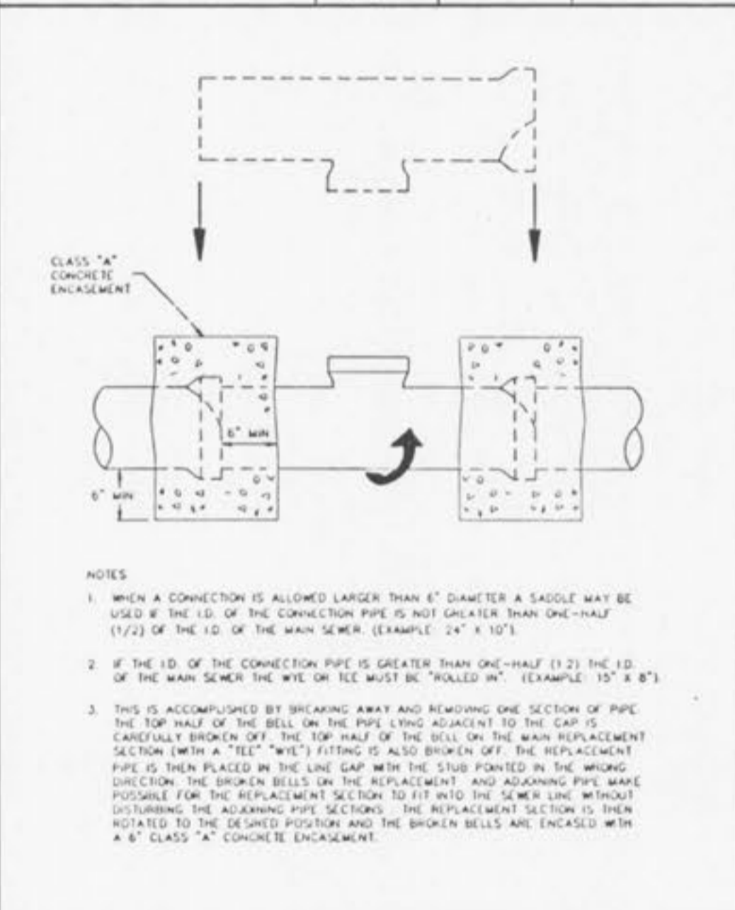
"ROLL-IN" (FOR EXISTING CLAY OR CONCRETE PIPE) METROPOLITAN ST. LOUIS SEWER DISTRICT Standard Details of Sewer Construction Dr. D.A.B. / Ch. J.C.K. / 1992 / SHEET 63
