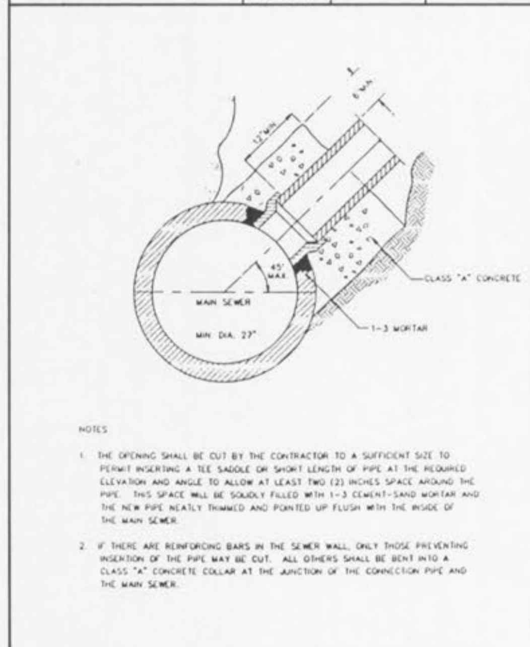
HOUSE CONNECTIONS ALLOWED BY TEE SADDLE METROPOLITAN ST. LOUIS SEWER DISTRICT Standard Details of Sewer Construction Dr. D.A.B. / Ch. J.C.K. / 1992 / SHEET 61
