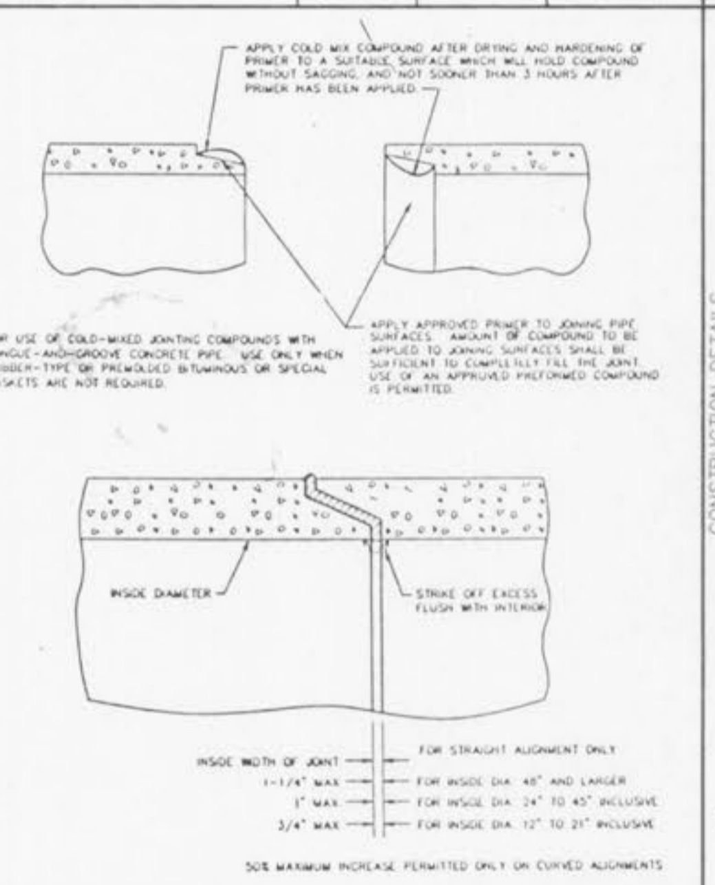
TONGUE AND GROOVE CONCRETE PIPE JOINTS METROPOLITAN ST. LOUIS SEWER DISTRICT Standard Details of Sewer Construction Dr. D.A.B. / Ch. J.C.K. / 1992 / SHEET 66
