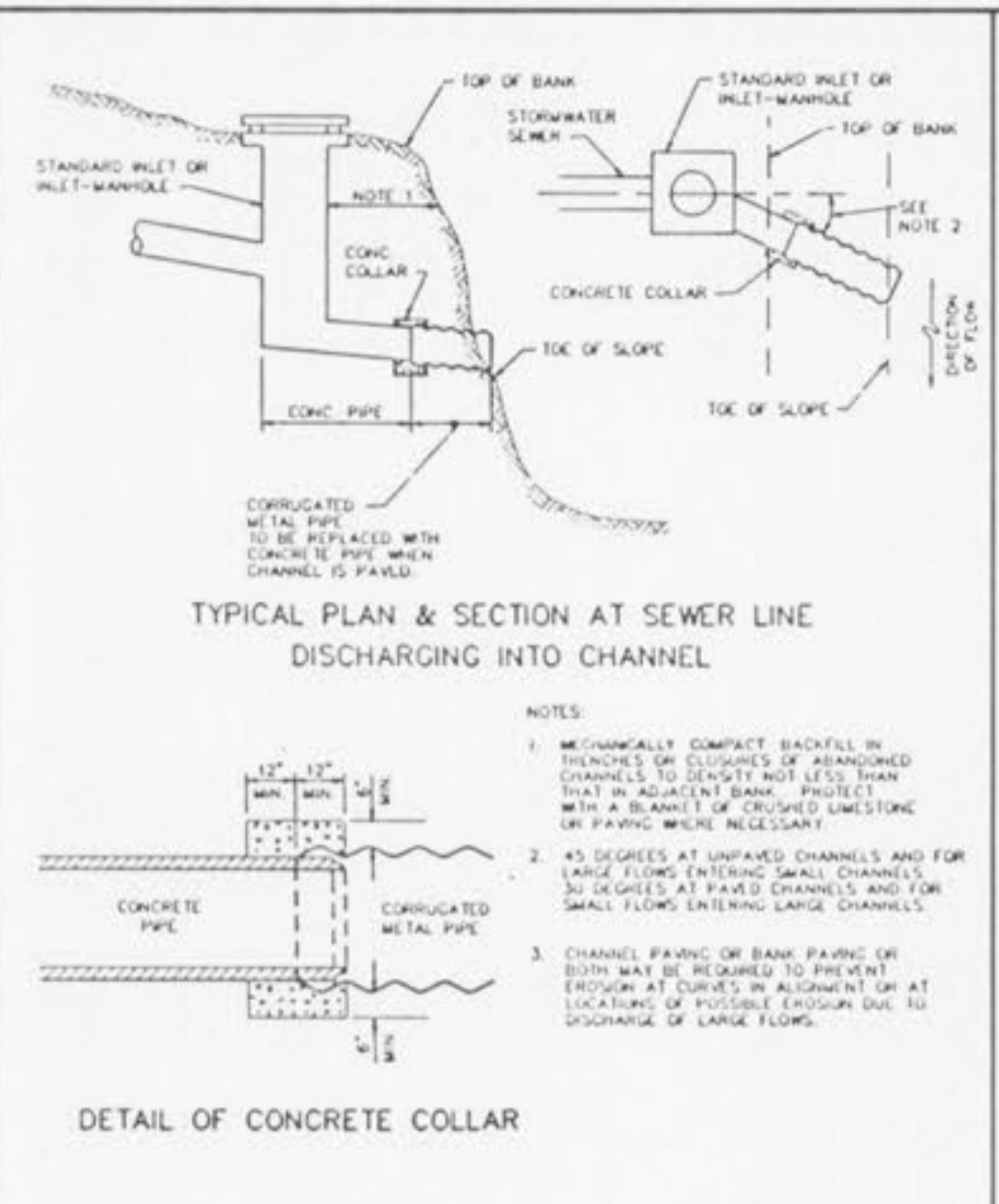
STORMWATER CHANNELS METROPOLITAN ST. LOUIS SEWER DISTRICT Standard Details of Sewer Construction Dr. R.G.W. / Ch. J.C.K. / 1992 / SHEET 58
