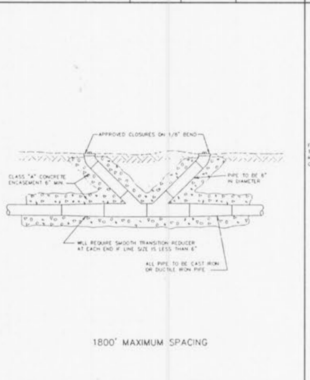
FORCE MAIN CLEANOUT (6" DIA. & SMALLER) METROPOLITAN ST. LOUIS SEWER DISTRICT Standard Details of Sewer Construction Dr. R.G.W. / Ch. J.C.K. / 1992 / SHEET 65
