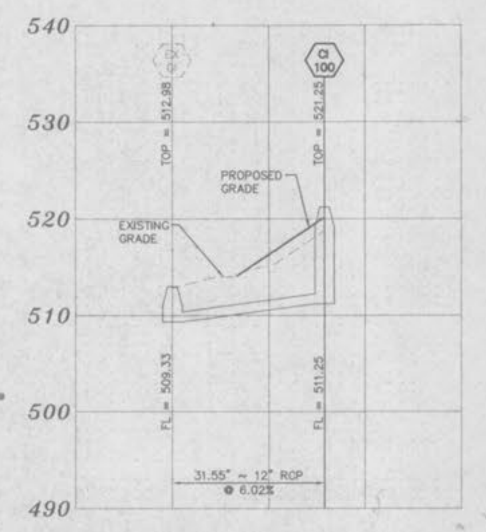
STORM SEWER PROFILE SCALE: 1" = 20' H. 1" = 10' V.
