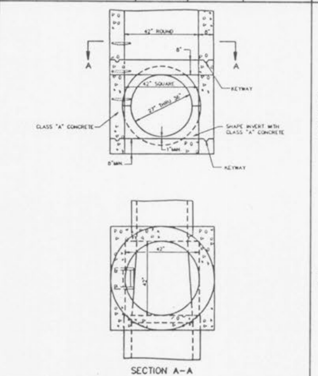
METROPOLITAN ST. LOUIS SEWER DISTRICT Standard Details of Sewer Construction Dr. W.S.H. Ch. J.C.K. 1992 SHEET 9
