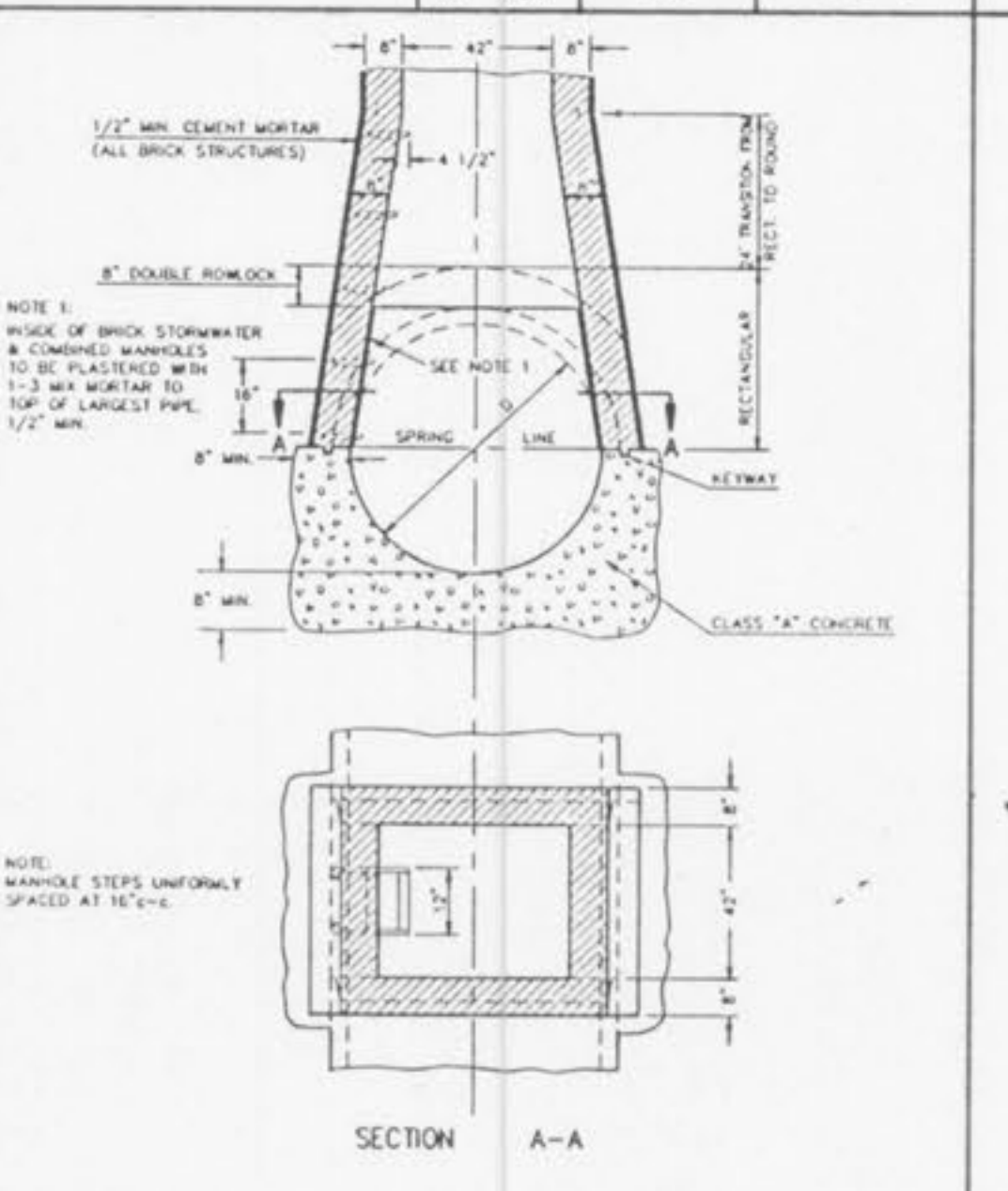
METROPOLITAN ST. LOUIS SEWER DISTRICT Standard Details of Sewer Construction Dr. D.A.B. Ch. J.C.K. 1992 SHEET 10
