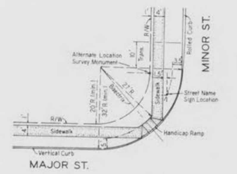
TYPICAL INTERSECTION DETAILS SIDEWALKS, STREET NAME SIGNS AND MONUMENTS
