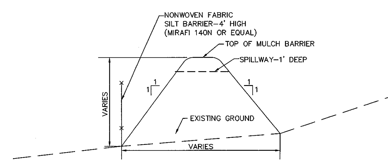
SEDIMENT TRAP MULCH BERM NOT TO SCALE
