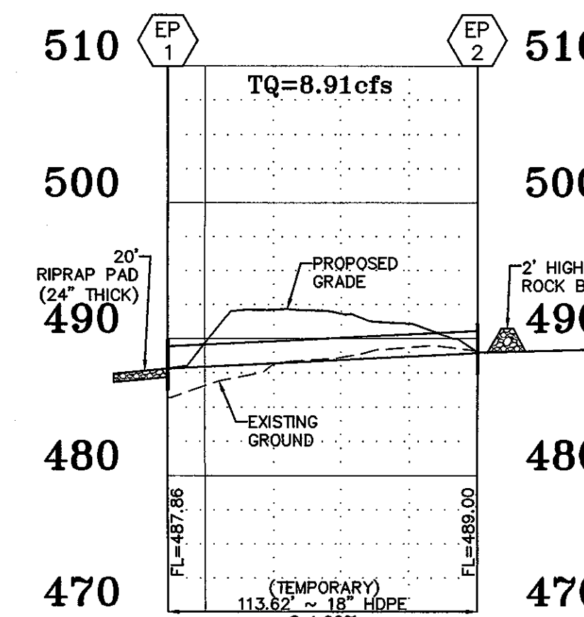
STORM SEWER PROFILE
