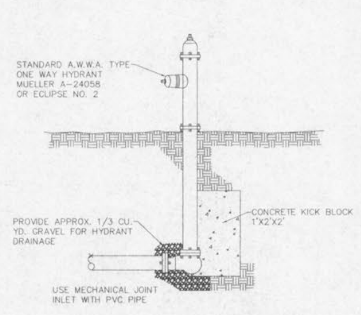
FLUSHING HYDRANT NOT TO SCALE
