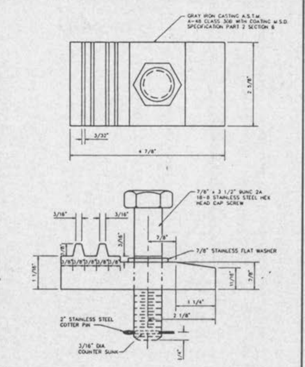
LOCKING DEVICE FOR TYPE 'J' LOCK TYPE MANHOLE COVER METROPOLITAN ST. LOUIS SEWER DISTRICT Standard Details of Sewer Construction Dr. R.C.W. Ch. J.C.K. 1992 SHEET 51
