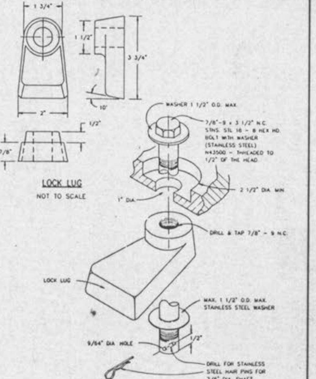
LOCKING DEVICE FOR TYPE 'M' LOCK TYPE MANHOLE COVER METROPOLITAN ST. LOUIS SEWER DISTRICT Standard Details of Sewer Construction Dr. J.L.G. Ch. J.C.K. 1992 SHEET 52
