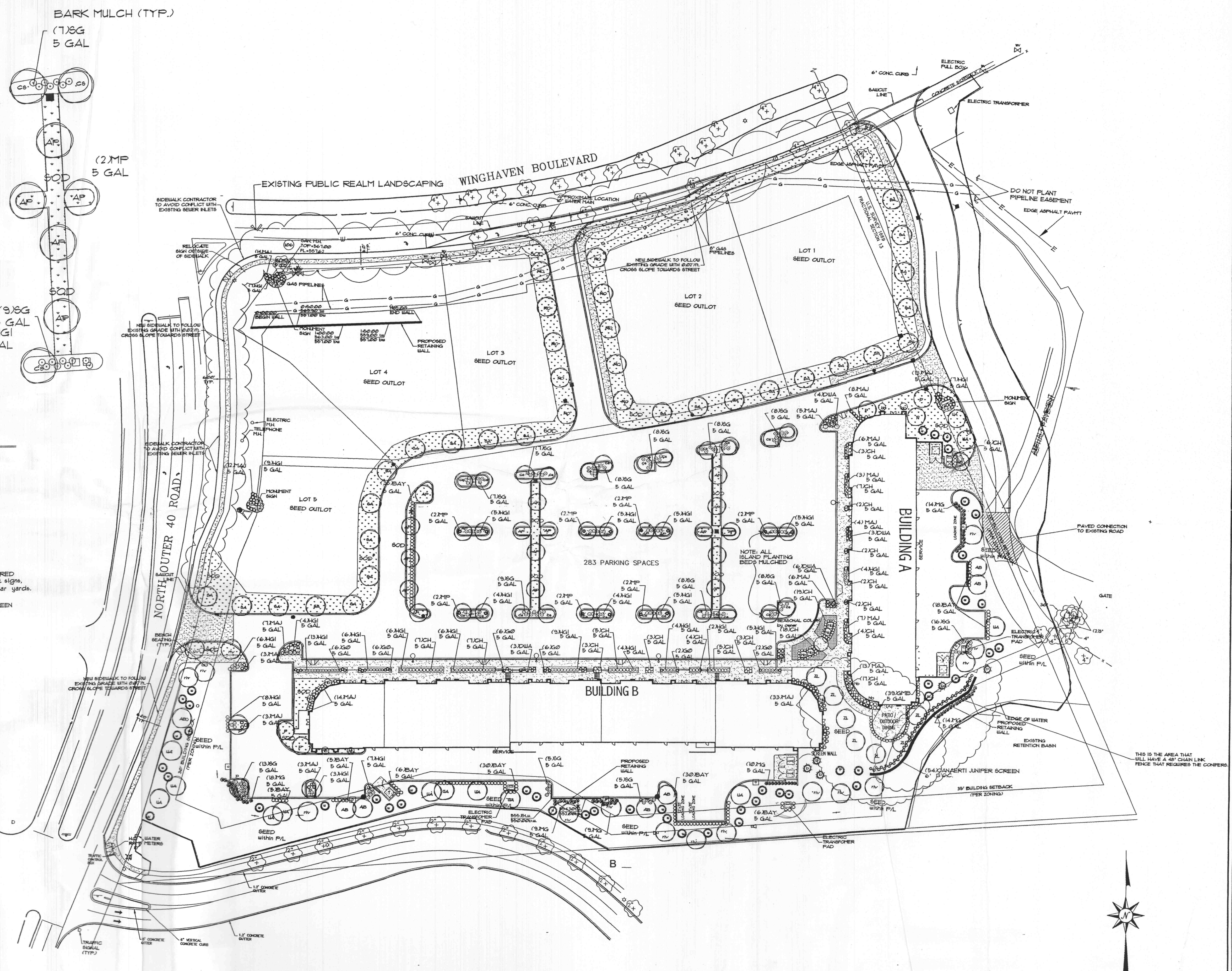
LANDSCAPE PLAN Scale: 1" = 50'
