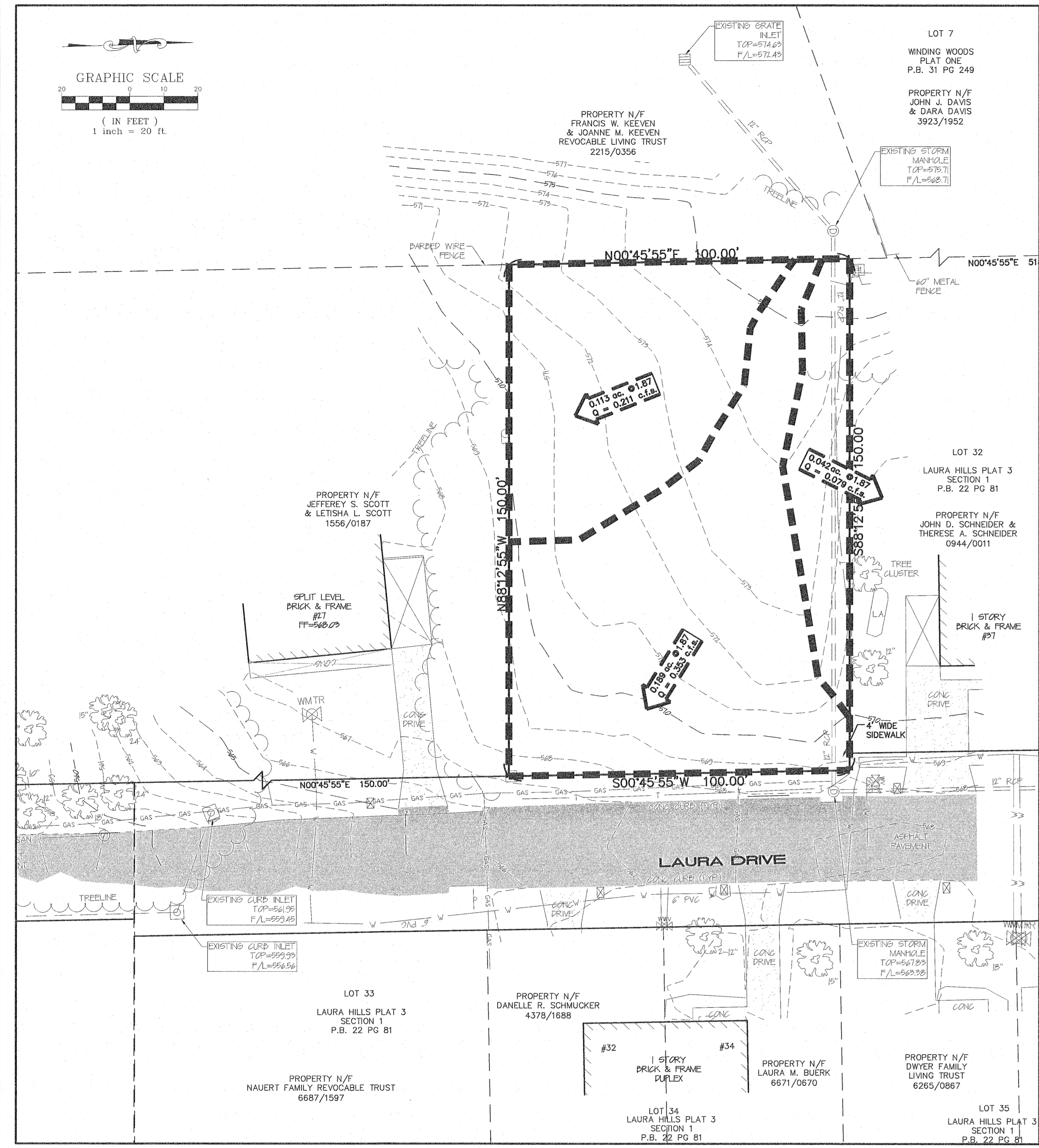
EXISTING DRAINAGE AREAS
