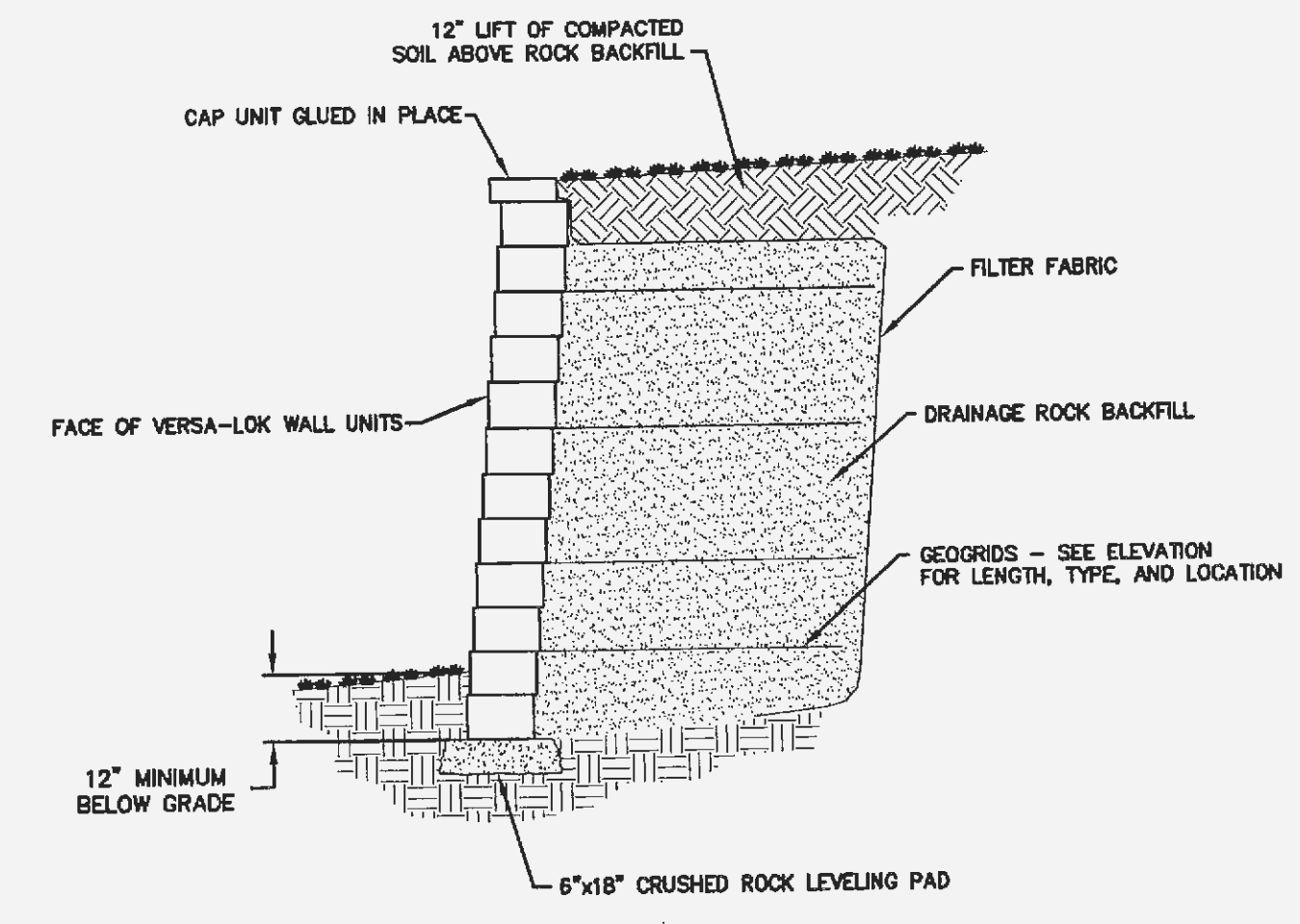
TYPICAL SECTION NOT TO SCALE
