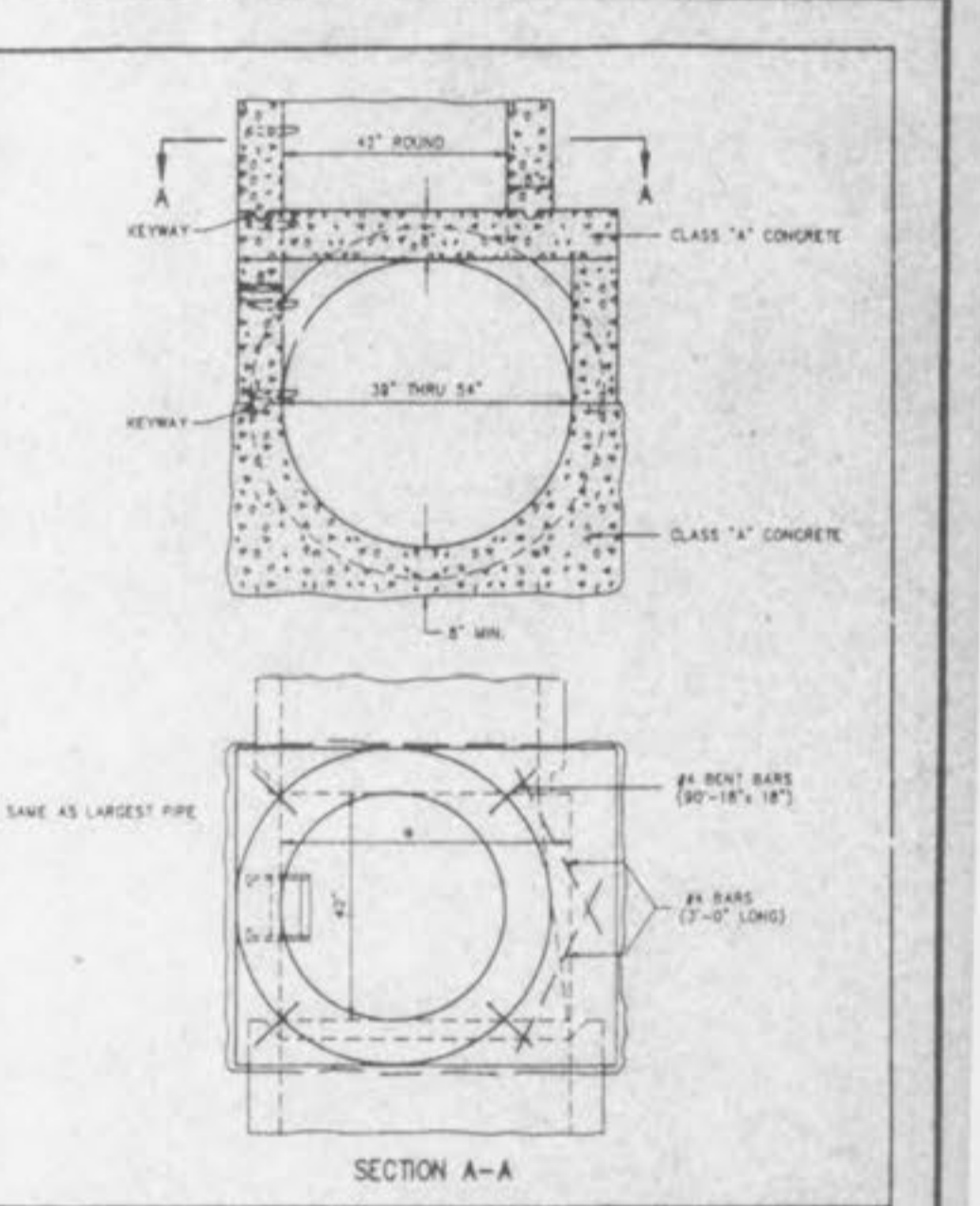
MANHOLE ON CONG. PIPE 39" THRU 54" (ALTERNATE) METROPOLITAN ST. LOUIS SEWER DISTRICT Standard Details of Sewer Construction Dr. W.S.H. Ch. J.C.K. 1992 SHEET 12
