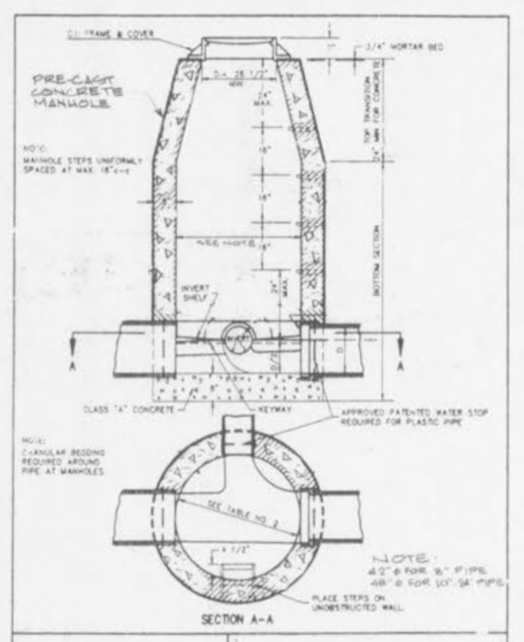
LINE MANHOLE PIPE SEWERS 8"-24" DIA. METROPOLITAN ST. LOUIS SEWER DISTRICT Standard Details of Sewer Construction Dr. W.S.H. Ch. J.C.K. 1992 SHEET 9
