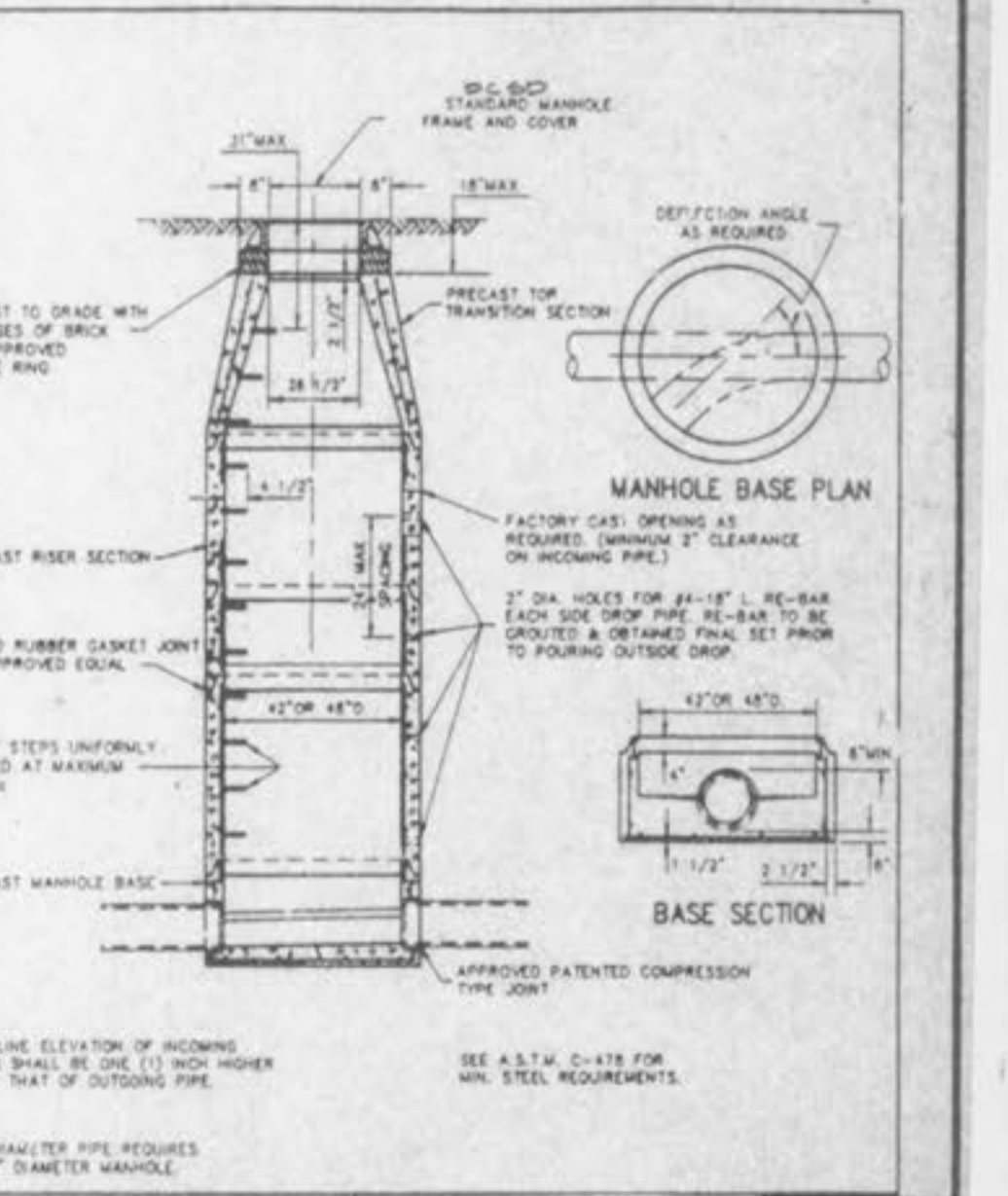
PRE-CAST CONCRETE MANHOLE FOR SEWERS 8" THROUGH 18" METROPOLITAN ST. LOUIS SEWER DISTRICT Standard Details of Sewer Construction Dr. W.S.H. Ch. J.C.K. 1992 SHEET 17
