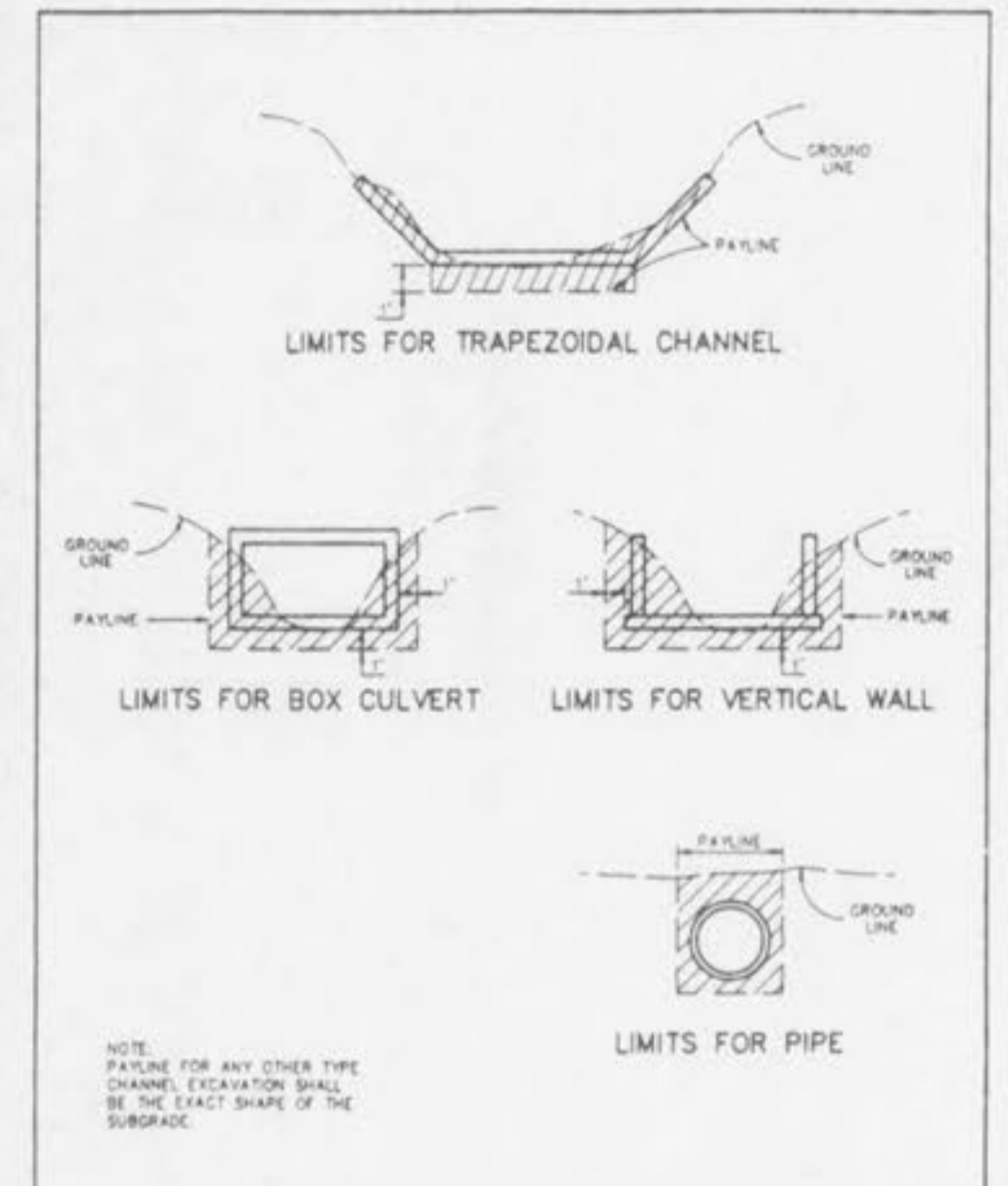
PAYLINE LIMITS FOR EXCAVATION METROPOLITAN ST. LOUIS SEWER DISTRICT Standard Details of Sewer Construction Dr. W.S.H. Ch. J.C.K. 1992 SHEET 2
