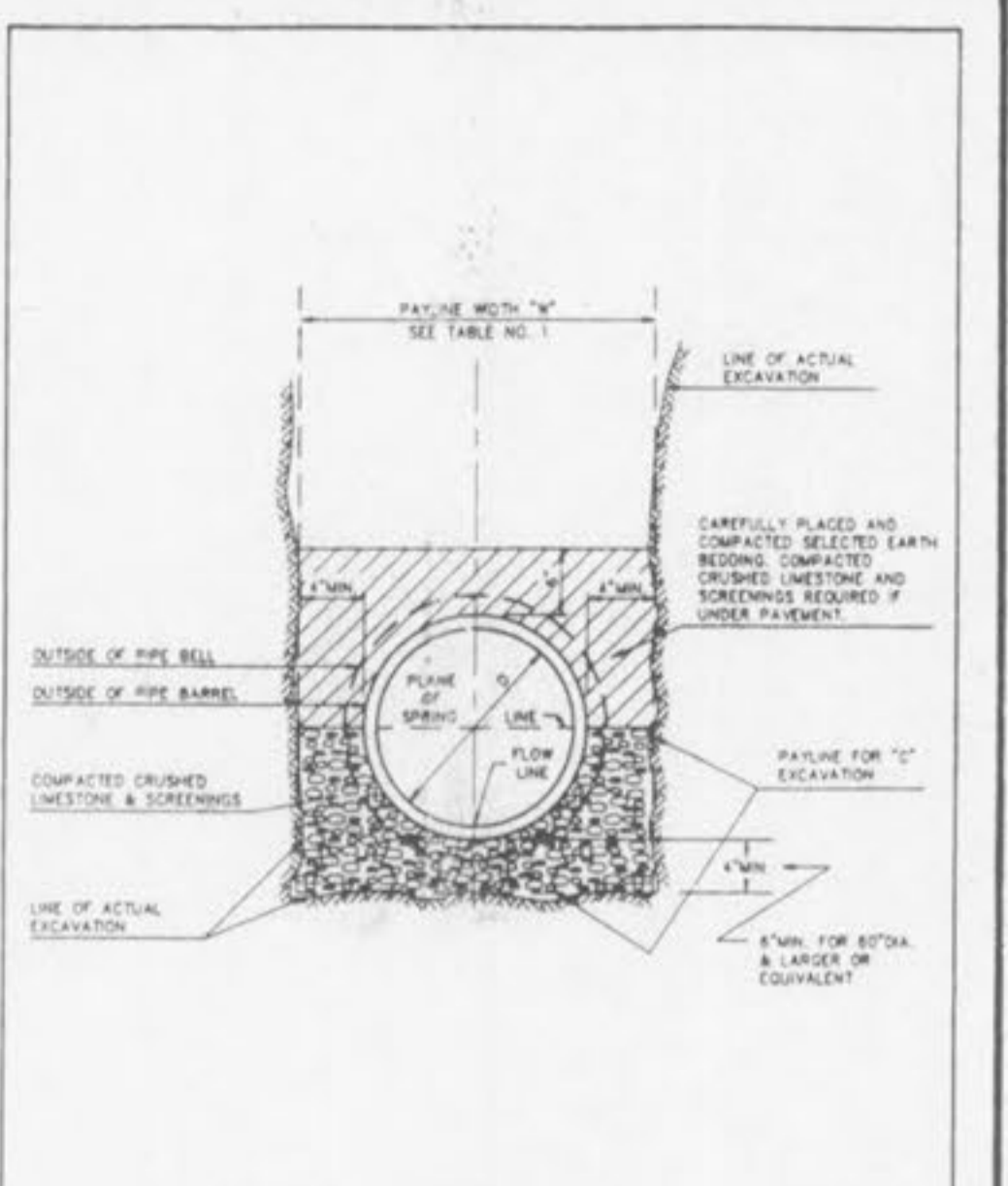
PIPE BEDDING CLASS "D" (MODIFIED FOR REINFORCED CONCRETE PIPE) METROPOLITAN ST. LOUIS SEWER DISTRICT Standard Details of Sewer Construction Dr. W.S.H. Ch. J.C.K. 1992 SHEET 5
