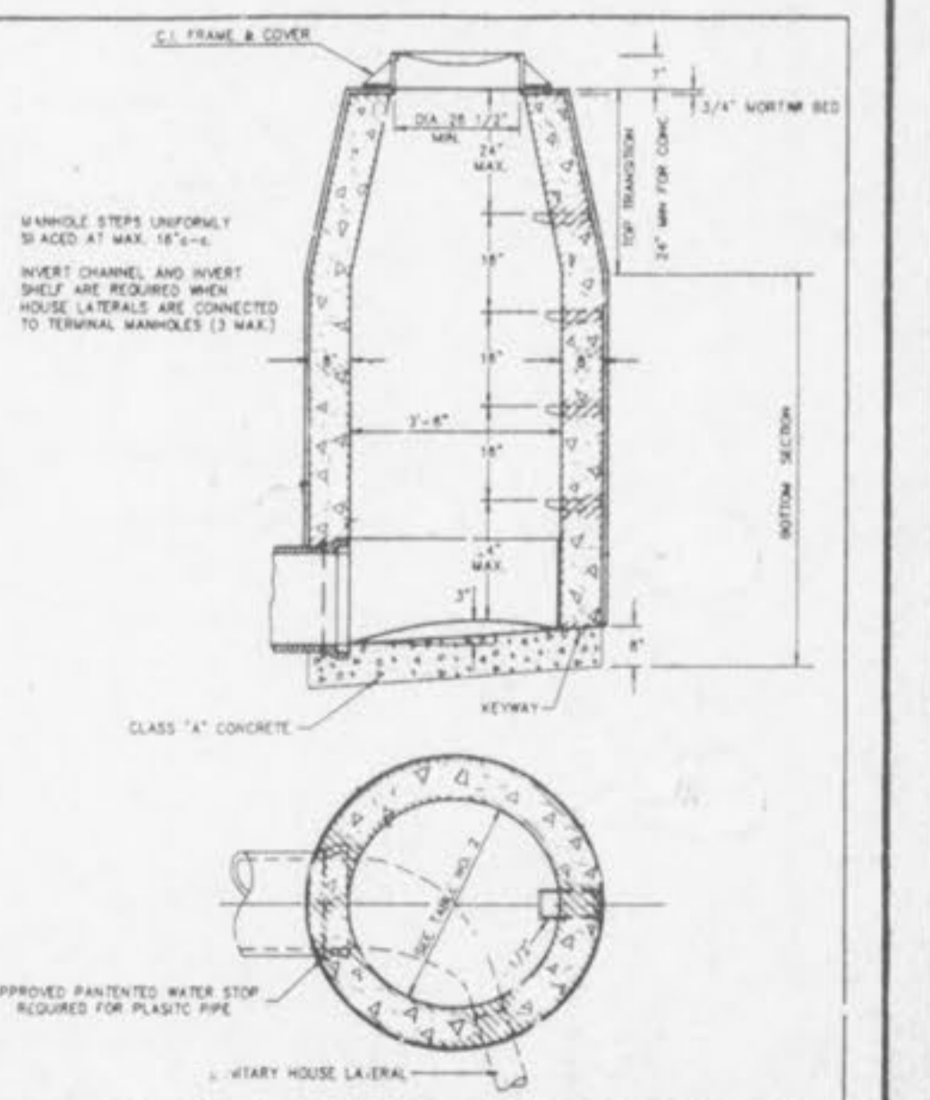
TERMINAL MANHOLE METROPOLITAN ST. LOUIS SEWER DISTRICT Standard Details of Sewer Construction Dr. W.S.H. Ch. J.C.K. 1992 SHEET 16
