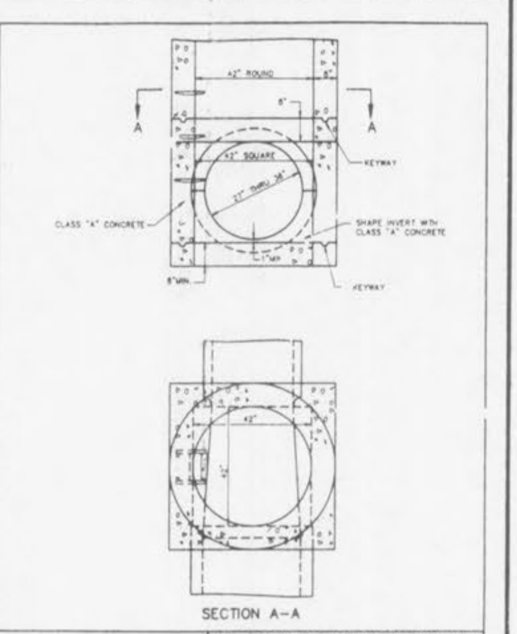
MANHOLE ON PIPE SEWER 27" THRU 36" (ALTERNATE) METROPOLITAN ST. LOUIS SEWER DISTRICT Standard Details of Sewer Construction Dr. D.L.A. Ch. J.C.K. 1992 SHEET 10
