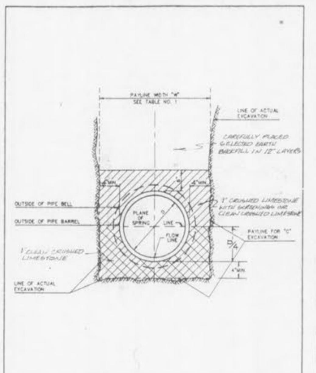
PIPE BEDDING CLASS "C" (FOR ALL PIPE EXCEPT REINFORCED CONCRETE PIPE) METROPOLITAN ST. LOUIS SEWER DISTRICT Standard Details of Sewer Construction Dr. W.S.H. Ch. J.C.K. 1992 SHEET 4
