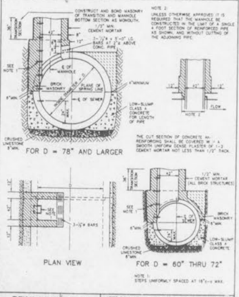
TYPICAL MANHOLE BASE REINFORCED CONCRETE PIPE SEWERS 60" AND LARGER IN DIAMETER METROPOLITAN ST. LOUIS SEWER DISTRICT Standard Details of Sewer Construction Dr. R.G.W. Ch. J.C.K. 1992 SHEET 13
