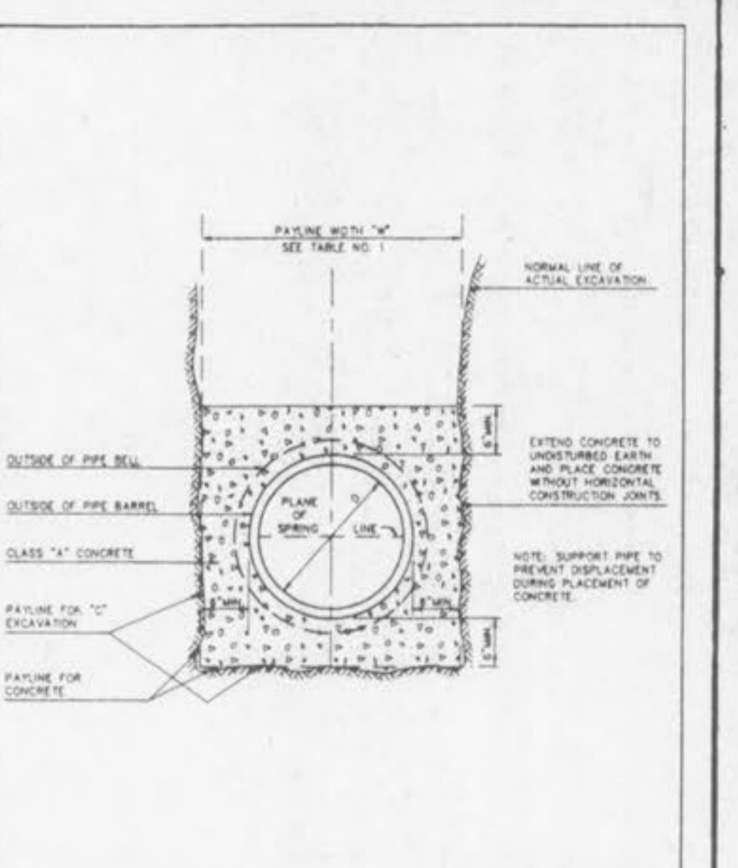
CONCRETE ENCASEMENT METROPOLITAN ST. LOUIS SEWER DISTRICT Standard Details of Sewer Construction Dr. W.S.H. Ch. J.C.K. 1992 SHEET 6
