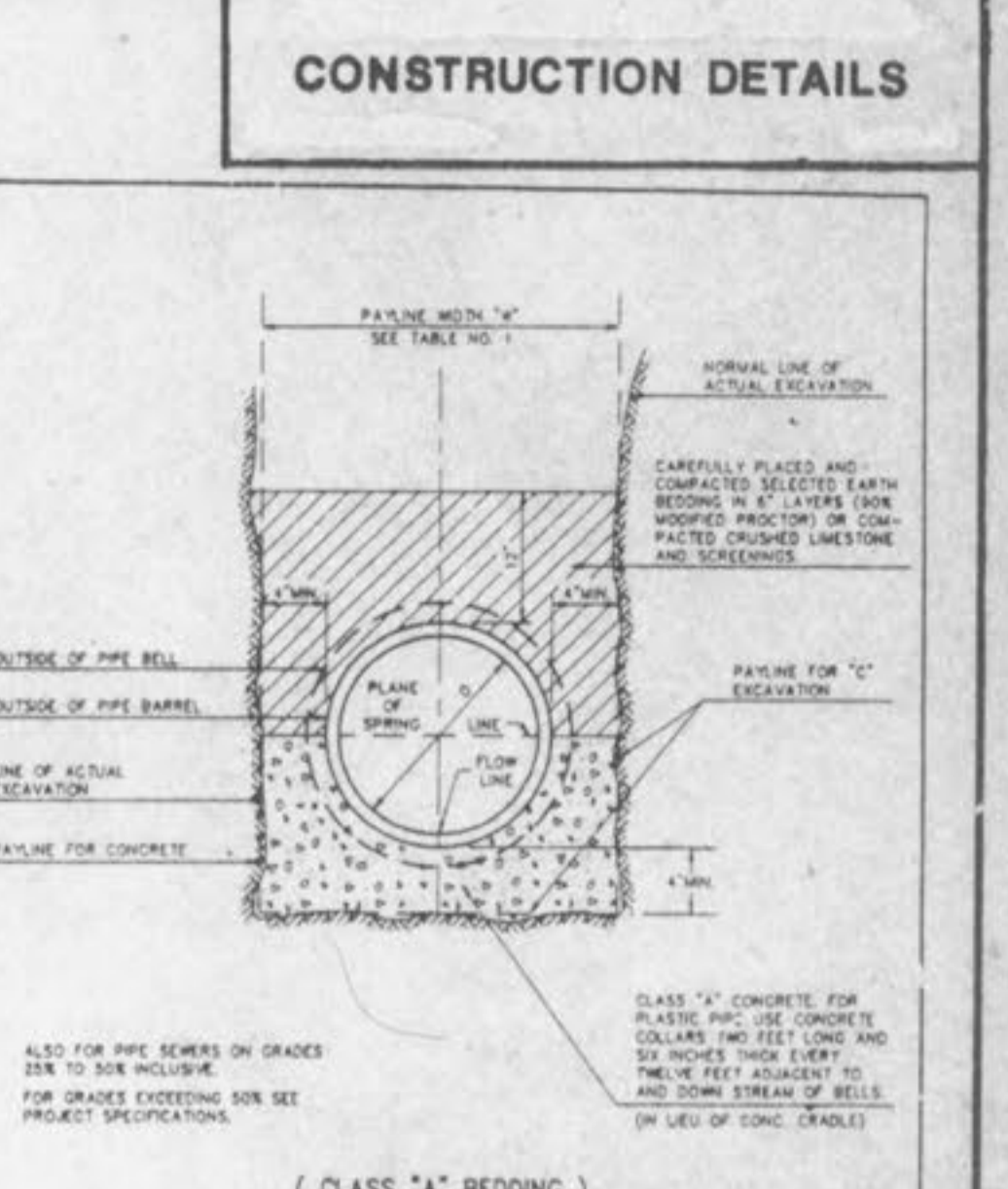
CONCRETE CRADLE METROPOLITAN ST. LOUIS SEWER DISTRICT Standard Details of Sewer Construction Dr. W.S.H. Ch. J.C.K. 1992 SHEET 7
