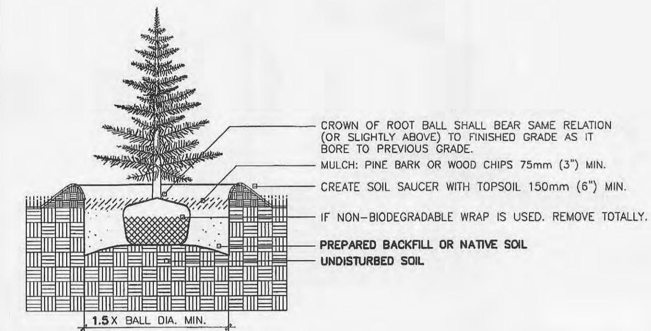
2 CONIFEROUS TREE PLANTING - MEDIUM DUTY
