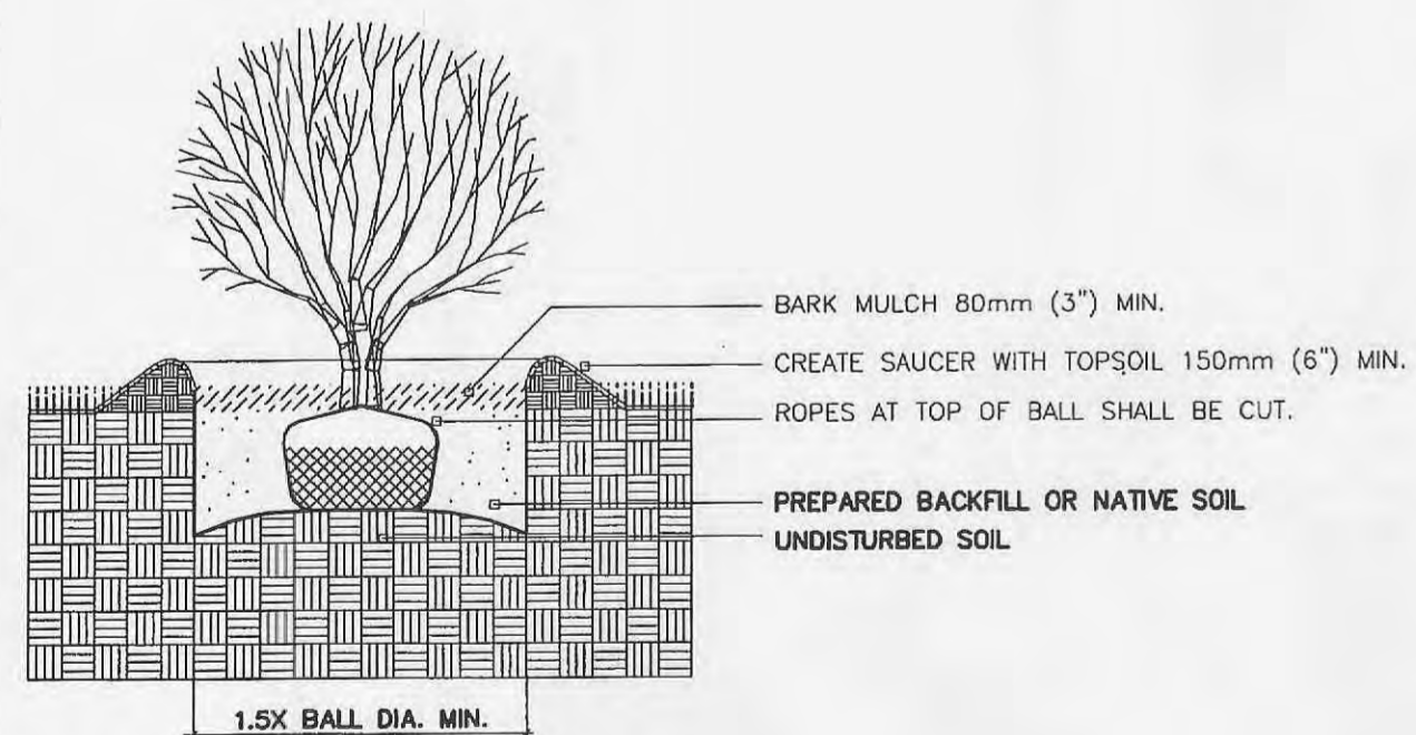
3 SHRUB PLANTING - BALL AND BURLAP
