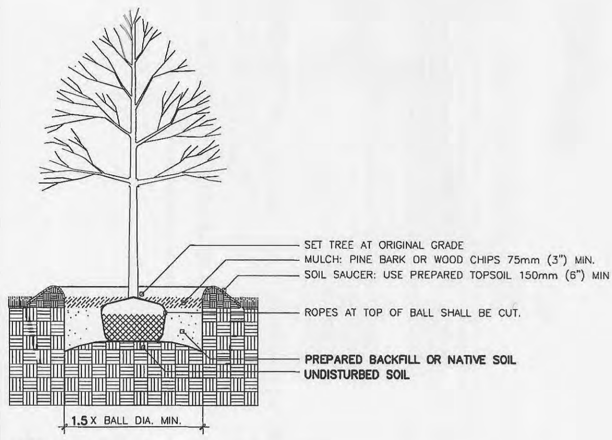
1 DECIDUOUS TREE PLANTING
