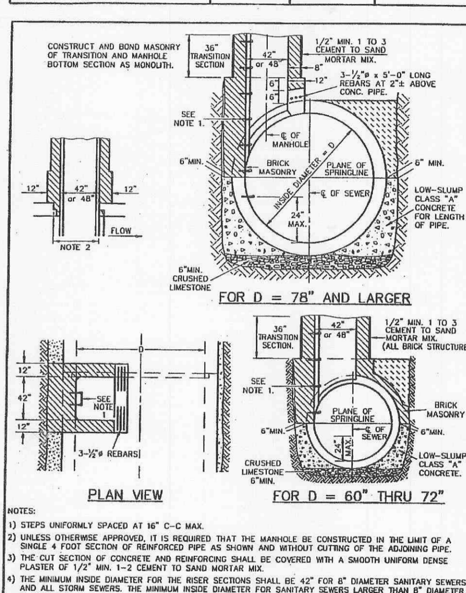
TYPICAL MANHOLE BASE REINFORCED CONCRETE PIPE SEWERS 60" AND LARGER IN DIAMETER METROPOLITAN ST. LOUIS SEWER DISTRICT Standard Details of Sewer Construction Dr. W.S.H./SAM 2000 SHEET 15 Ch. J.C.K.
