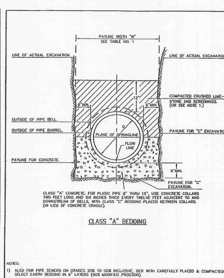
CONCRETE CRADLE METROPOLITAN ST. LOUIS SEWER DISTRICT Standard Details of Sewer Construction Dr. W.S.H./SAM 2000 SHEET 9 Ch. J.C.K.
