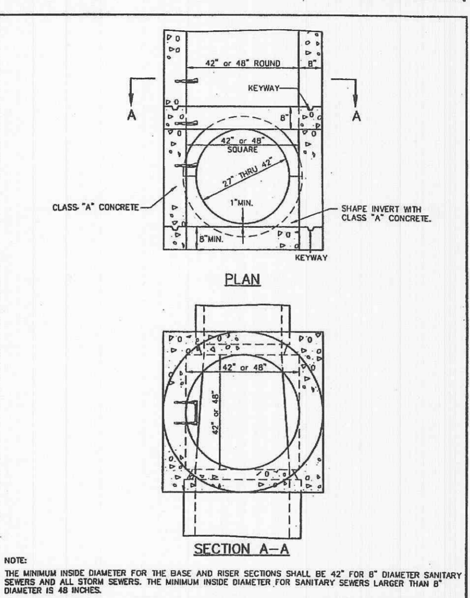
MANHOLE ON PIPE SEWER 27" THRU 42" (ALTERNATE) METROPOLITAN ST. LOUIS SEWER DISTRICT Standard Details of Sewer Construction Dr. D.A.B./SAM 2000 SHEET 12 Ch. J.C.K.
