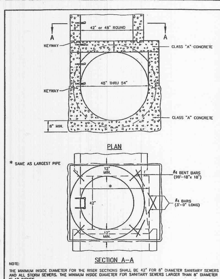
MANHOLE ON CONG. PIPE 48" THRU 54" (ALTERNATE) METROPOLITAN ST. LOUIS SEWER DISTRICT Standard Details of Sewer Construction Dr. W.S.H./SAM 2000 SHEET 14 Ch. J.C.K.
