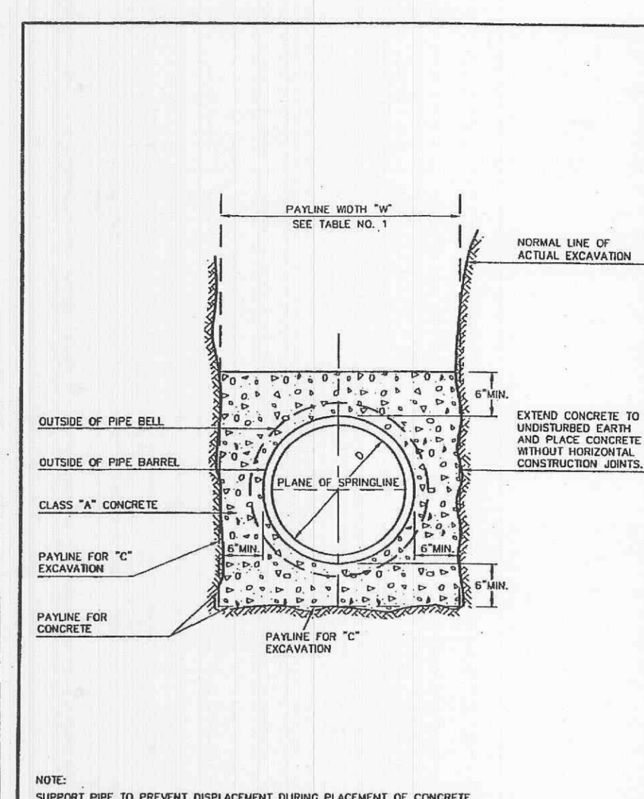
CONCRETE ENCASUREMENT METROPOLITAN ST. LOUIS SEWER DISTRICT Standard Details of Sewer Construction Dr. W.S.H. 2000 SHEET 8 Ch. J.C.K.
