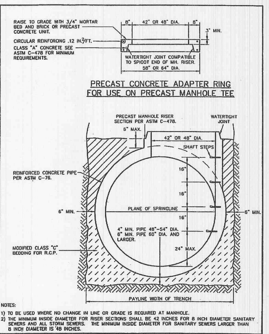
TYPICAL PRECAST MANHOLE TEE FOR REINFORCED CONCRETE PIPE SEWERS 48 INCH AND LARGER IN DIAMETER METROPOLITAN ST. LOUIS SEWER DISTRICT Standard Details of Sewer Construction Dr. W.S.H./SAM 2000 SHEET 24 Ch. J.C.K.
