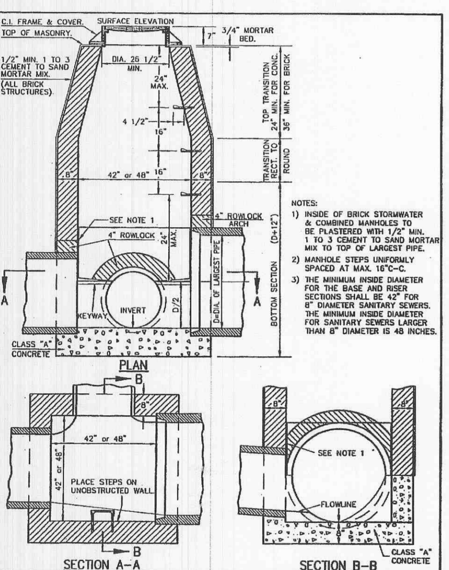
TYPICAL LINE MANHOLE ON PIPE SEWER 27" THRU 42" IN DIAMETER METROPOLITAN ST. LOUIS SEWER DISTRICT Standard Details of Sewer Construction Dr. W.S.H./SAM 2000 SHEET 11 Ch. J.C.K.
