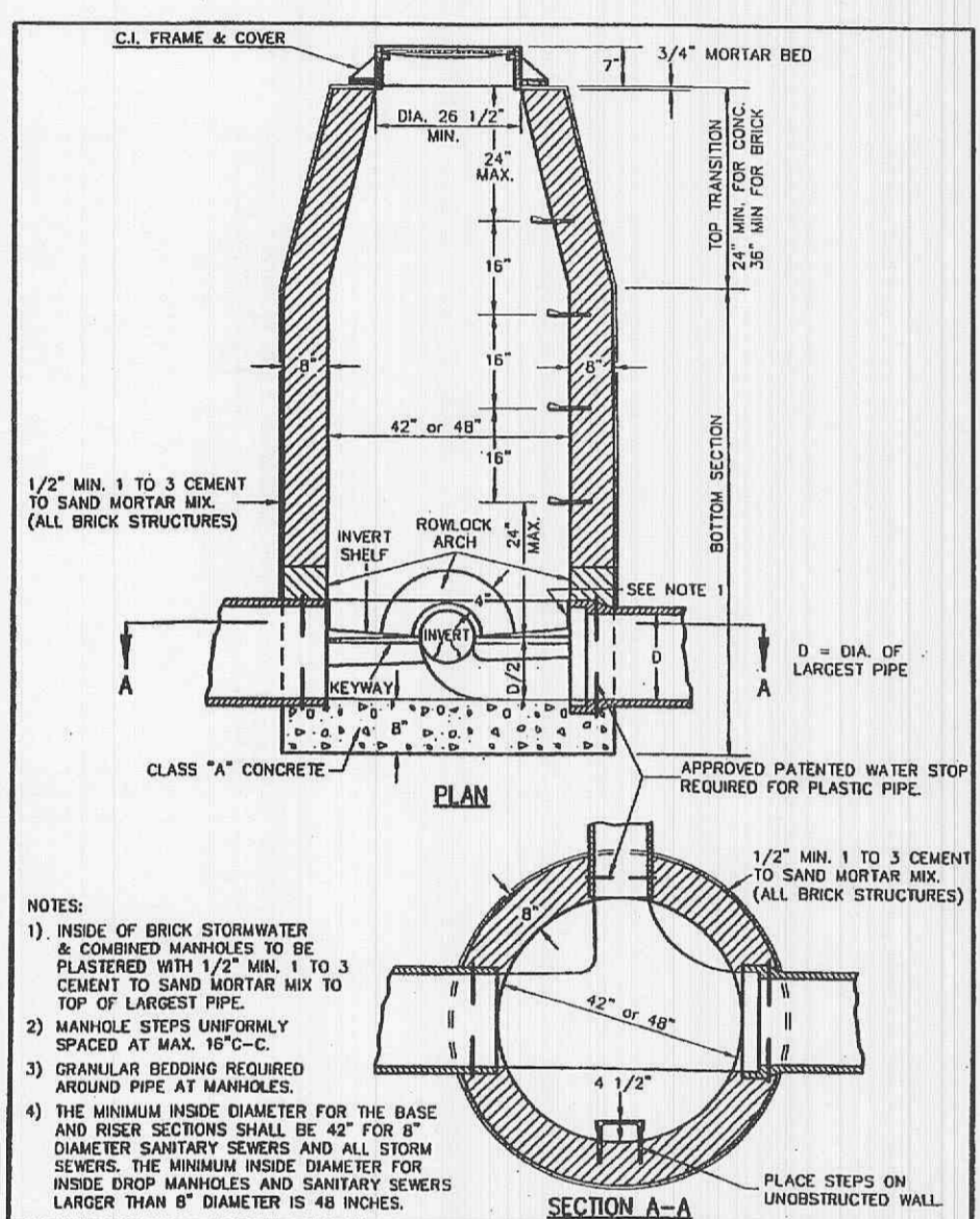
LINE MANHOLE ON PIPE SEWERS 8"-24" DIA. METROPOLITAN ST. LOUIS SEWER DISTRICT Standard Details of Sewer Construction Dr. W.S.H./SAM 2000 SHEET 10 Ch. J.C.K.
