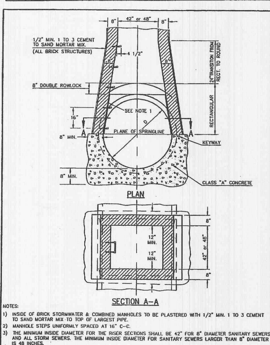
MANHOLE ON CONCRETE PIPE SEWERS 48" THRU 54" DIAMETER METROPOLITAN ST. LOUIS SEWER DISTRICT Standard Details of Sewer Construction Dr. W.S.H./SAM 2000 SHEET 13 Ch. J.C.K.
