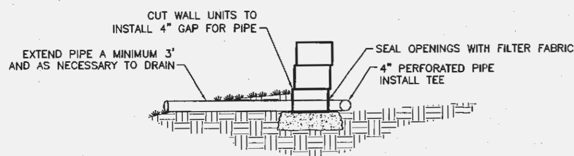
PERFORATED PIPE OUTLET NOT TO SCALE
