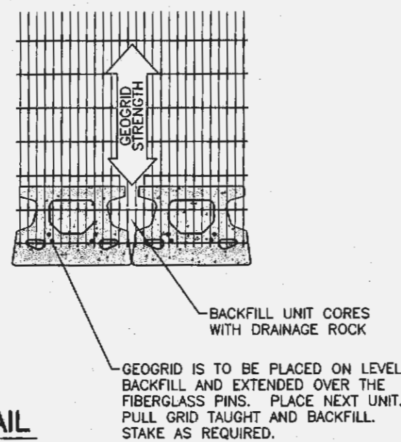
COMPAC II UNIT NOT TO SCALE
