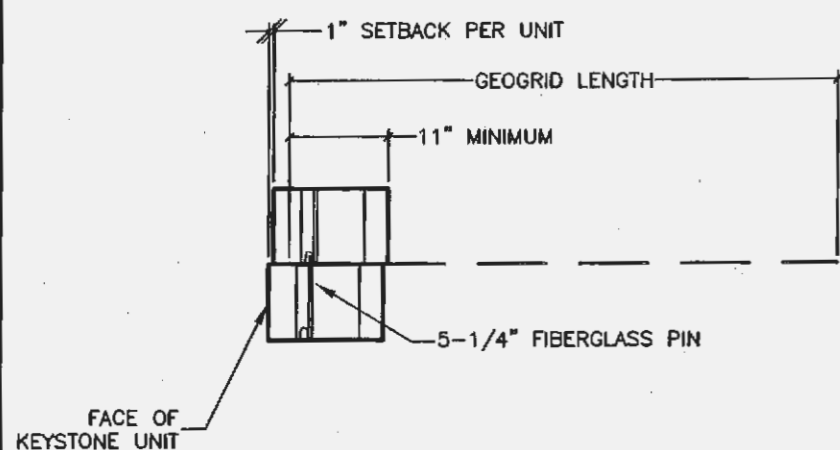
CONNECTION DETAIL NOT TO SCALE
