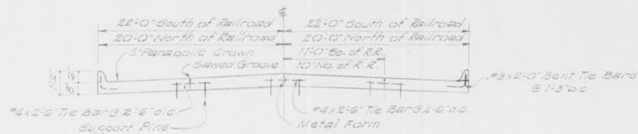
TYPICAL STREET SECTION P.C. CONCRETE PAVEMENT From Sta. 18+41 to Sta. 14+66 & From Sta. 15+02 to Sta. 15+02
