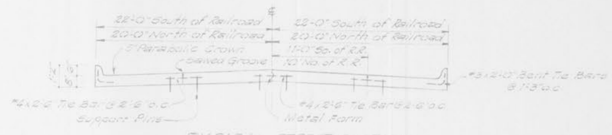
TYPICAL STREET SECTION R.C. CONCRETE PAVEMENT From Sta. 18+41 to Sta. 14+00 & From Sta. 16+02 to Sta. 15+02
