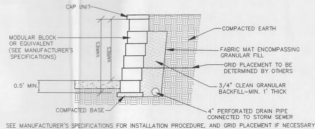
MODULAR BLOCK CONCRETE RETAINING WALL (NO DESIGN REQUIRED HEIGHT OF WALL IS MINIMAL) NOT TO SCALE
