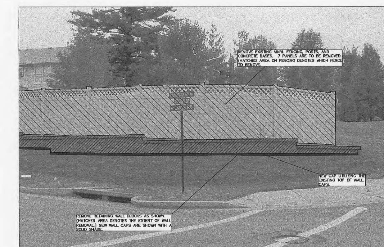
DETAIL SHOWING WALL MODIFICATIONS SCALE: NTS
