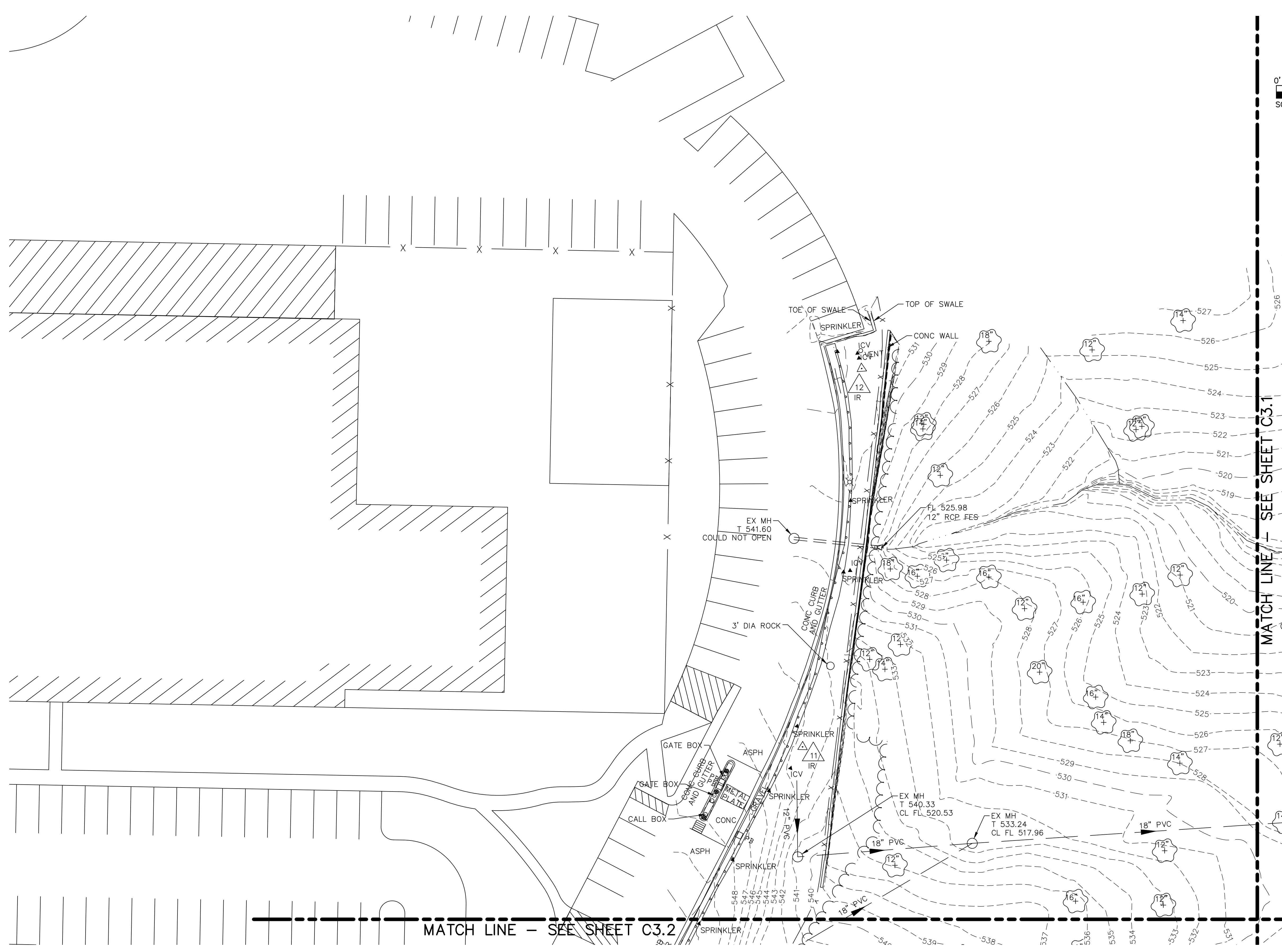
1 EXISTING CONDITIONS PLAN - AREA 1 C3.0
