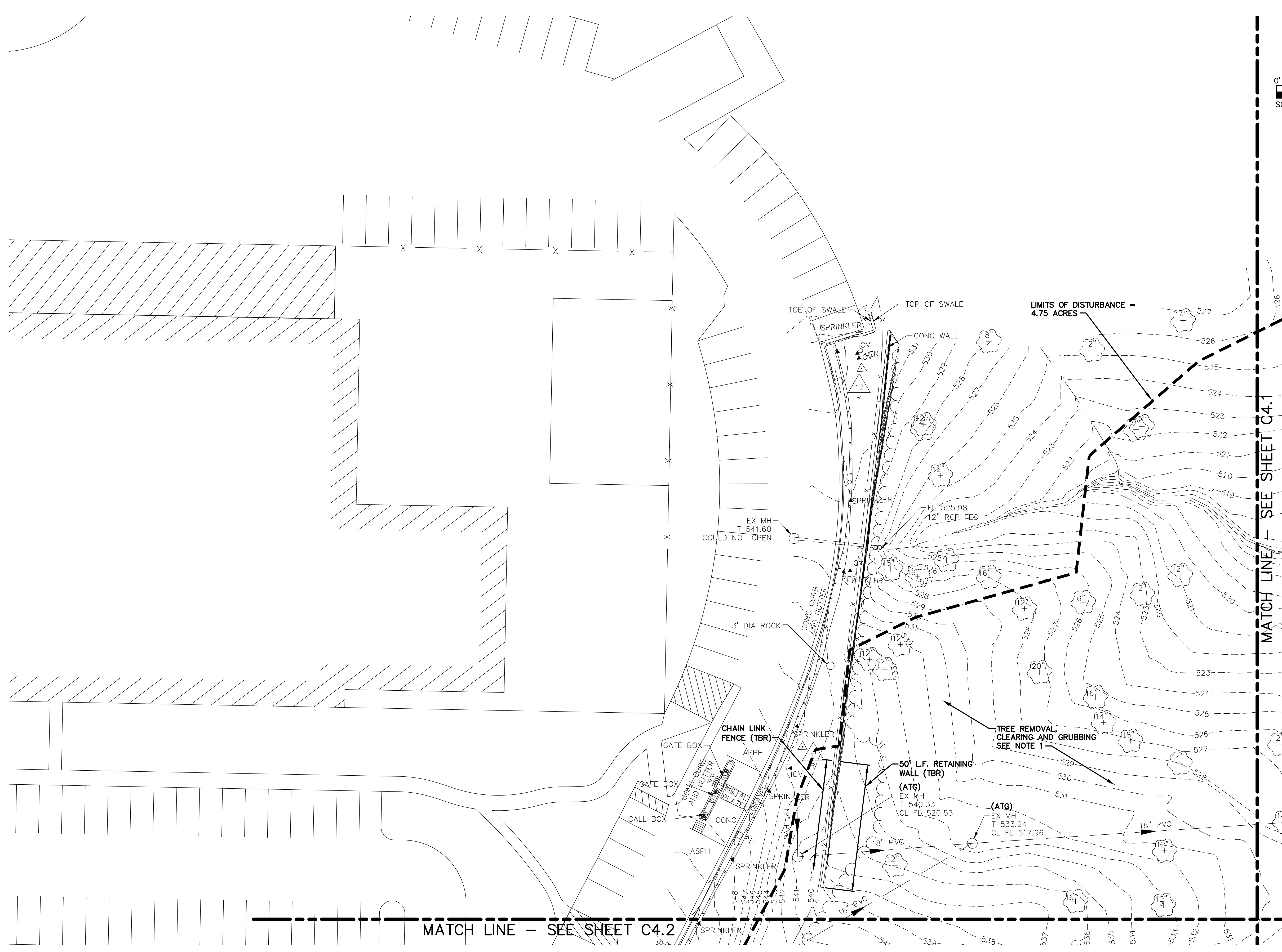
1 SITE DEMOLITION PLAN - AREA 1 C4.0
