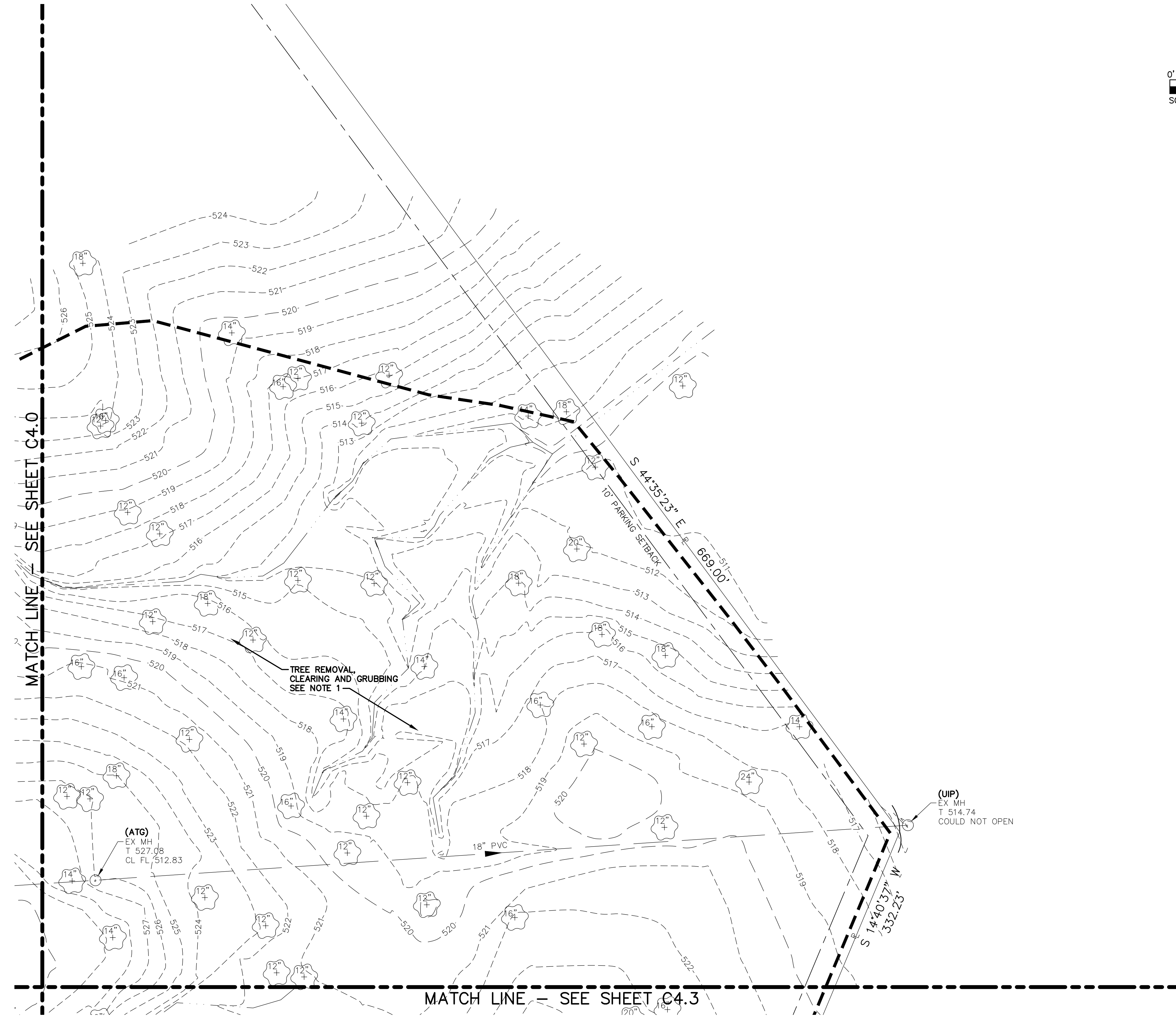
1 SITE DEMOLITION PLAN - AREA 2
