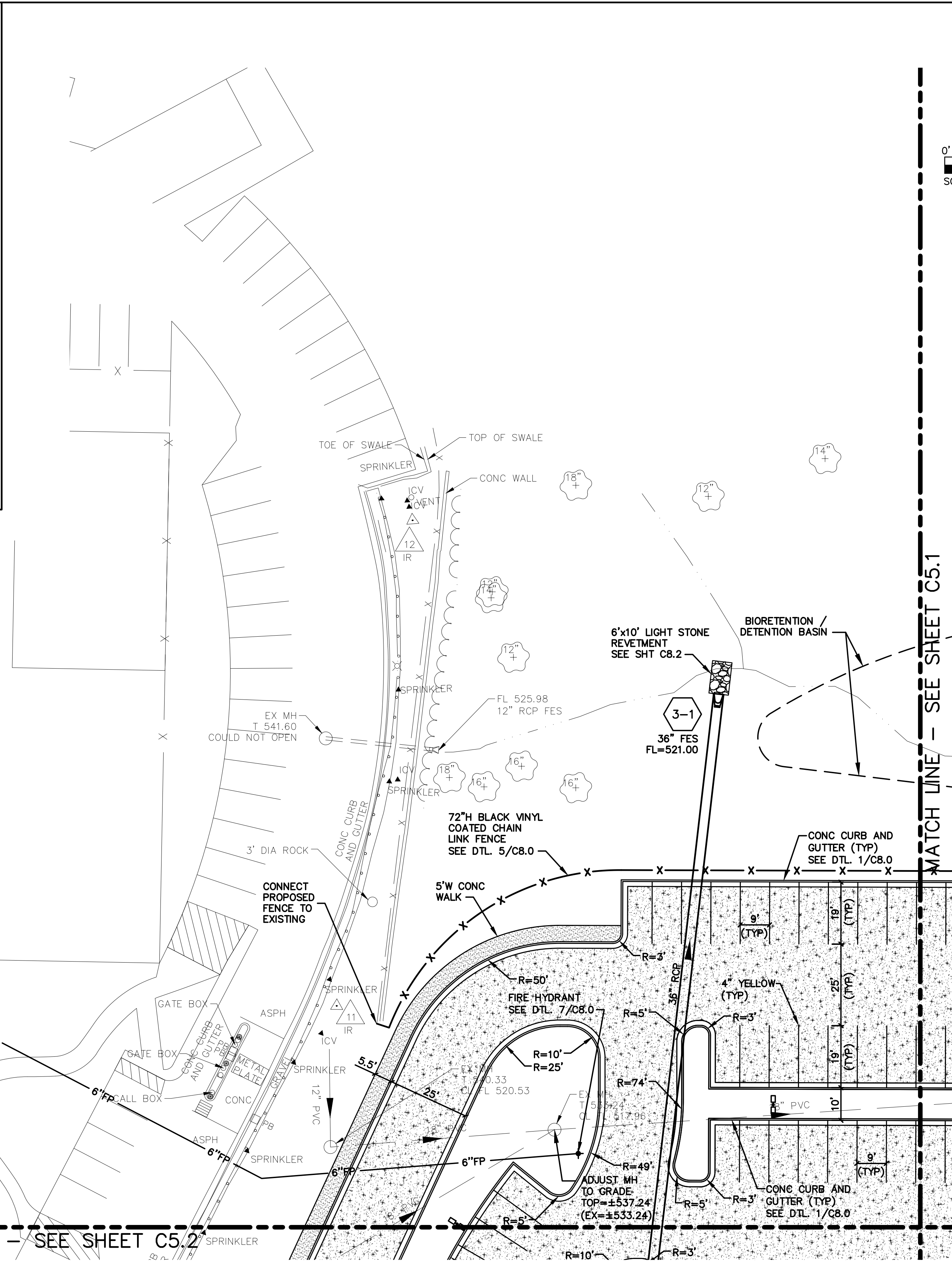
1 SITE IMPROVEMENT PLAN - AREA 1 C5.0
