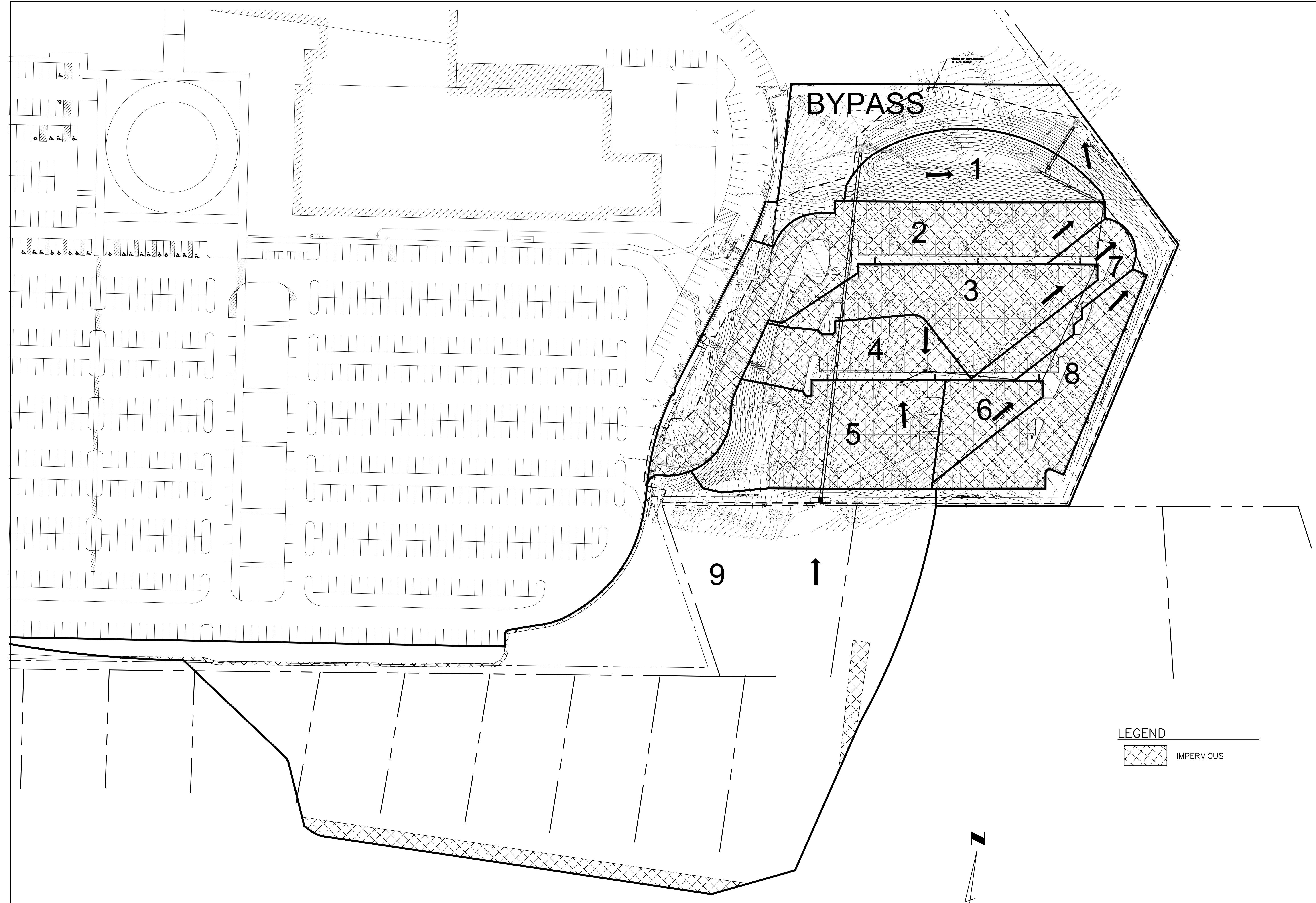
POST DEVELOPMENT - DRAINAGE AREA MAP FOR STORM SEWER CALCULATIONS
