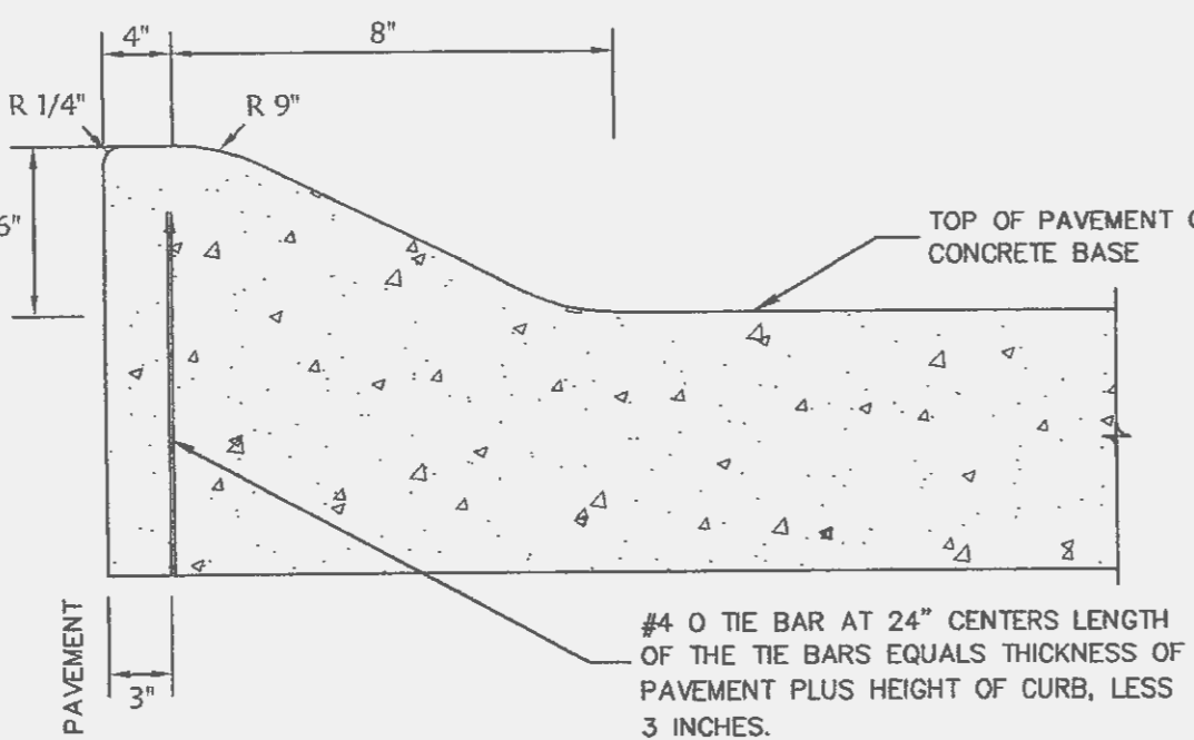
7 "TYPE M" MOUNTABLE CURB Not To Scale
