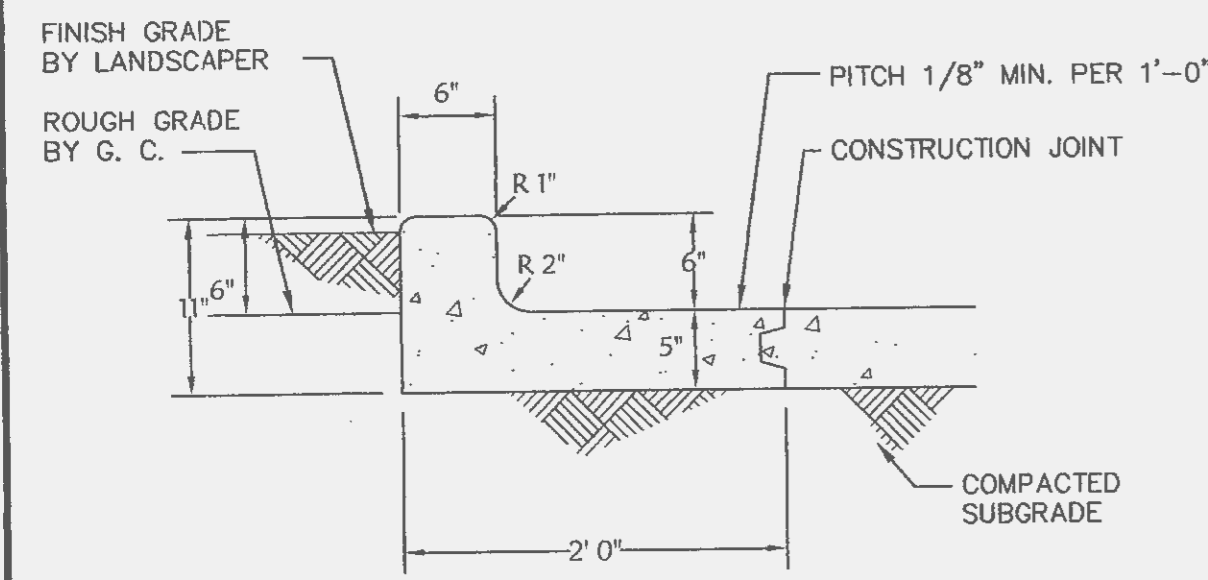
6 INTEGRAL CURB FOR CONC. LOTS Not To Scale
