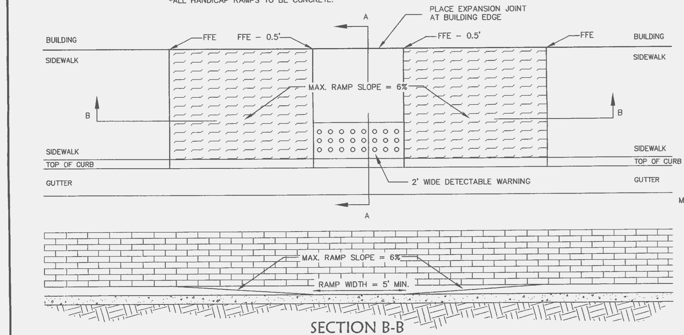
12 SIDEWALK WITH RAMP CONDITIONS Not To Scale
