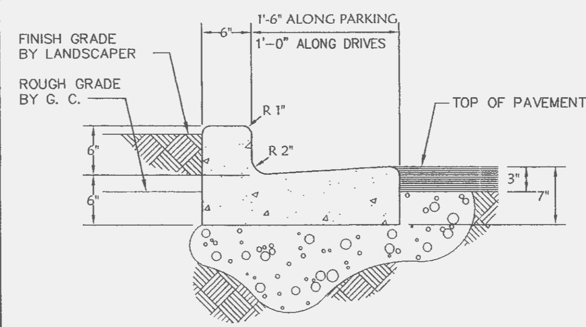
4 CONCRETE CURB & GUTTER Not To Scale
