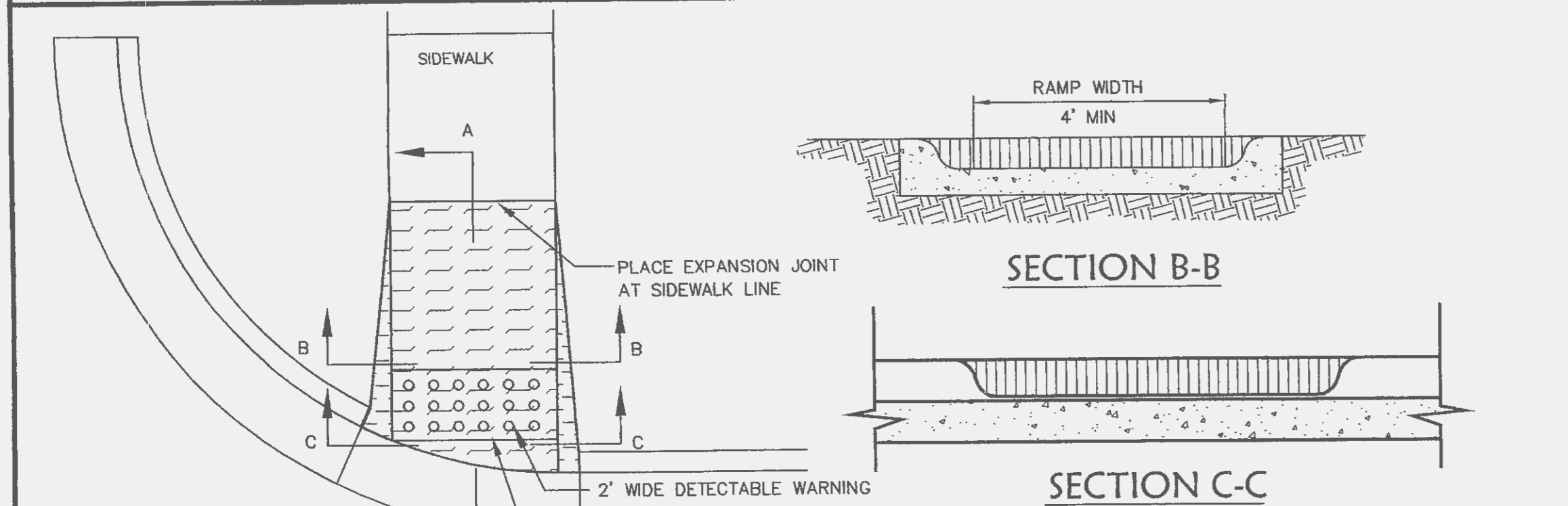
11 SIDEWALK WITH RAMP CONDITIONS Not To Scale
