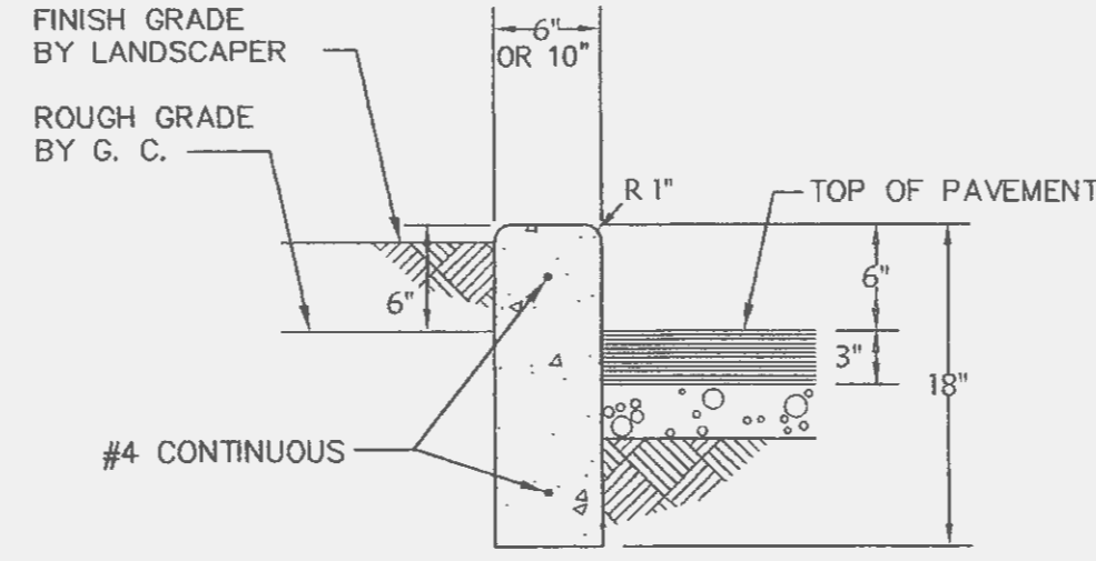
3 CONC. CURB - 6" X 18" & 10" X 18" Not To Scale
