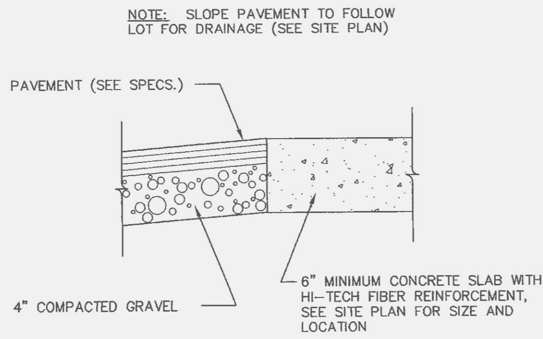
2 DRIVE-THRU PAD DETAIL Not To Scale
