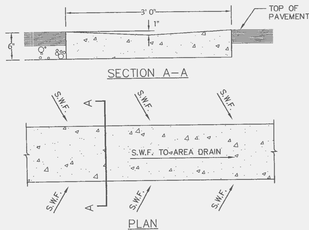
1 CONCRETE SWALE Not To Scale
