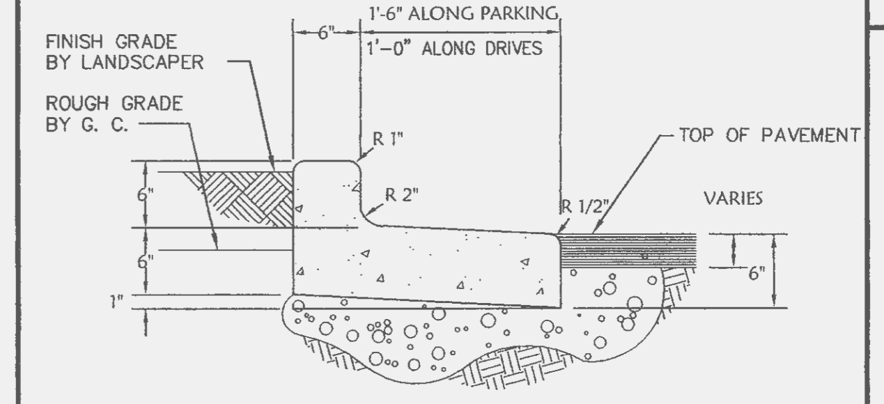
10 DRY CONCRETE CURB & GUTTER Not To Scale
