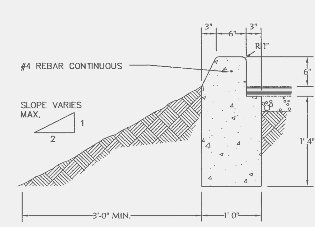
5 CURB AT TOP OF SLOPE Not To Scale
