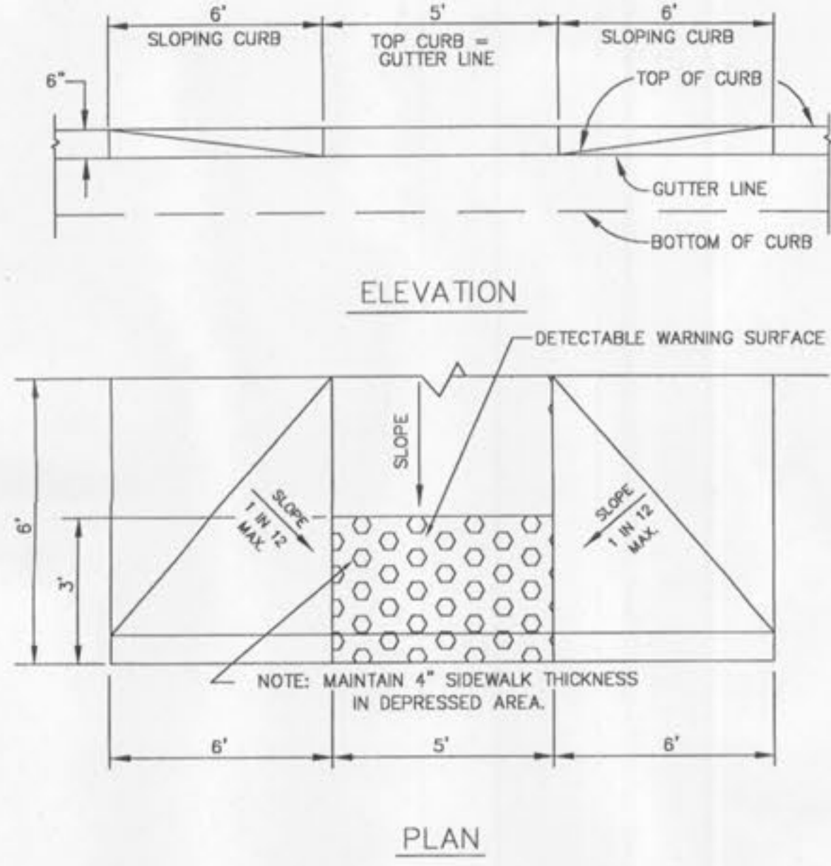
5 HANDICAP RAMP DETAIL-TYPE 3 SCALE: N.T.S. REF. DWG. C3.0
