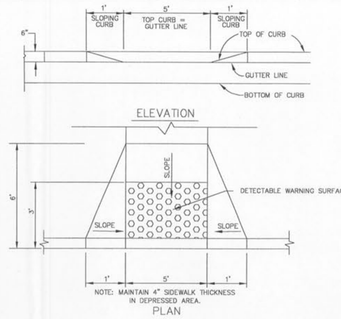
3 HANDICAP RAMP DETAIL-TYPE 1 SCALE: N.T.S. REF. DWG. C3.0
