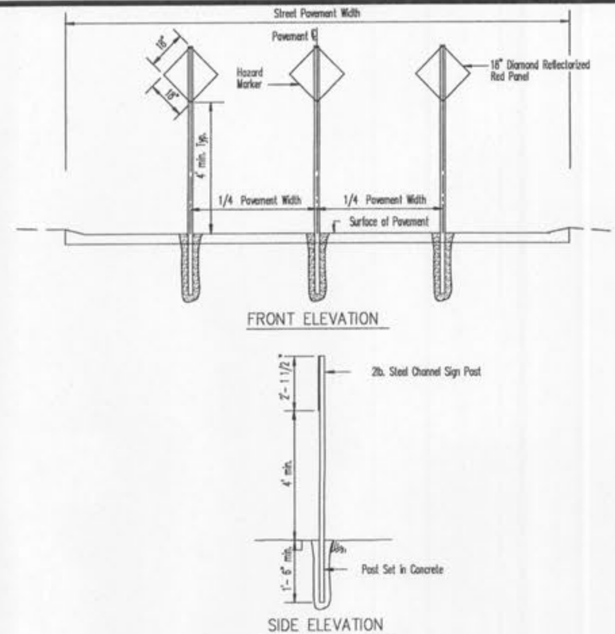
11 SIGN DETAIL FOR TERMINATION OF ROAD PAVEMENT SCALE: N.T.S. REF. DWG. C3.0
