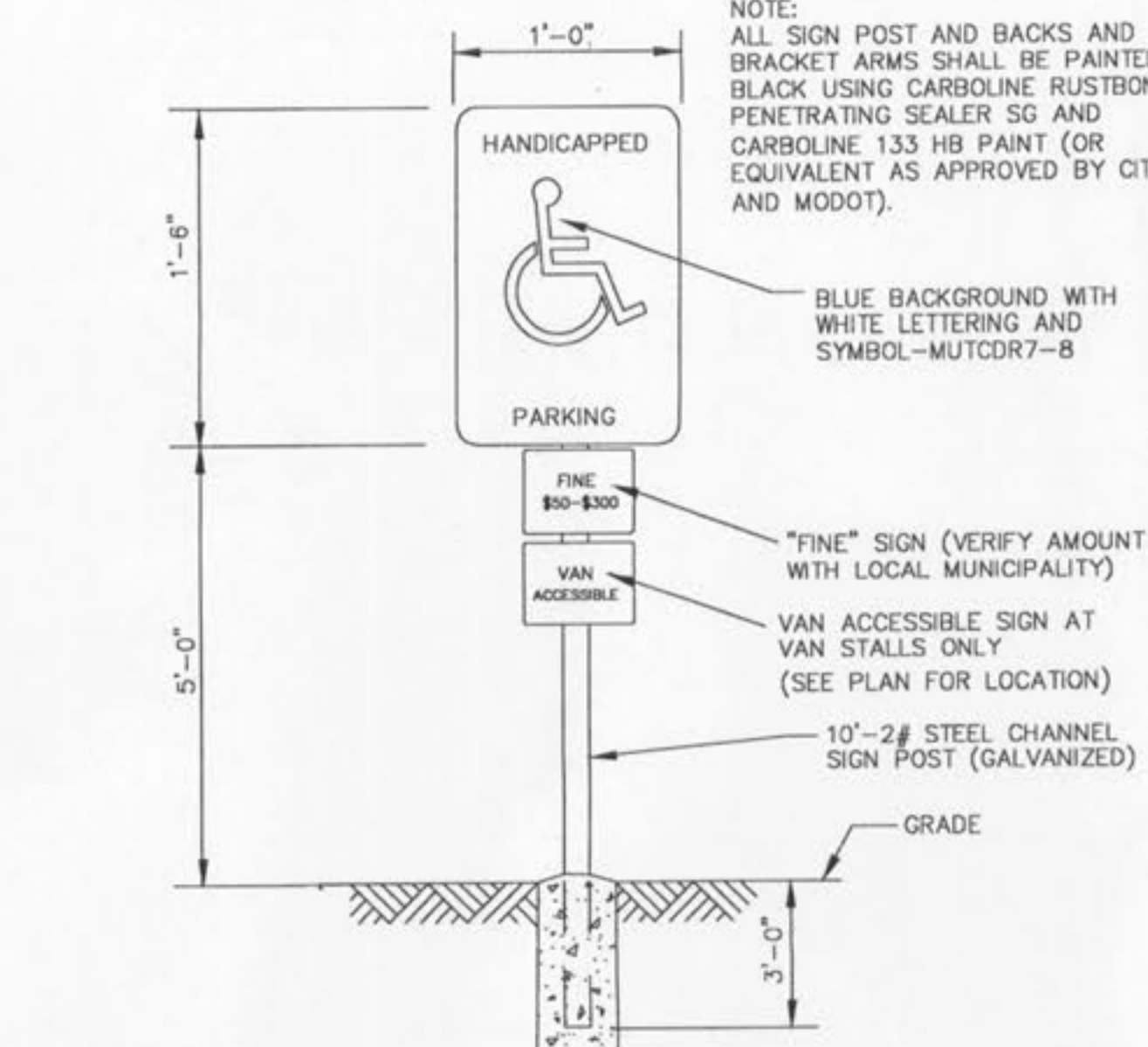
9 HANDICAP SIGN DETAIL SCALE: N.T.S. REF. DWG. C3.0
