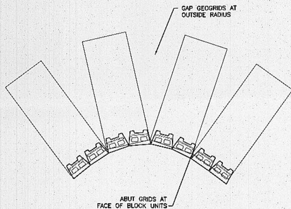
INSIDE RADIUS NOT TO SCALE
