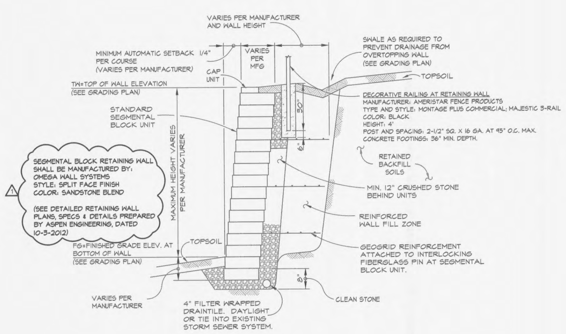
SEGMENTAL UNIT RETAINING WALL N.T.S.
