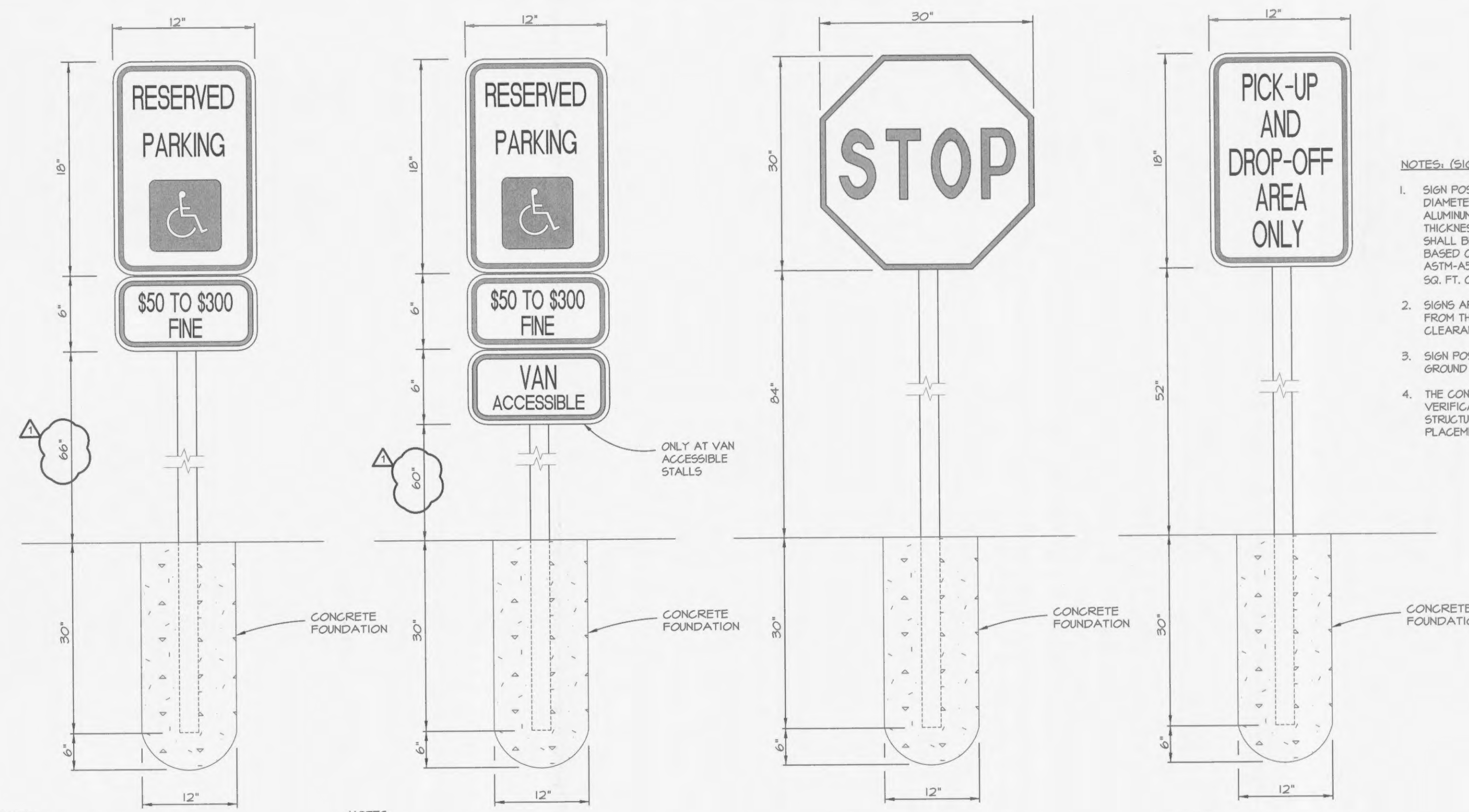
HANDICAPPED SIGN DETAIL (R7-8) N.T.S.
