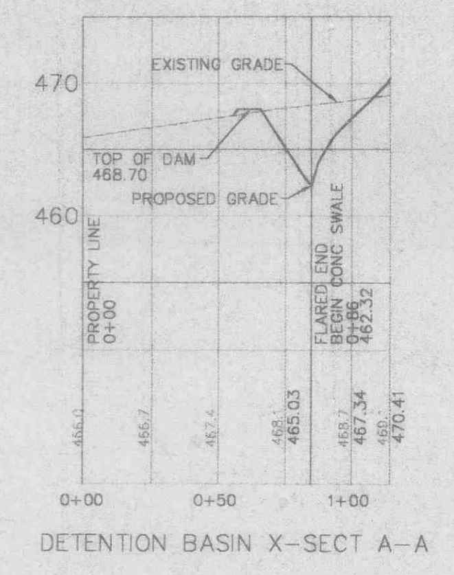
DETENTION BASIN CROSS SECTIONS HORIZONTAL SCALE: 1"=50' VERTICAL SCALE: 1"=10'
