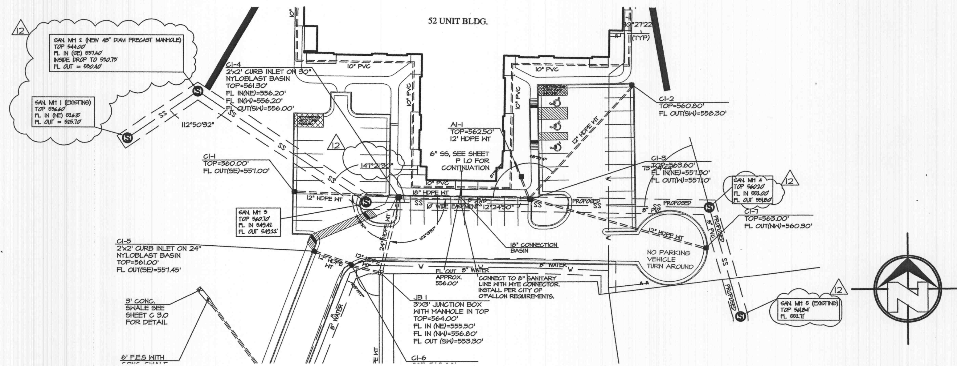
1 SANITARY SEWER PLAN HORIZONTAL SCALE: 1" = 40'
