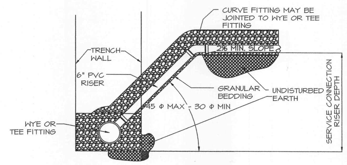
SANITARY SEWER CONNECTION DETAIL SCALE: 1" = 40'
