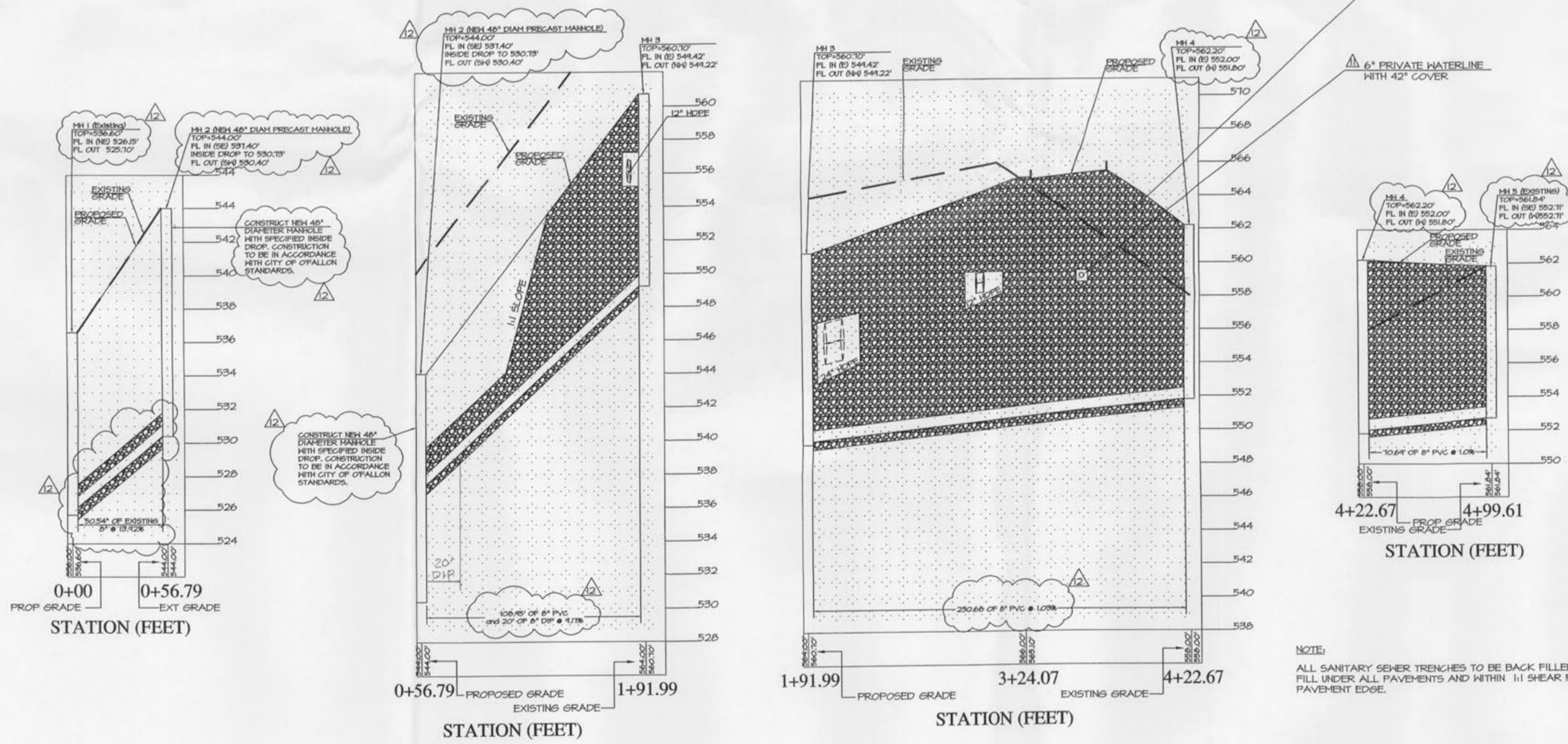
2 SANITARY SEWER PROFILE HORIZONTAL SCALE: 1" = 40' VERTICAL SCALE: 0.25" = 1'
