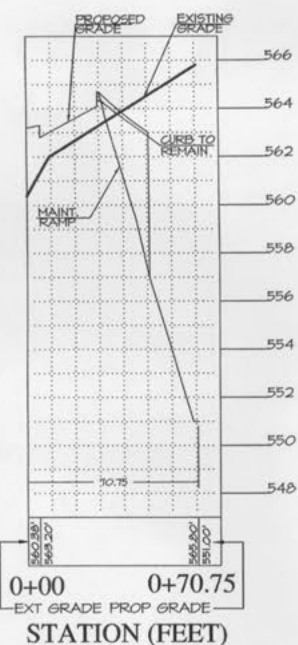
DETENTION BASIN 8' WIDE MAINT. ACCESS RAMP PROFILE HORIZONTAL SCALE: 1" = 40' VERTICAL SCALE: 0.25" = 1'
