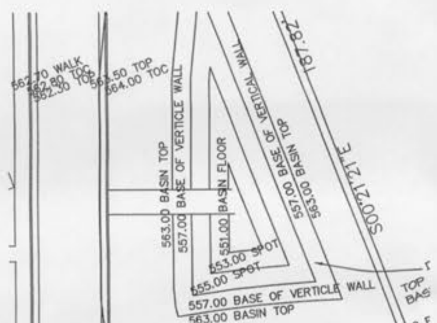
DETENTION BASIN 8' WIDE MAINT. ACCESS RAMP PLAN HORIZONTAL SCALE: 1" = 40'
