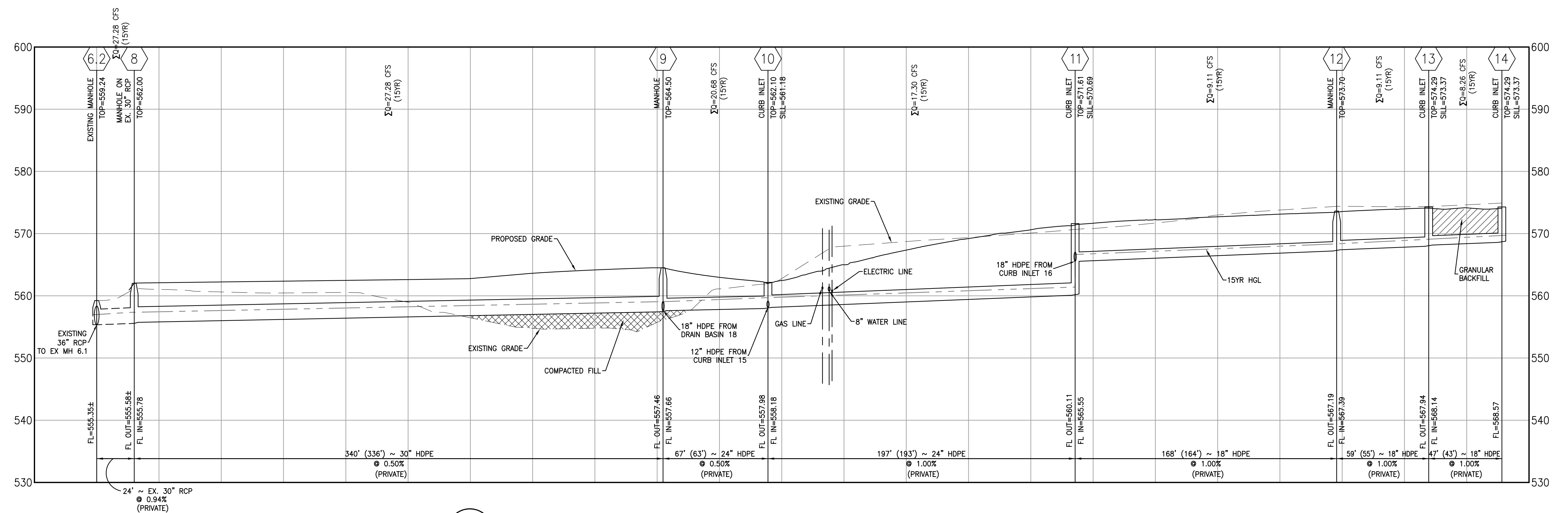
1 STORM SEWER PROFILES SCALE: 1"=40' HORIZ. 1"=10' VERT. REF. DWG. C7.1
