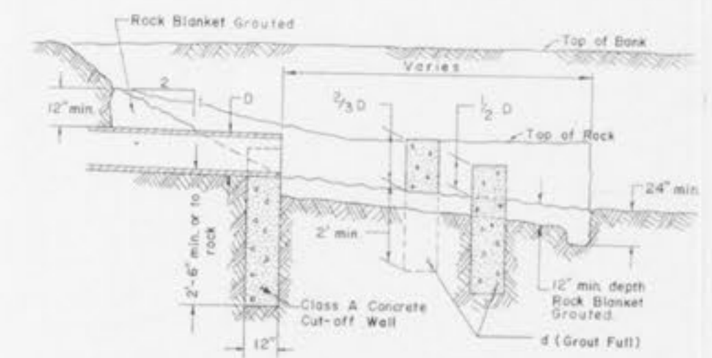
SECTION A-A D = Diameter d = Half Dia End of Pipe with Energy Dissipator FOR 12" - 24" CULVERTS
