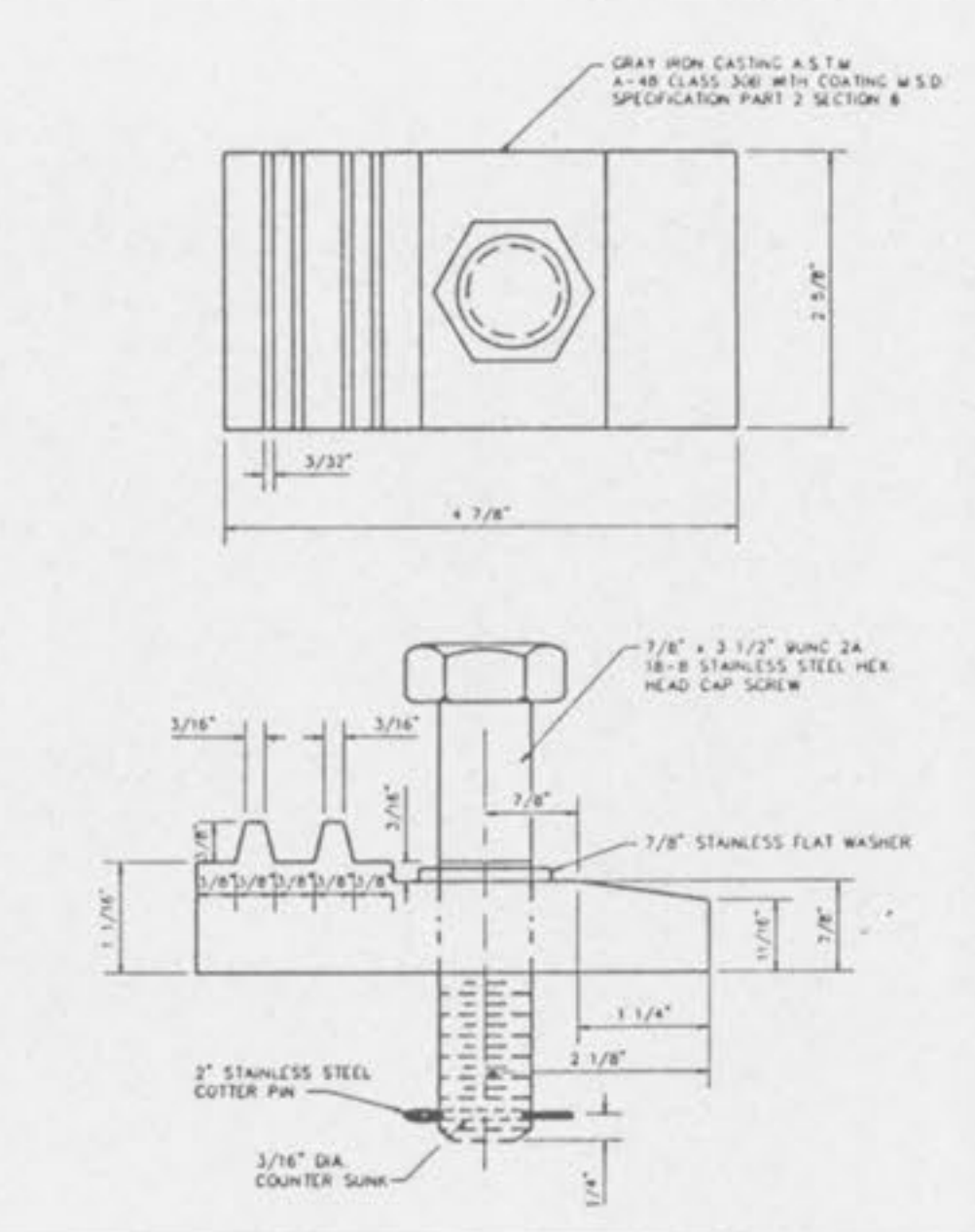
LOCKING DEVICE FOR TYPE 'I' LOCK TYPE MANHOLE COVER METROPOLITAN ST. LOUIS SEWER DISTRICT Standard Details of Sewer Construction Dr. W.S.H. Ch. J.C.K. 1992 SHEET 51
