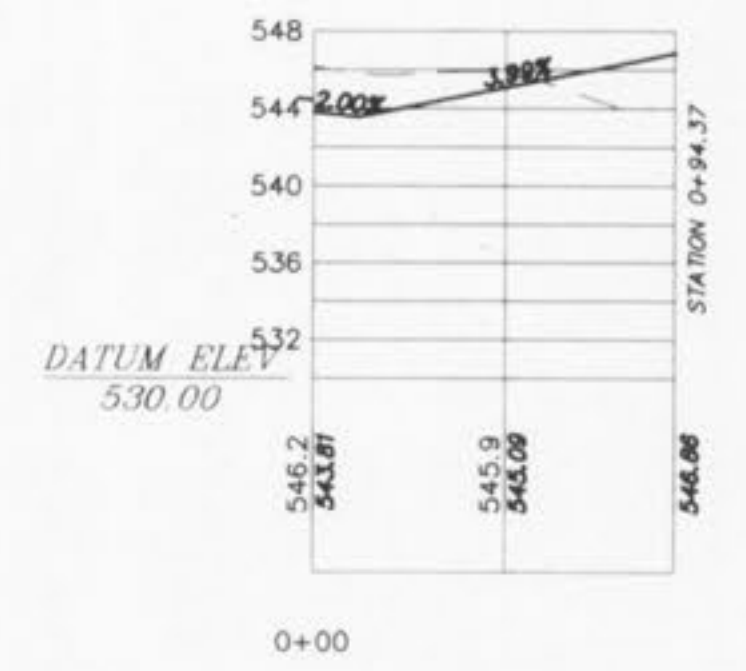
CARTER'S GROVE 'EYEBROW COURT' (STA. 6+22.11)
