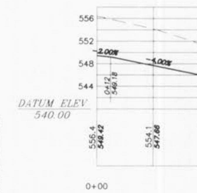
CARTER'S GROVE 'EYEBROW COURT' (STA. 3+72.00)
