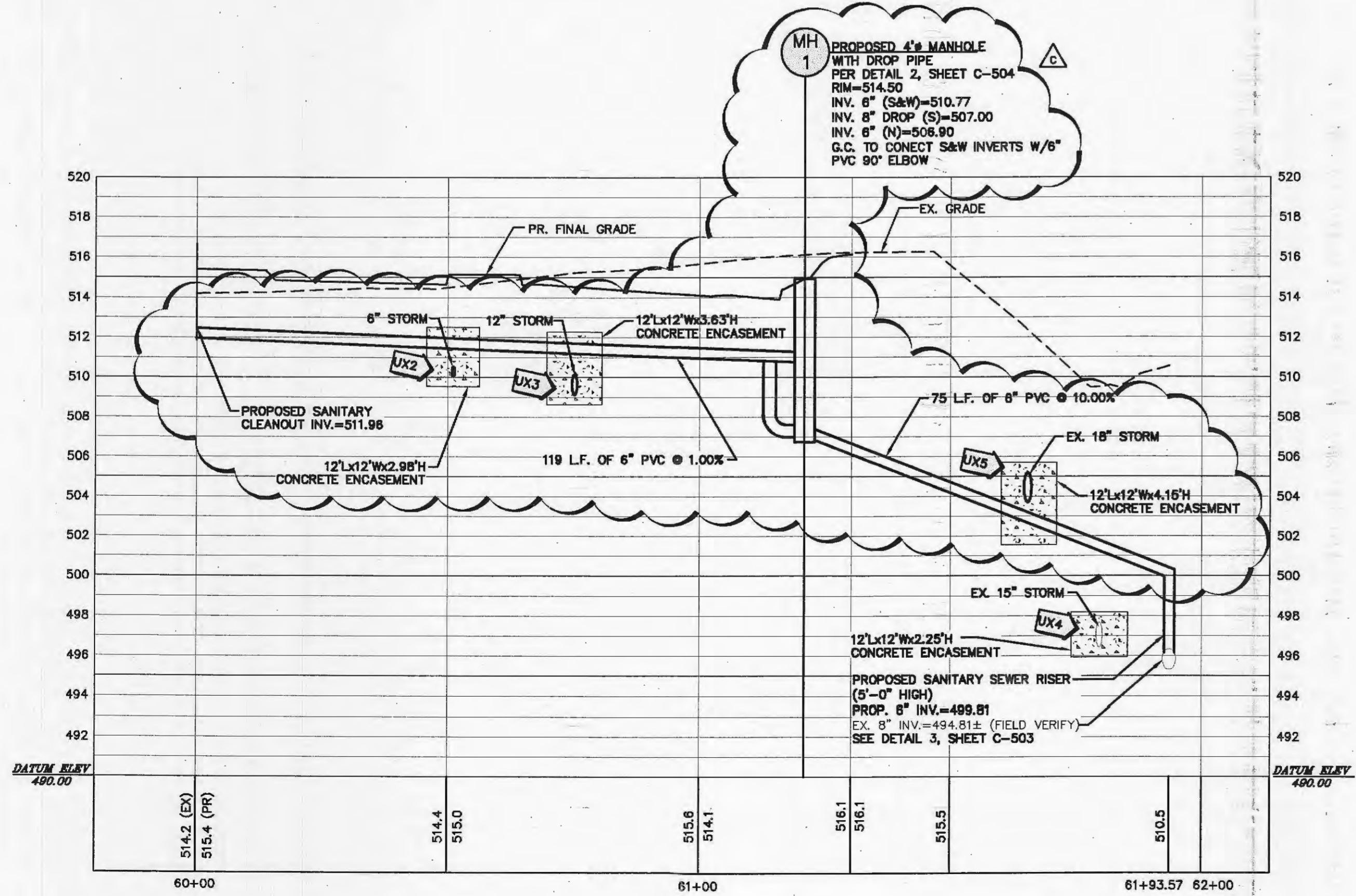
SANITARY SEWER PROFILE HOR.: 1"=20' VERT.: 1"=5'
