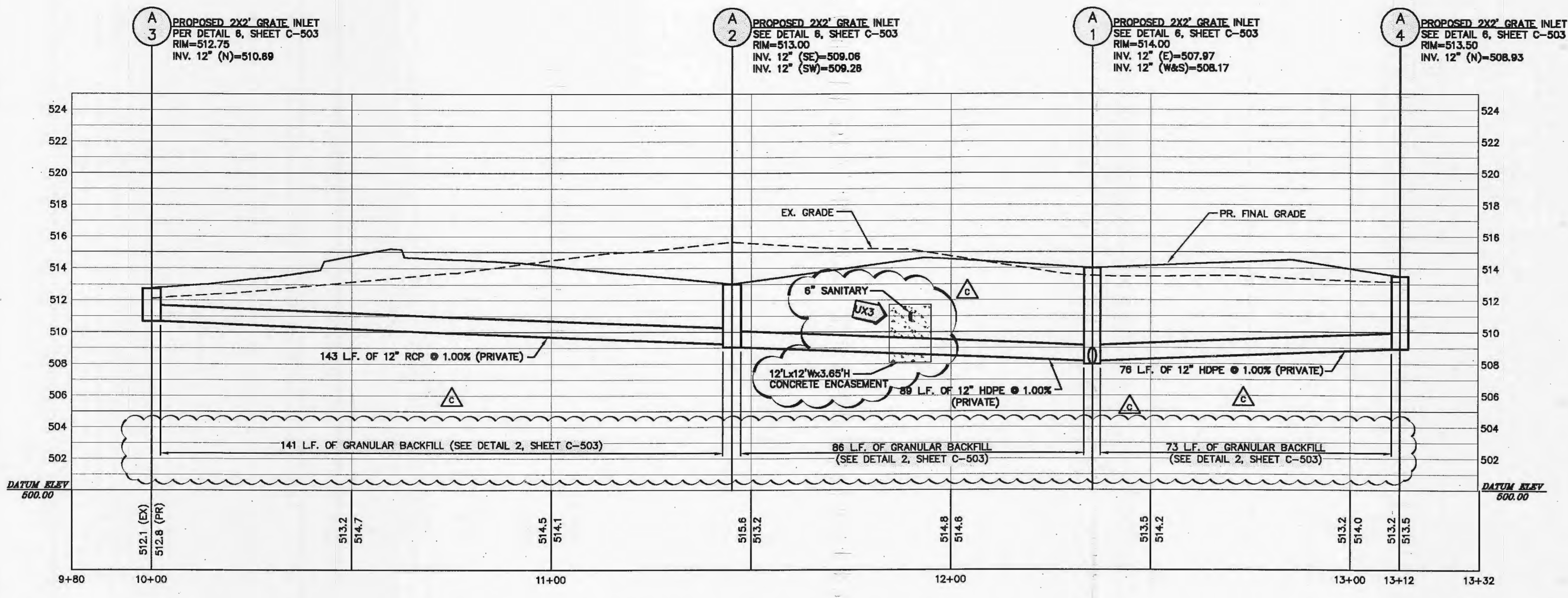
STORM SEWER PROFILE STRUCTURES A1-A4 HOR.: 1"=20' VERT.: 1"=5'
