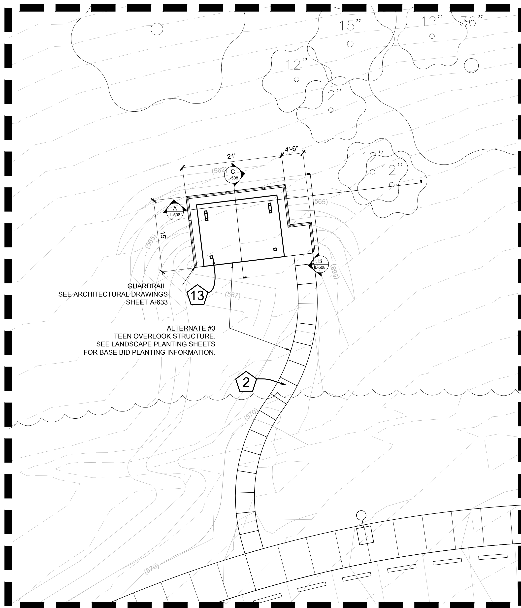
C TEEN OVERLOOK SHELTER ENLARGEMENT PLAN SCALE: 1"=10'
