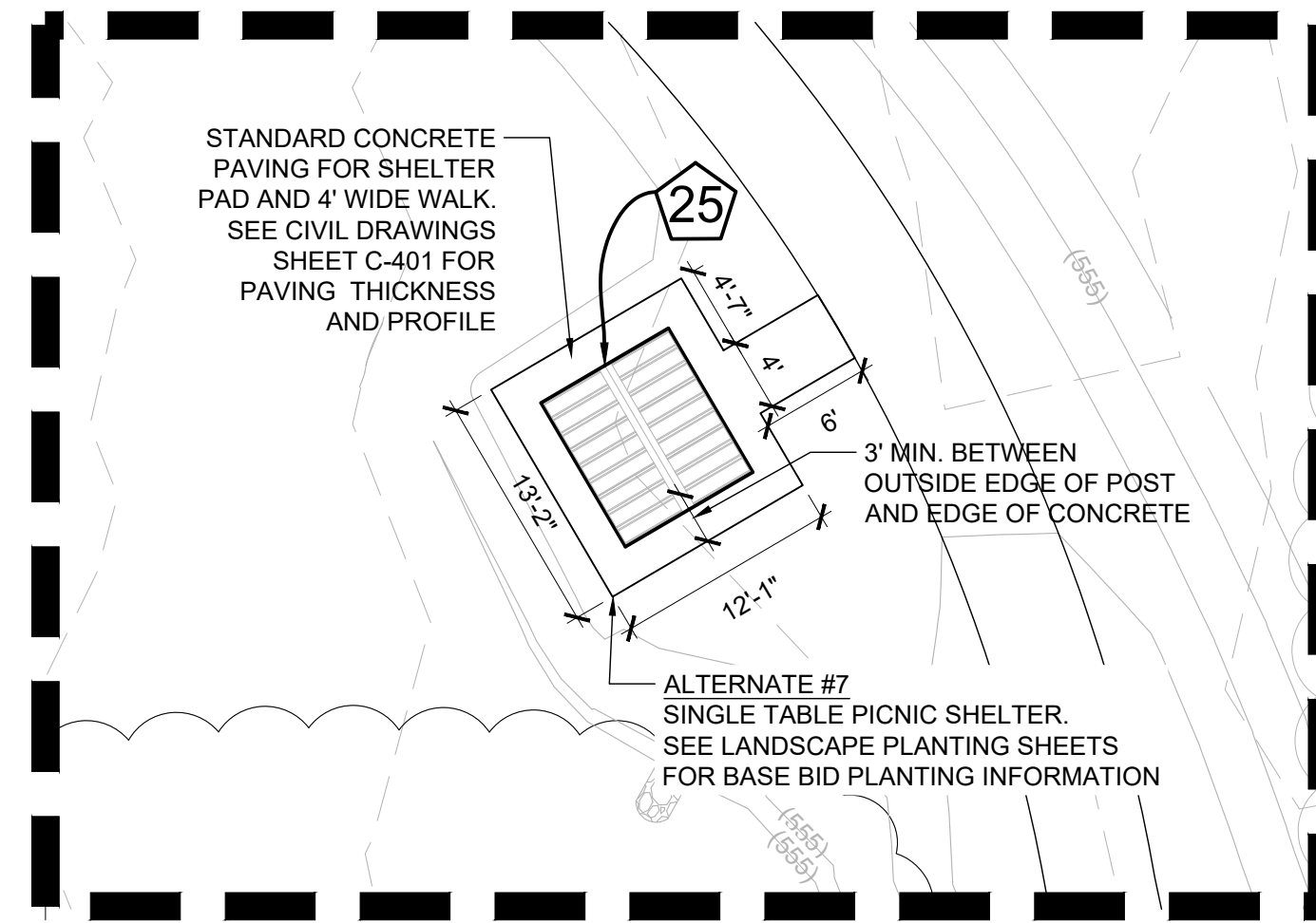
B TYPICAL PICNIC SHELTER LAYOUT SCALE: 1"=10'
