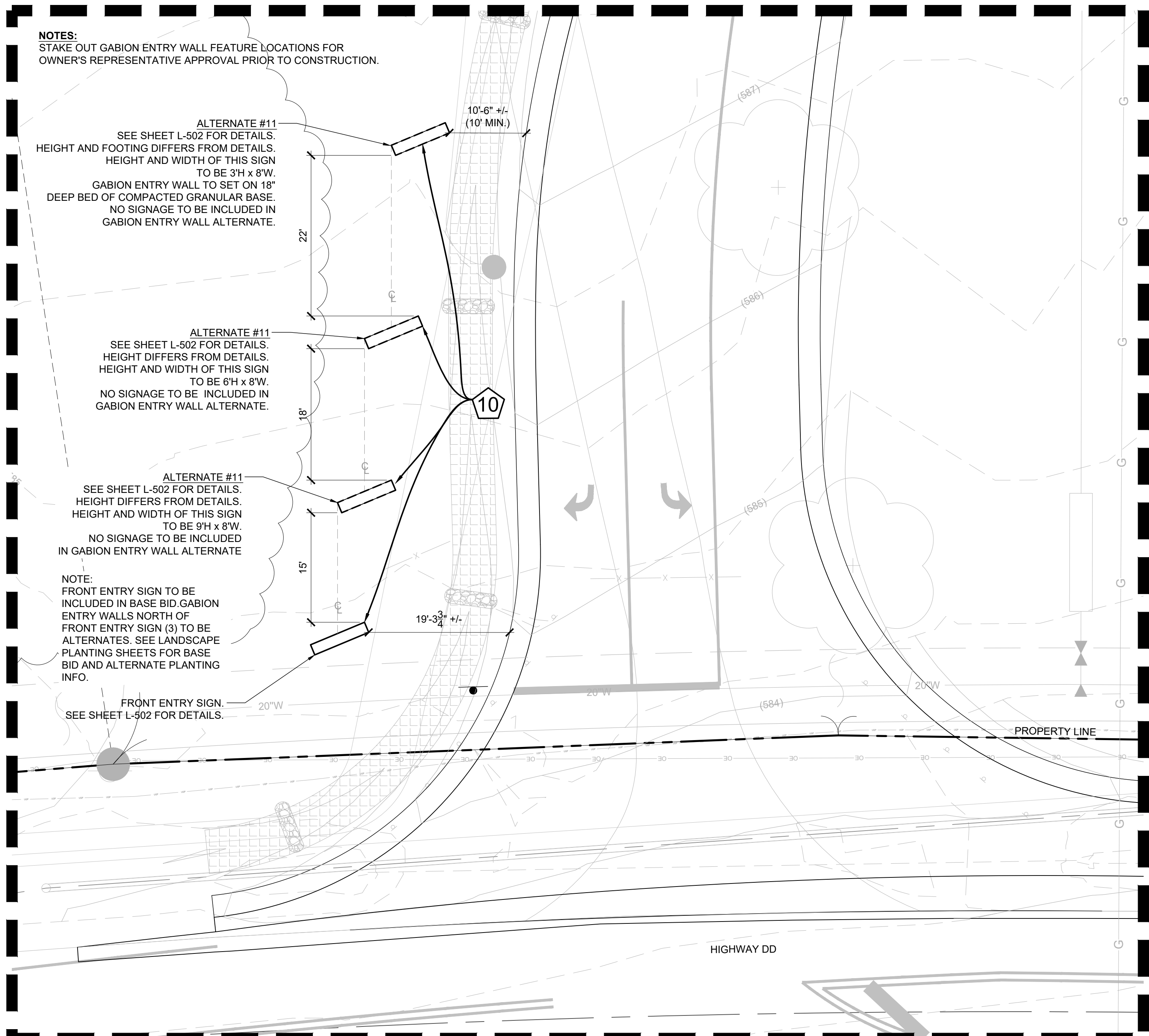
A ENTRY MONUMENT ENLARGEMENT PLAN SCALE: 1"=10'
